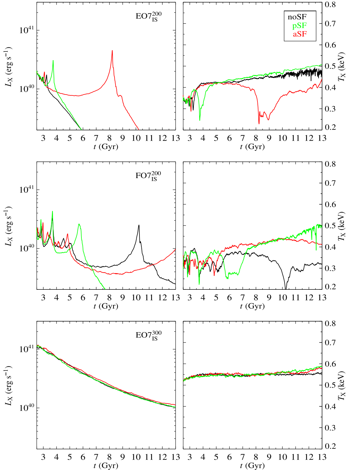
Figure 5. Time evolution of the X-ray luminosity L_X and X-ray emission weighted temperature T_X for the EO7_{IS}^{200} (top panels), FO7_{IS}^{200} (middle panels), EO7_{IS}^{300} (bottom panels) models. The black, green, and red lines refer to the noSF model, and to the passive and active SF schemes, respectively, with \eta_{SF} = 0.1 . The FO7_{IS}^{200} model has an evolution almost identical to that of EO7_{IS}^{300} shown here. See Section 3.1 for more details.
