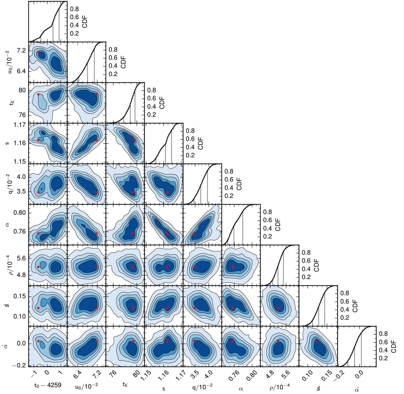
Fig. 11. Idem for ESBL+LOM's model.
