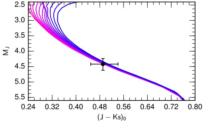
Fig. 5. Colour-magnitude diagram ( M_J , (J-K_s)_0 ) of the lens. The curves are a set of isochrones from 2 Gyr (in pink) to 8 Gyr (in blue) with solar metallicity (Bressan et al. 2012). The black cross indicates the range of colours and magnitudes explored by the MCMC at the 1\sigma level.
