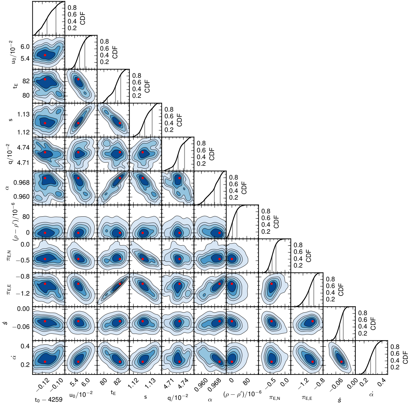
Fig. 12. Idem for ESBL+P+LOM's model ( u_0 > 0 ) with \rho' = 5.3 \times 10^{-4} .
