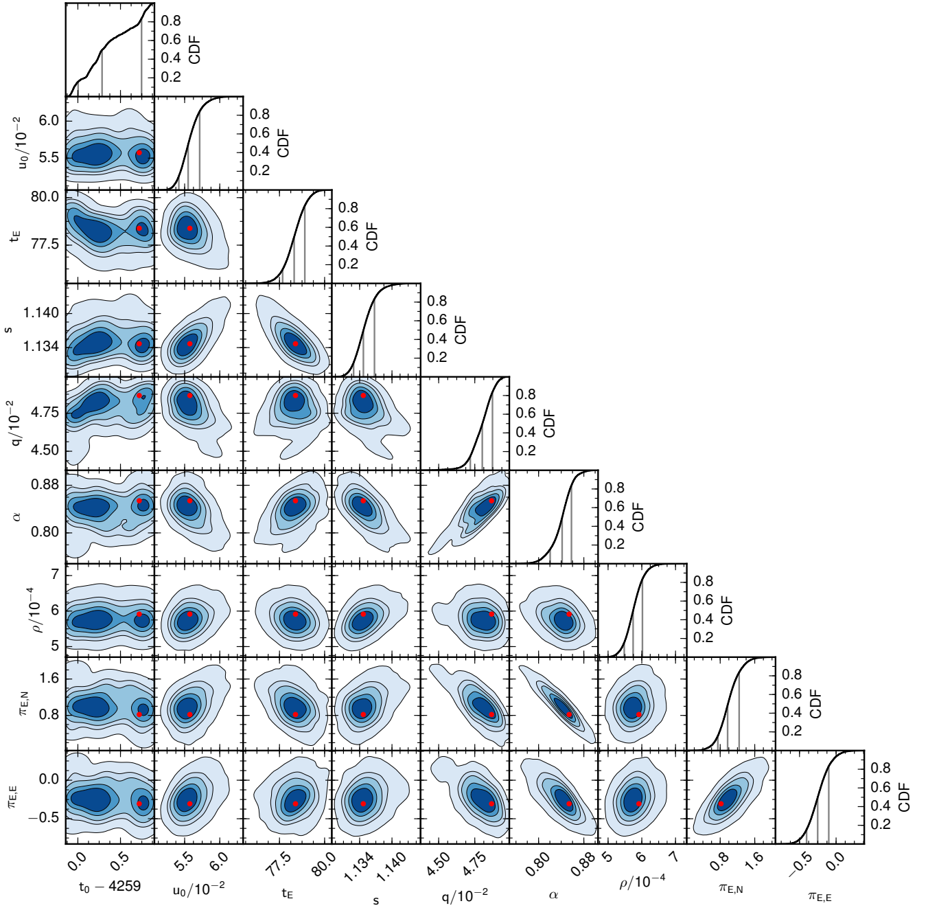
Fig. 10. Idem for ESBL+P's model.
