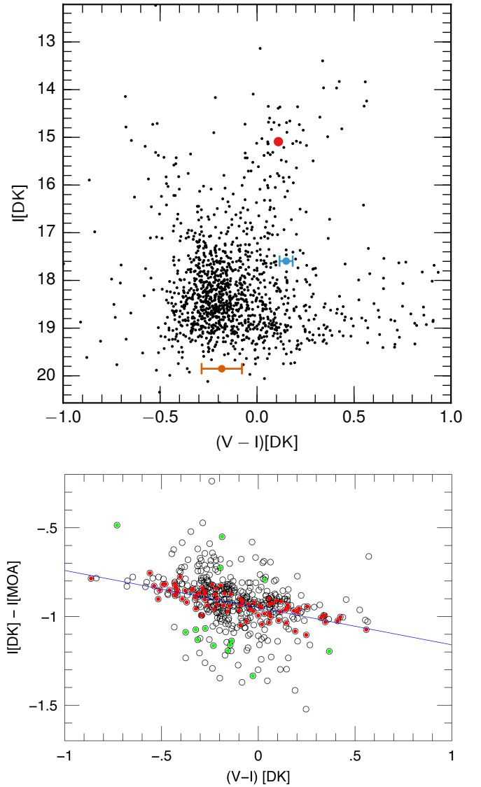
Fig. 4. Upper panel: ( I, V-I ) Danish instrumental CMD of the field around MOA-2007-BLG-197, not corrected for interstellar extinction. The red point marks the position of the RCG. The magnitude of the microlensing target is in blue (i.e. magnified source, lens and blended light). The orange point corresponds to the source alone. Lower panel: empirical linear relation between instrumental colours ( I_{\text{DK}} - I_{\text{MOA}} ) and (V-I)_{\text{DK}} (red and green points are astrometric matches that are uncrowded in the MOA image; after sigma-clipping, only red points are used for the fit).
