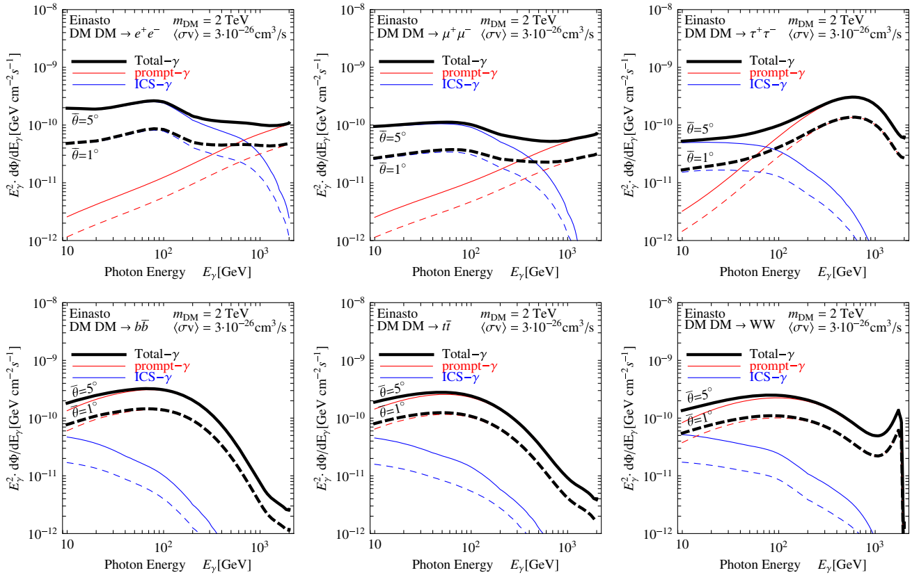
FIG. 1 (color online). Several example of \gamma -rays fluxes for 2 TeV DM candidates annihilating with thermal cross-section ( \langle \sigma v \rangle = 3 \times 10^{-26} \text{ cm}^3/\text{s} ) into leptonic channels (first row) and hadronic ones (second row). In all plots, the different hashing shows the predicted signal in two benchmark RoIs with apertures \bar{\theta}_1 (dotted line), and \bar{\theta}_5 (solid line). The red, blue and thick black lines denote instead the spectral features of the prompt, ICSs and total fluxes, respectively. See the text for further details.
