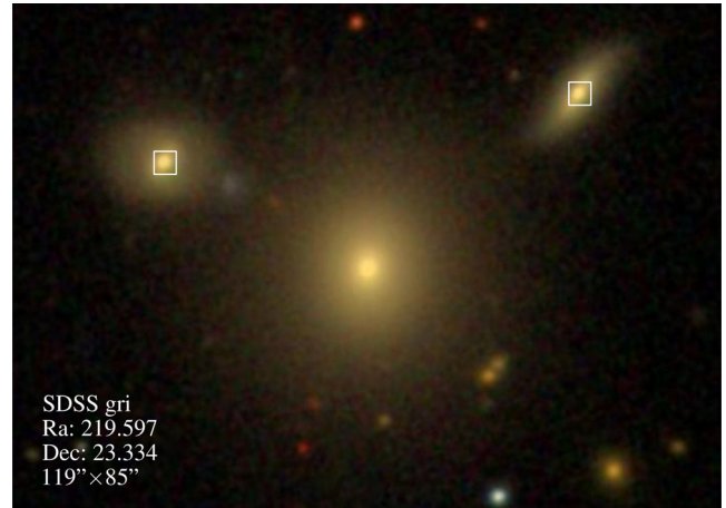
Figure 3. SDSS gri colour image of a BCG ( 119 \text{ arcsec} \times 85 \text{ arcsec} , corresponding to 72 \text{ kpc} \times 52 \text{ kpc} at z = 0.03 ). The spectroscopic target selection algorithm for the SDSS maximizes the number of non-fibre-collided targets. This selects against BCGs, whose central location would result in fibre collisions with many nearby satellites. As in the above example, more spectroscopic targets (white squares) can be obtained in a given area if satellites are targeted instead of the BCG. Cases where this bias impacted host galaxy isolation criteria were cleaned from our sample via visual inspection.
