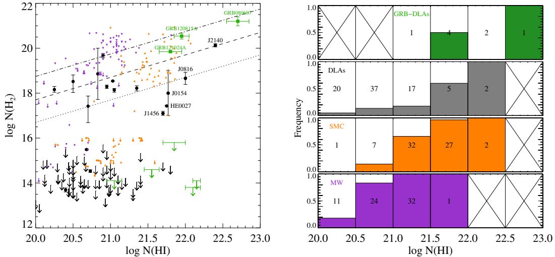
Fig. 1. Left: column density of H 2 as a function of that of H I. Data for high-redshift ( z > 1.8 ) quasar-DLAs (black points and arrows) are from Noterdaeme et al. (2008; updated to more recent determination in a few cases, Ivanchik et al. 2010; Rahmani et al. 2013; Alborno Vázquez et al. 2014). Additional measurements in ESDLAs are from Noterdaeme et al. (2015) and Guimarães et al. (2012). Data for GRB-DLAs (green) are from Ledoux et al. (2009, upper limits), Prochaska et al. (2009, GRB 080607), Krühler et al. (2013, GRB 120815A), and Friis et al. (2015, GRB 121024A). With the exception of GRB 080607 and GRB 121024A, in which damped H 2 lines allow for accurate column density measurement at medium spectral resolution, all high- z values (quasar and GRB DLAs) are from UVES data. Purple (resp. orange) points represent measurements in the Milky Way (resp. SMC). The dotted, dashed, and dash-dotted lines represent average molecular fractions of, respectively, f = 0.1 , 1, and 10%. Right: frequency of H 2 detection as a function of the H I column density. For each N(\text{H I}) bin, systems with \log N(\text{H}_2) \geq 17 are coded in colour, and systems with \log N(\text{H}_2) < 17 are shown in white. Systems with upper limits that are not stringent (i.e. above \log N(\text{H}_2) = 17 ) are not taken into account. The numbers in each box indicate the total number of systems contributing to the bin. Crossed boxes have no statistics.
