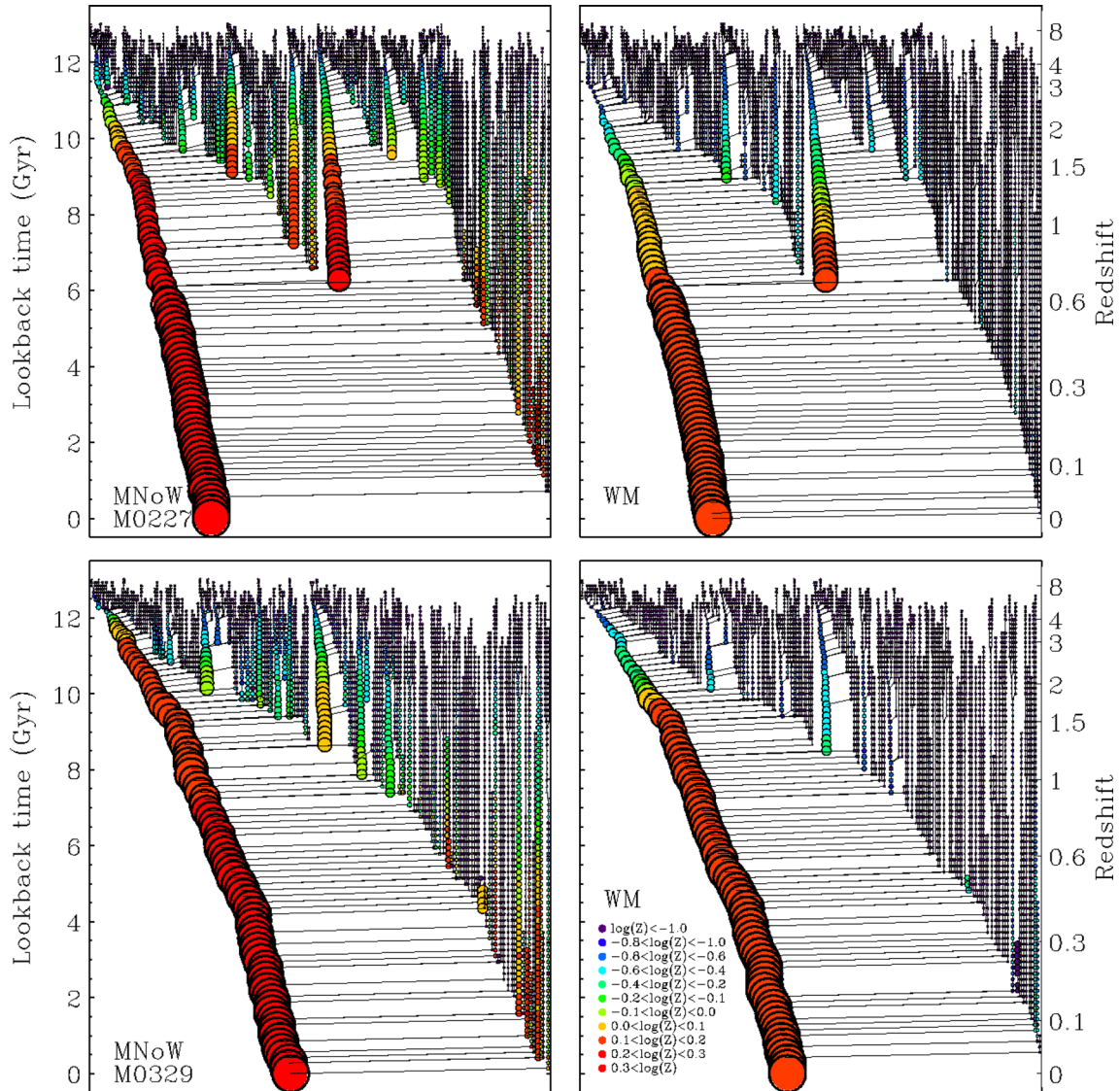
Figure 1. Halo-based merger trees for the two example galaxies M0227 (top panels) and M0329 (bottom panels) for the model without winds (MNOW, left-hand column) and with winds (WM, right-hand column). The size of the circles is scaled to the mass of the central galaxy in the respective haloes, the colour is coded by the metallicity of the stellar component from blue (low metallicity) to red (high metallicity). In the no wind models (MNOW, left-hand panels), the satellite haloes host more massive galaxies with more metal-rich stellar components, in particular at low redshifts. M0227 has a major merger with galaxy of comparable metallicity at z \sim 0.7 , whereas M0329 grows by minor mergers alone. The infalling systems are particularly metal-poor in the wind simulations (WM, bottom-right panel). Not all galaxies of the haloes indicated here merge with the central galaxy by z = 0 (see Fig. 2).
