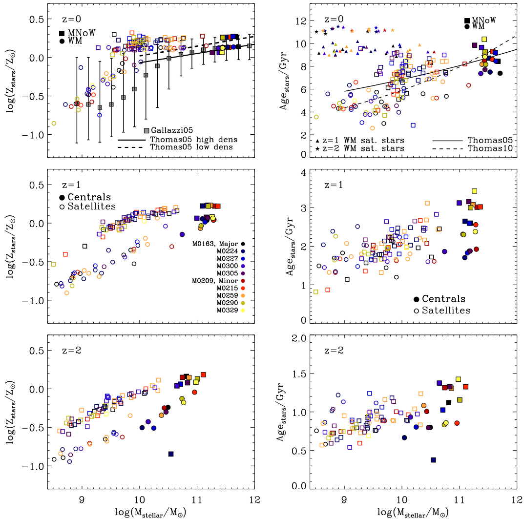
Figure 3. Left-hand column: mean stellar metallicity as a function of galaxy stellar mass at z = 0, 1 and 2 (from top to bottom) for 10 massive galaxies (different colours) simulated with the MNoW model (filled squares) and the WM model (filled circles). The satellite galaxies residing in the respective galaxy haloes (same colours) are indicated by open symbols. At all redshifts, the satellite galaxies in the wind model (WM) have significantly lower metallicities than those simulated without winds (MNoW). For this model, the z = 0 metallicities agree with observational estimates (Thomas et al. 2005, black lines; Gallazzi et al. 2005, grey squares). Right-hand column: mean stellar age as a function of galaxy mass at z = 0, 1 and 2 (from top to bottom) for the 10 galaxies and their satellites as in the left-hand column. Compared to observations (Thomas et al. 2005, 2010), the central galaxies in the WM model are slightly too young by roughly 2 Gyr. For the WM model, the small filled triangles and stars indicate the hypothetic present-day ages of the satellites at z = 1 and 2 , most of them have merged with the central galaxies until z = 0 .
