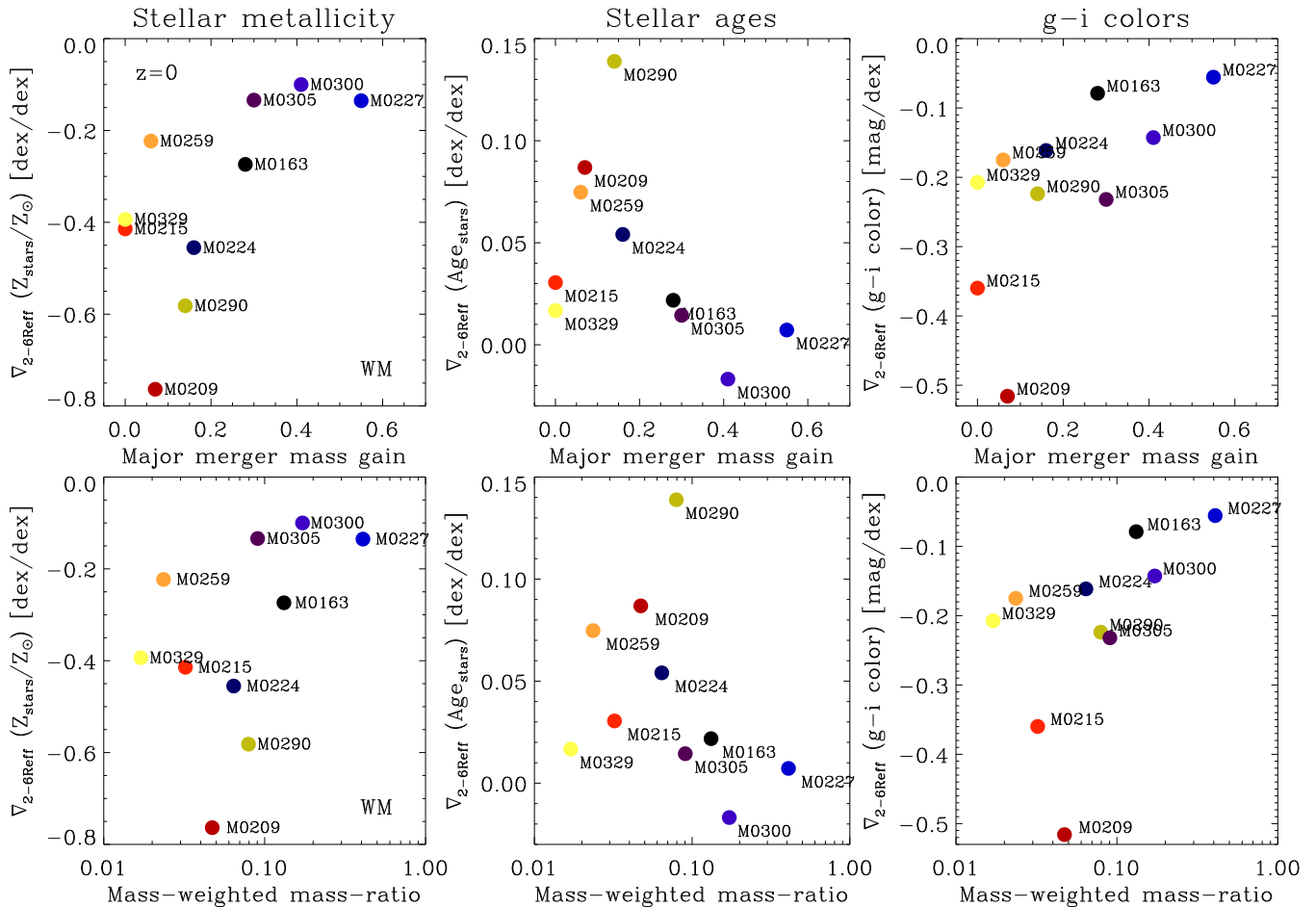
Figure 10. Left-hand panels: stellar metallicity gradients (between 2 and 6 R_{\text{eff}} ) versus the mass gain through major mergers (top panel) and versus the mass-weighted merger mass-ratio (bottom panels) for the 10 re-simulated galaxies in the WM simulations at z = 0 . The points are colour-coded according to their past major mergers as in Fig. 4. The higher the major merger mass gain or the mass-weighted mass-ratio, the smaller is the slope of the metallicity gradient. Middle panels: the same as in the left-hand panels, but for stellar age at z = 0 . The higher the major merger mass gain, the flatter are the age gradients. Right-hand panels: the same as in the left-hand panels but for g - i colours at z = 0 . The higher the major merger mass gain or the mass-weighted mass-ratio, the smaller is the slope of the colour gradient. This trend is entirely driven by the negative metallicity gradients.
