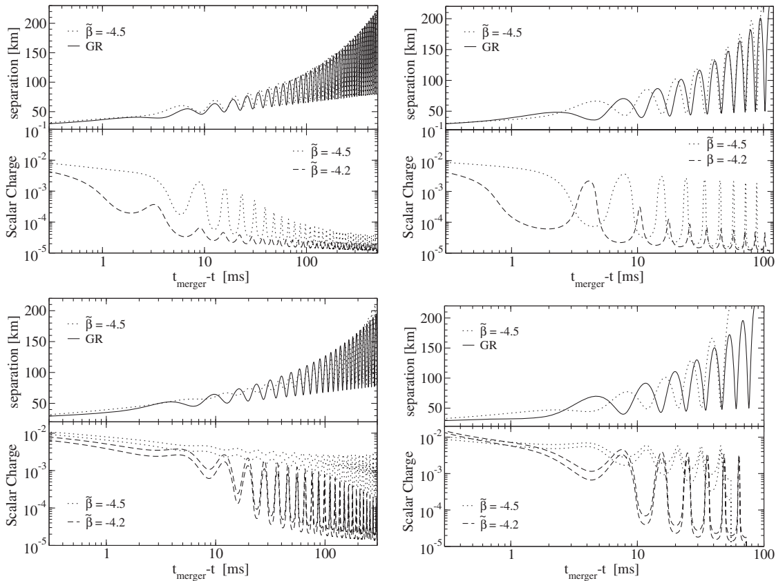
FIG. 9. Eccentric binaries: evolution of the separation for a binary governed by GR and ST with \tilde{\beta} = -4.5 and scalar charges of the binary’s components (for binaries governed by ST with \tilde{\beta} = -4.5 and \tilde{\beta} = -4.2 for comparison purposes) as a function of time to merger, for an equal-mass binary (top panels) and an unequal-mass binary (bottom panels), for low-eccentricity orbits (left column) and high-eccentricity orbits (right column) (see text for the details on the exact masses and eccentricities). As the orbit progresses, and scalar charges become significant, the eccentricity is reduced more rapidly in the ST cases as illustrated by the increasingly reduced differences between local maxima and minima of the binary’s separation.
