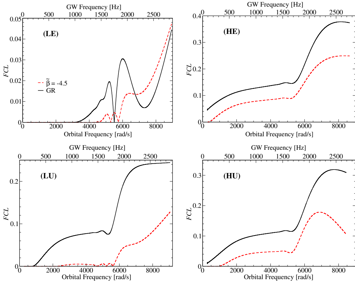
FIG. 8 (color online). Fractional change of the luminosity, FCL \equiv |\mathcal{L}_{ST} - \mathcal{L}_{GR}|/\mathcal{L}_{GR} , for the LE (top-left panel), HE (top-right panel), LU (bottom-left panel), and HU (bottom-right panel) binaries as a function of orbital and GW frequencies (assuming b = 0.1 for concreteness and for clarity's sake). The solid black line shows the FCL of a ST with \tilde{\beta} = -4.5 with respect to GR, while the dashed red line represents the FCL of a ST with \tilde{\beta} = -4.2 (again with respect to GR).
