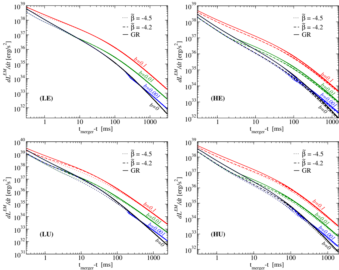
FIG. 6 (color online). Time derivative of the luminosity as a function of time to merger, for the same parameters shown in Fig. 4. Note that the differences are less significant for the low-mass binaries.
