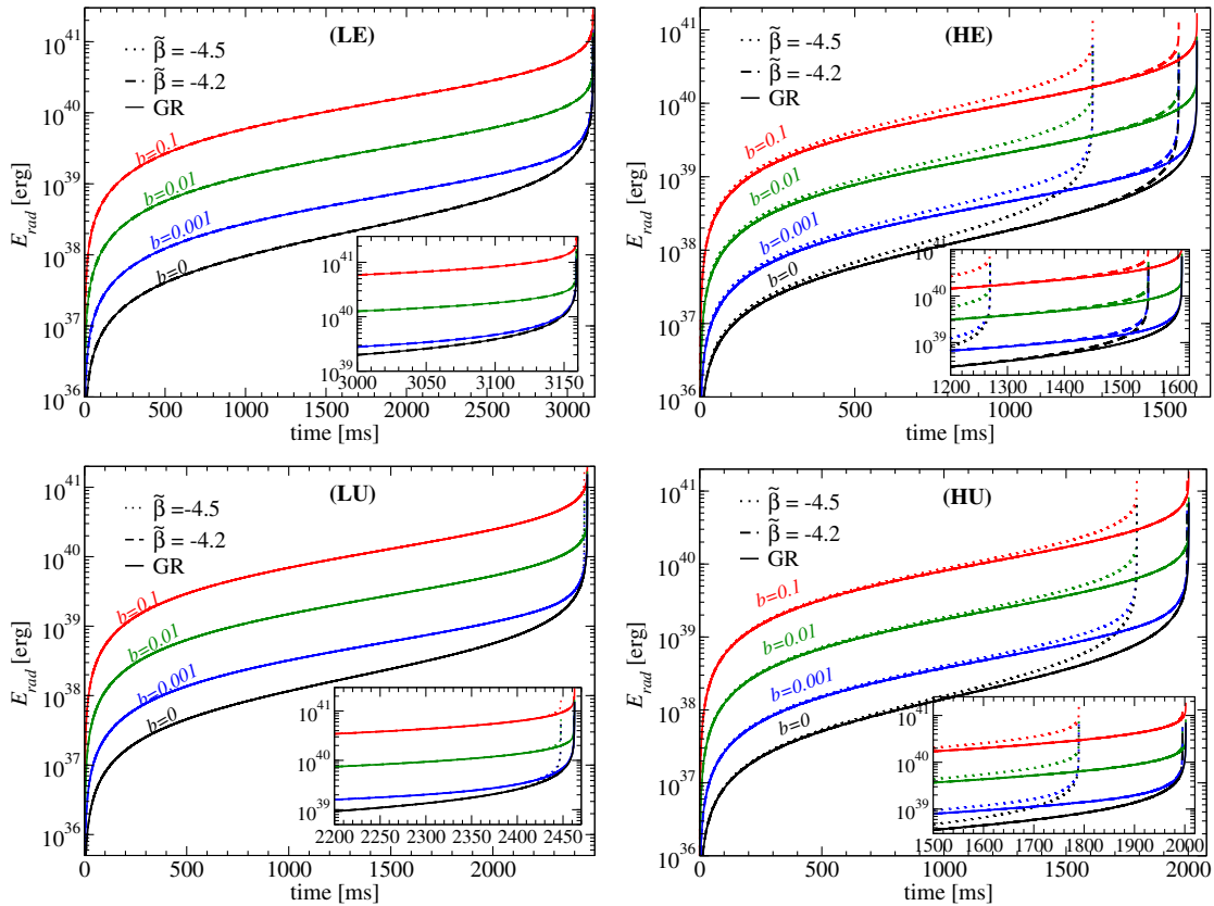
FIG. 7 (color online). Total energy radiated in electromagnetic waves (i.e. the time integral of the luminosity) as a function of time elapsed from an initial separation of approximately 180 km for the same parameters shown in Fig. 4. Insets show zoom-ins of the total energy radiated at late times, when the binary is close to the merger.
