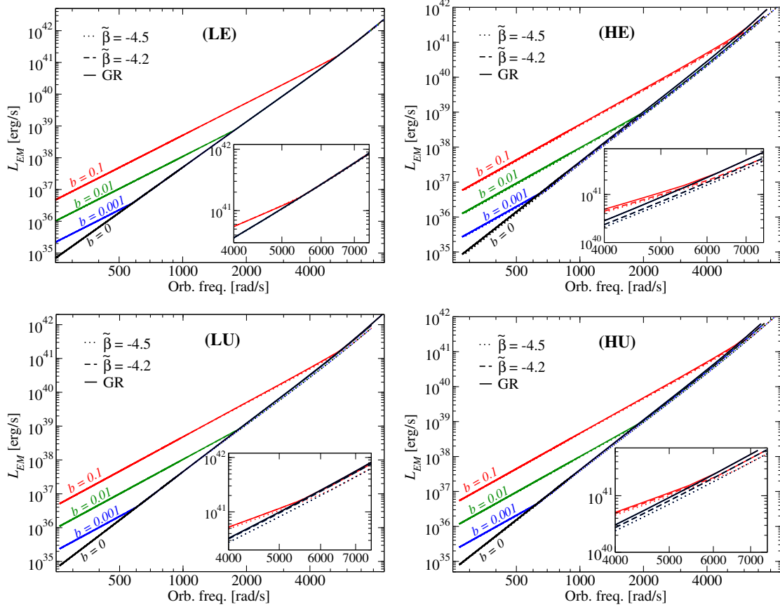
FIG. 5 (color online). Luminosity as a function of orbital frequency, for the same parameters shown in Fig. 4.
