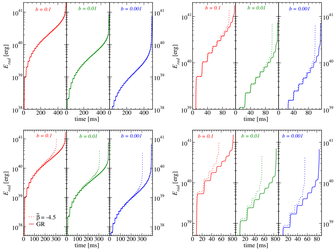
FIG. 11 (color online). Energy radiated by eccentric binaries, as a function of the time elapsed from an initial binary separation of approximately 220 km, for the same parameters shown in Fig. 9. We show, in contiguous panels, three different magnetic ratios (from left to right within each plot): b = 0.1 (in red), 0.01 (in green), and 0.001 (in blue). Note that in the case of low-eccentricity orbits (left column), the radiated energy has a smoother (continuous) trend, while in the case of high-eccentricity orbits (right column) the radiated energy is more jagged; this is a consequence of the oscillatory features in the luminosity, and ultimately the effect of the different dynamics of each binary.
