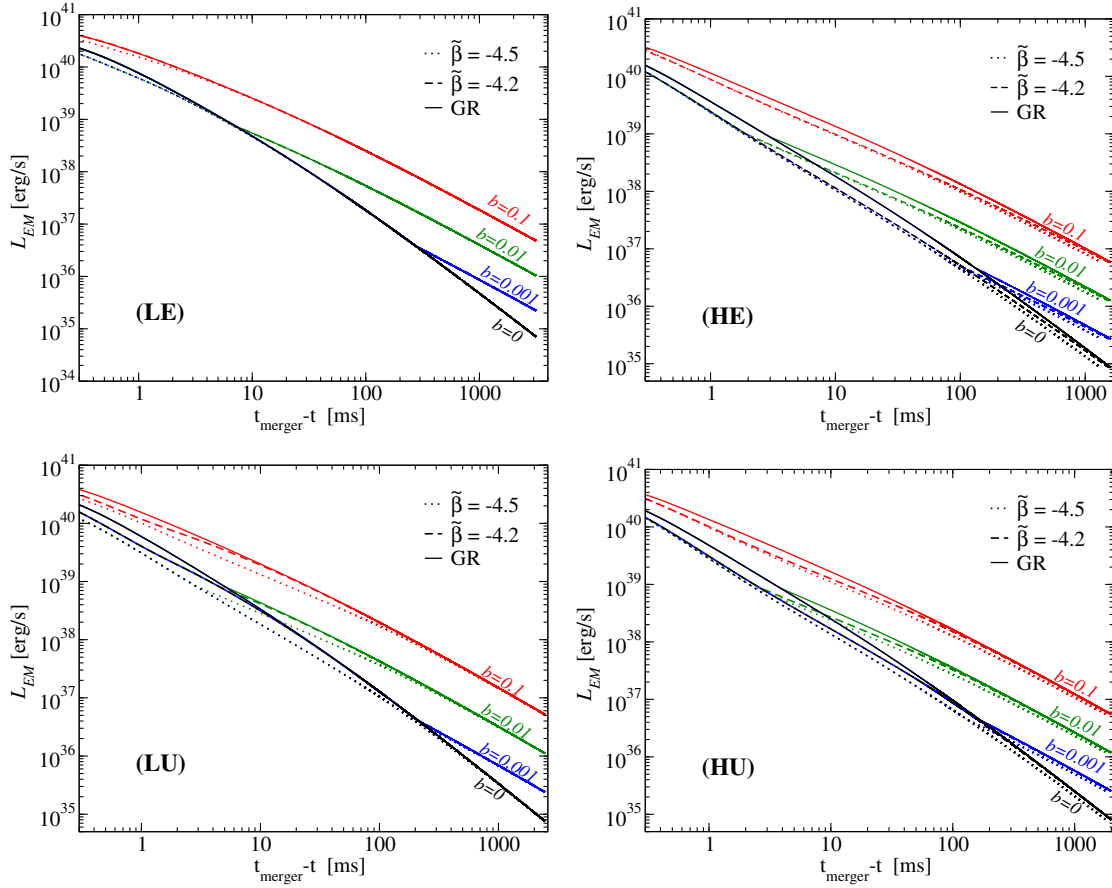
FIG. 4 (color online). Luminosity vs time to merger, for the same parameters shown in Fig. 1. Different lines in each panel indicate the ratio between the secondary and primary magnetic fields (from top to bottom): b = 0.1 (in red), b = 0.01 (in green), b = 0.001 (in blue), and a nonmagnetized secondary (i.e. b = 0 , in black).
