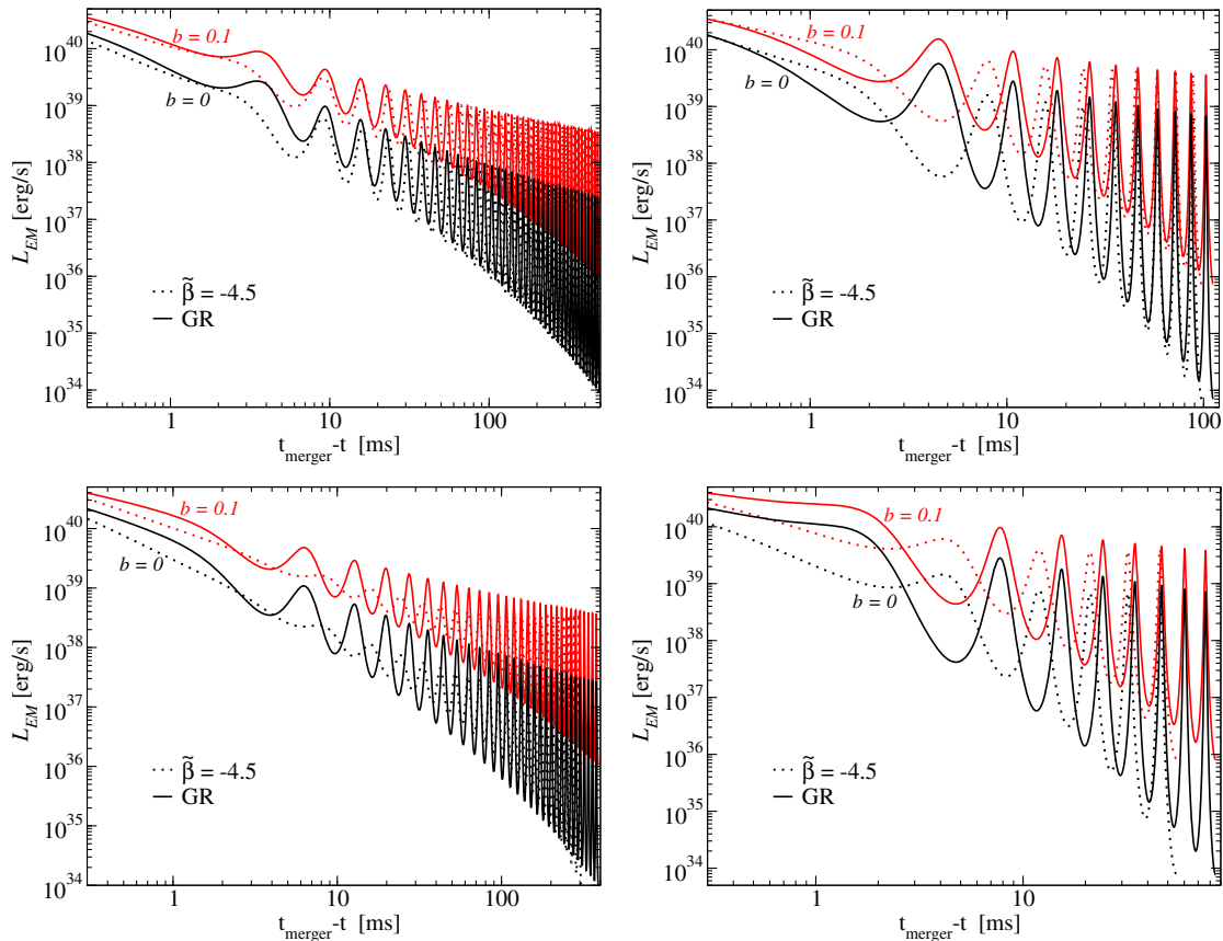
FIG. 10 (color online). Luminosity vs time to merger, for the same parameters shown in Fig. 9. For clarity’s sake we show here the two extremal magnetic ratios considered, b = 0.1 and b = 0 (i.e. a nonmagnetized companion).
