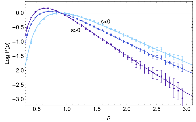
Figure 4. Density PDF in negative slope (solid light blue), positive slope (dashed purple) and all regions (dashed blue) for cells of radii R_1 = 10 \text{ Mpc } h^{-1} and R_2 = 11 \text{ Mpc } h^{-1} at redshift z = 0.97 . Predictions are successfully compared to measurements in simulations (points with error bars).
