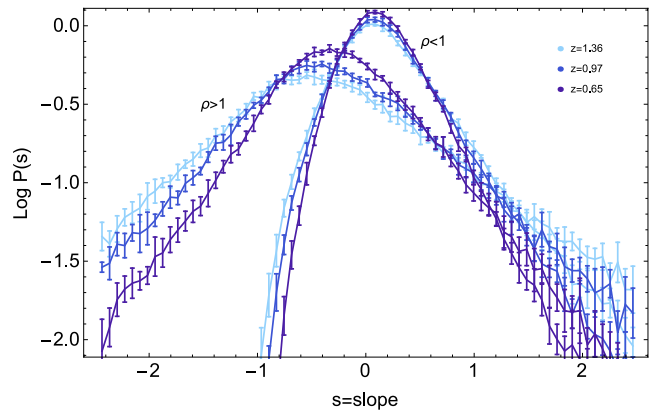
Figure 5. Same as Fig. 3 for a range of redshifts as labelled. Only the underdense ( \rho < 1 ) and the overdense ( \rho > 1 ) PDFs are shown.
