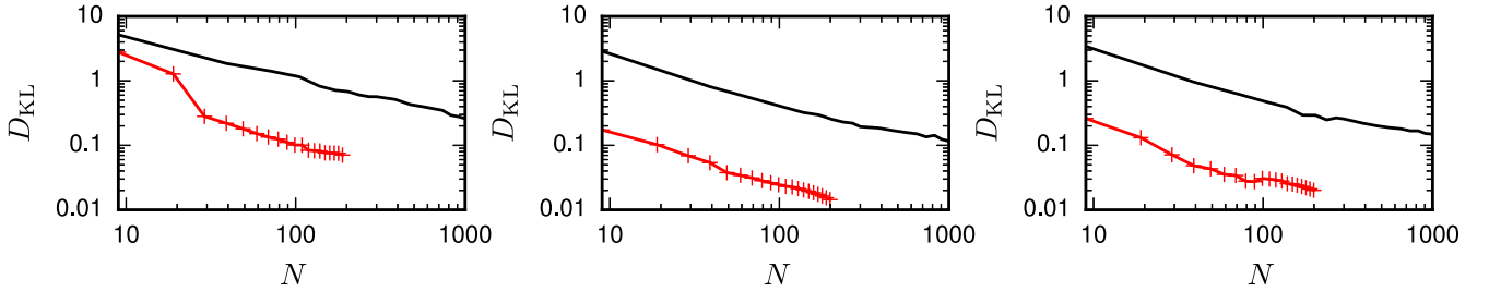
Figure 11. Kullback–Leibler divergences as a function of the number of parameters required. Smaller divergences indicate a greater degree of similarity between the two distributions and so a more successful approximation. In black we plot D_{\text{KL}} for thinned MCMC chains relative to the long unthinned chain, using kernel density estimates of both and in red we plot values the D_{\text{KL}} between the Gaussian mixture approximation and the kernel density estimate of the unthinned chain, with crosses indicating different values of K running from K = 1 to 20. In the left-hand plot we show values for star A, in the middle star B and star C on the right.
