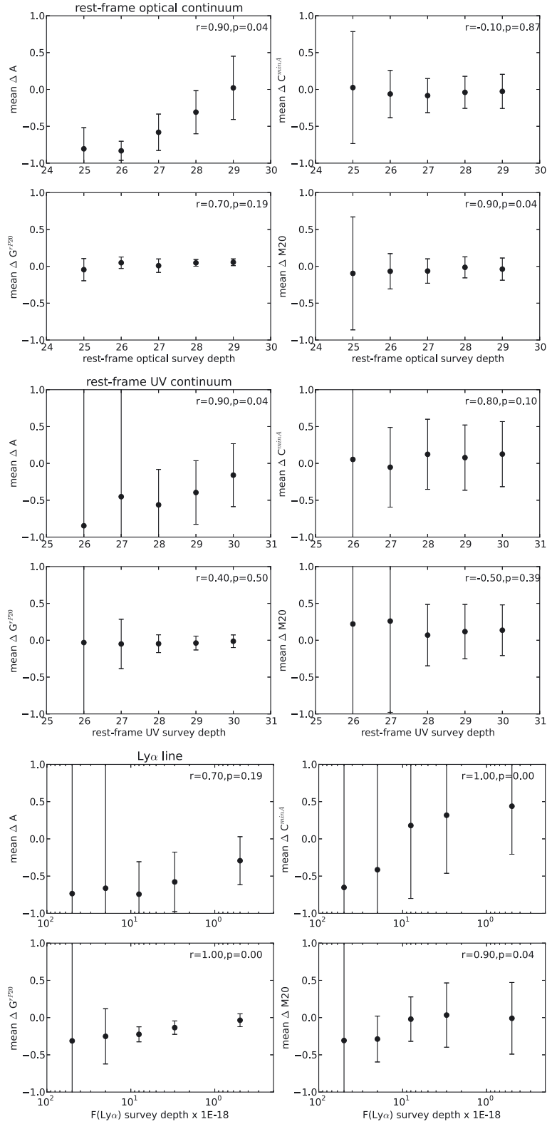
Fig. A.4. Mean \Delta(\text{param}) as defined in Eq. (A.1) vs. simulated survey depth. param is A (upper left), C^{\text{min}A} (upper right), G^{rP20} (lower left), and M20 (lower right) for the rest-frame optical, UV, and \text{Ly}\alpha simulated images. The deepest simulated survey is represented by the most right data point in each panel. The error bars represent the standard deviation among all the high- z simulated LARS galaxies. In the case fewer-than-twelve galaxies are detected at a specific depth, the error bars are increased proportionally to the number of undetected galaxies. The numbers on the top right corner of each panel represent the Spearman test coefficient, r , and probability, p , of uncorrelated datasets, assuming that the depth vector indicates the deepest survey on the right of the x -axis.
