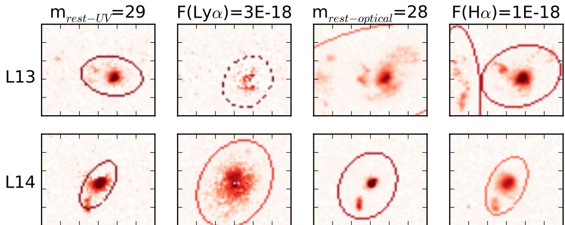
Fig. B.6. As Fig. B.3, but for a shallow simulated survey. Only the bright right clump of z2L13 is detected in UV at a 10\sigma detection limit of m_{\text{rest-UV}} = 29 . Its Ly \alpha emission is localized around the lower side of the right clump. In H \alpha the two overlapping sources become well separated.
