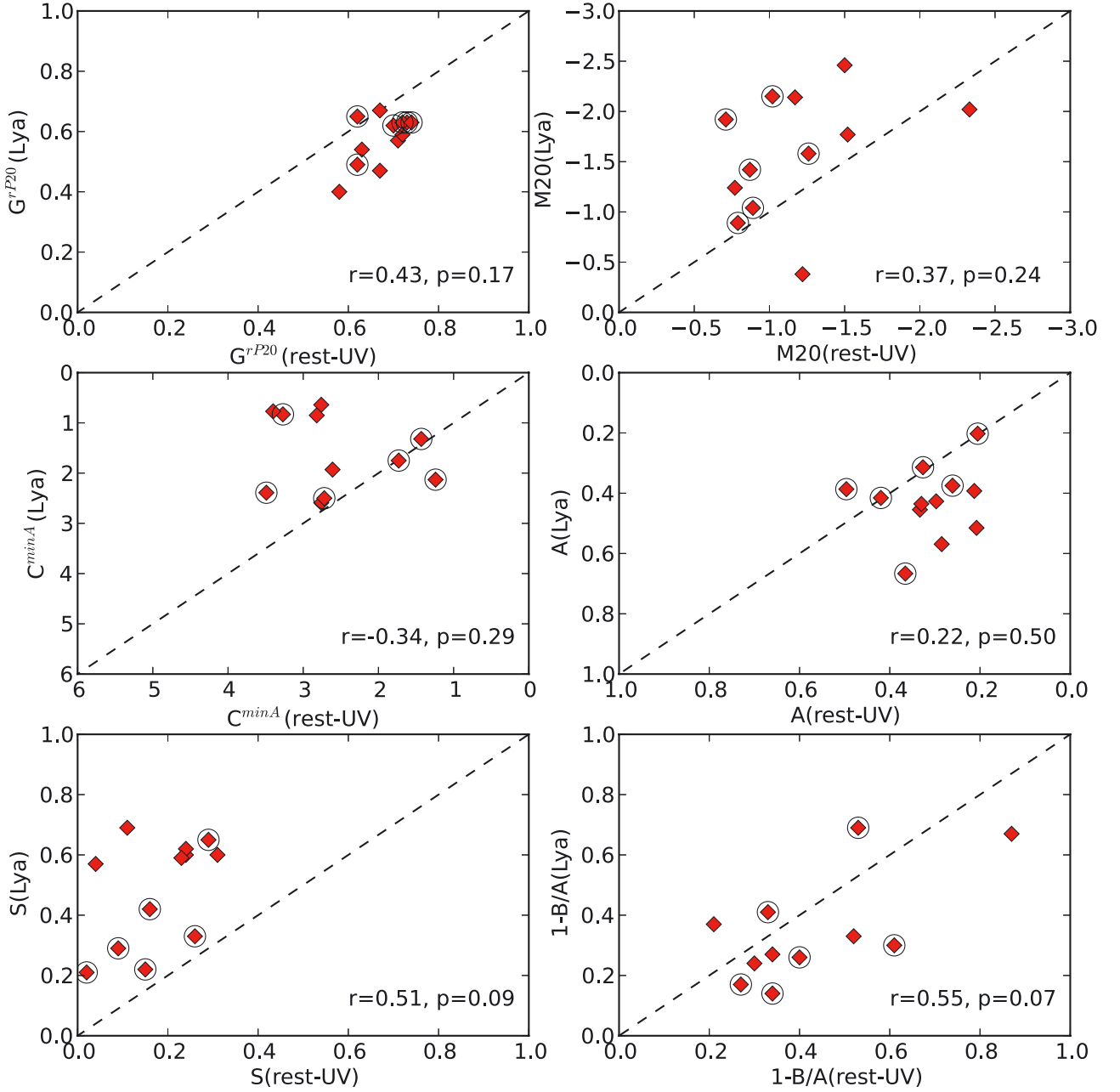
Fig. 5. Non-parametric measurements performed in the Ly \alpha images versus the ones performed in the rest-frame UV. From the upper left to the lower right : G^{rP20} , M20 , C^{\min A} , A , S , and SExtractor ellipticity ( 1 - B/A , where A and B are the semi-major and semi-minor axes of the detection ellipse). The dashed line indicates the 1:1 relation. The numbers reported in each panel correspond to the Spearman test coefficient, r , and probability, p , of uncorrelated datasets. r = 0 indicates no correlation, r = 1(-1) indicates direct(indirect) proportionality.
