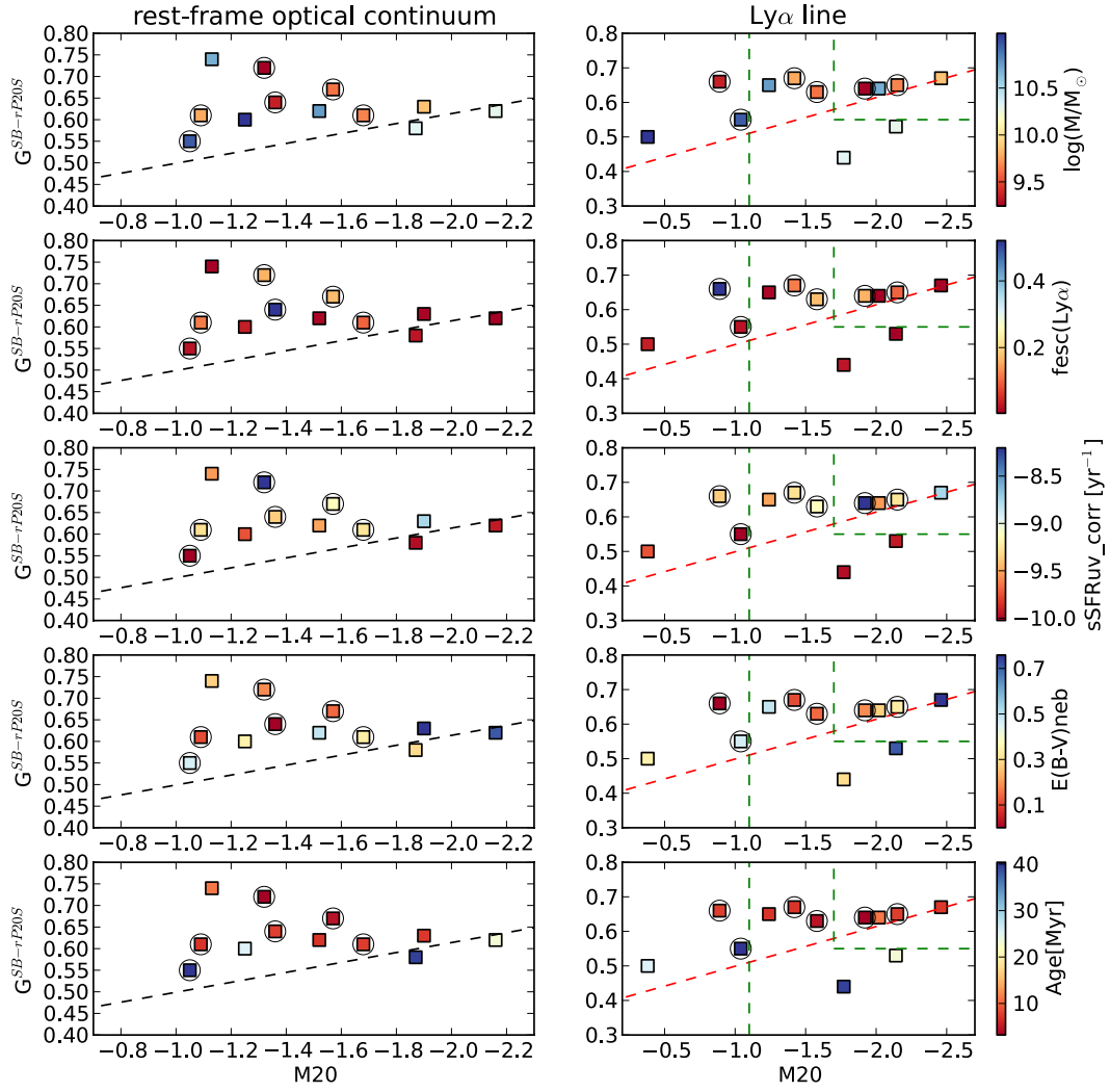
Fig. 18. G^{SB-rP20S} vs. M20 measured in the rest-frame optical (left panels) and \text{Ly}\alpha (right panel) of the original LARS galaxies (squares). LARS-LAEs are indicated with open circles. In each row the colour scale corresponds to an integrated physical property derived in Paper II (vertical colour bar). From the top row the integrated physical properties are stellar mass, \text{Ly}\alpha escape fraction, dust-corrected specific star formation rate, nebular reddening, and age. The dashed lines indicate the regions of separation between merging system, normal galaxies, and bulge-dominated systems as presented in Figs. 13 and 14.
