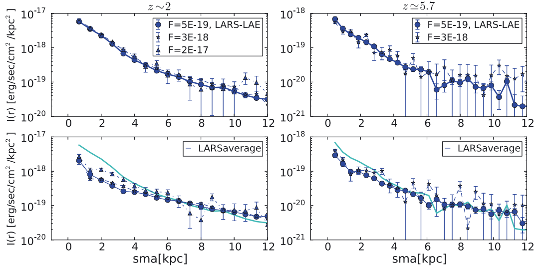
Fig. 15. \text{Ly}\alpha surface brightness profiles of the two stacks: LARS-LAE (upper) and LARSaverage (lower; see text for details). Left and right panels show the profiles at z \sim 2 and 5.7 , respectively, corresponding to three and two 10\sigma detection limits (blue circles, stars, and triangles). The cyan solid line represents the LARS-LAE profile of the deepest simulated survey and it is shown in the lower panels for comparison. The difference in the surface brightnesses in the left and right panels is the result of surface brightness dimming. The error bars correspond to the shallowest survey in each panel; for the other depths they are usually smaller than the symbols. The large error bars at \text{sma} > 5 kpc are produced by background noise.
