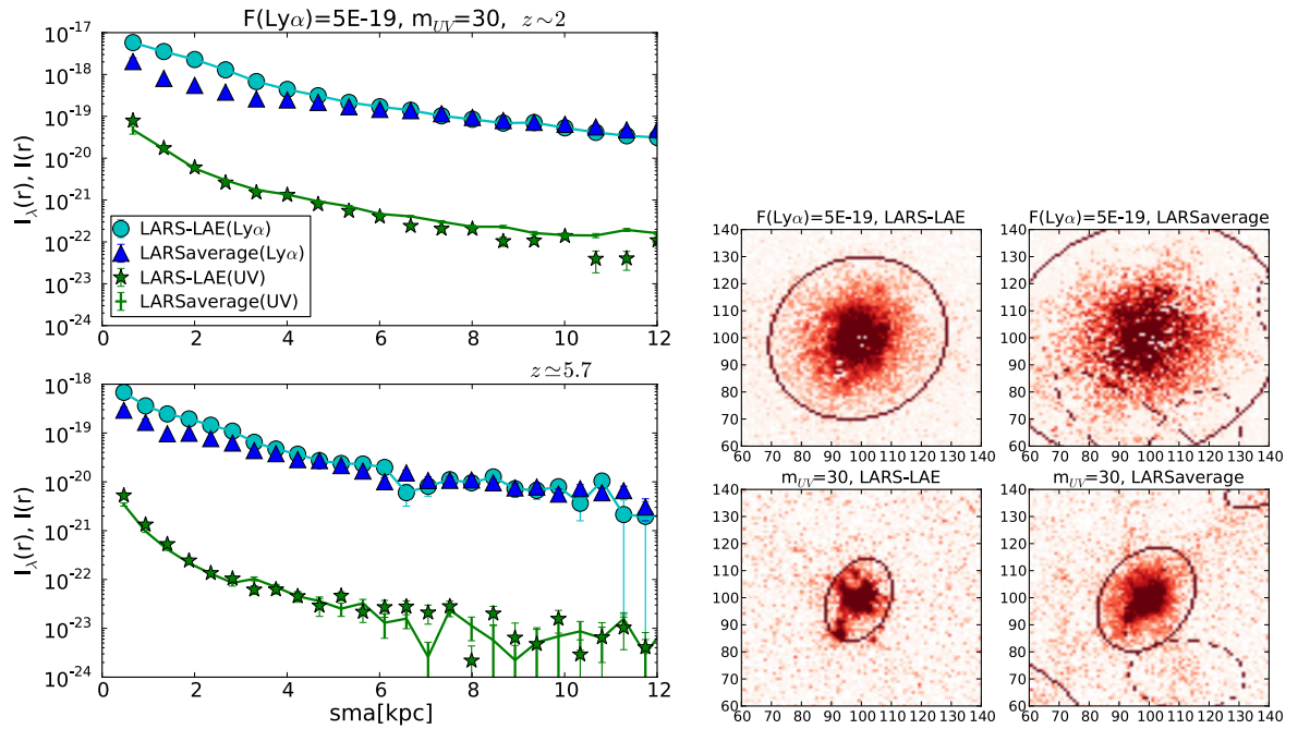
Fig. 16. Left: surface brightness profiles for \text{Ly}\alpha (units of \text{erg s}^{-1} \text{cm}^{-2} \text{kpc}^{-2} ) at z \sim 2 (upper panel). LARS-LAEs are shown with the cyan circles and line, and LARSaverage with (blue triangles). Rest UV profiles (units of \text{erg s}^{-1} \text{cm}^{-2} \text{kpc}^{-2} \text{\AA}^{-1} ) are shown for the LARS-LAE sample (green stars) and LARSaverage (green line with errorbars). The lower panel shows the equivalent profiles at z = 5.7 . Right: from the upper left to the lower right: \text{Ly}\alpha for the LARS-LAE and LARSaverage stacks; rest-frame UV continuum for LARS-LAEs and LARSaverage. The logarithmic colour scale is adjusted to match the background level. The elongated structures in the LARSaverage continuum frame come from L09 (vertical) and L11 (diagonal). The whitish structures in the LARSaverage \text{Ly}\alpha come from the same galaxies, which are weak \text{Ly}\alpha emitters but show strong absorption centrally. The cut-out size is about 15 kpc.
