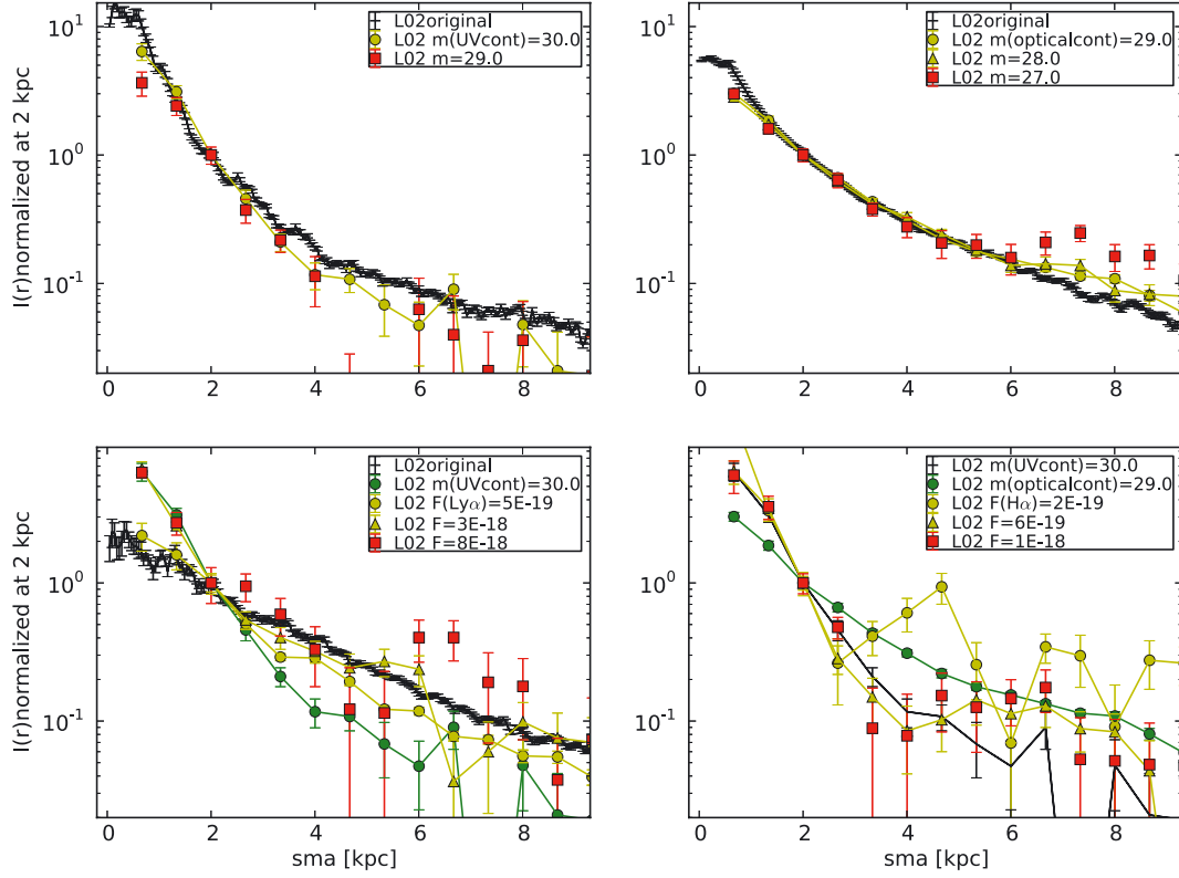
Fig. C.1. Normalized surface brightness profiles of L02. Black points with error bars correspond to the surface brightness profile of the original LARS images in the rest-frame UV, optical, and \text{Ly}\alpha as explained in the text (Fig. 8). The red squares represent the profile affected by background noise, for a certain shallow survey.
