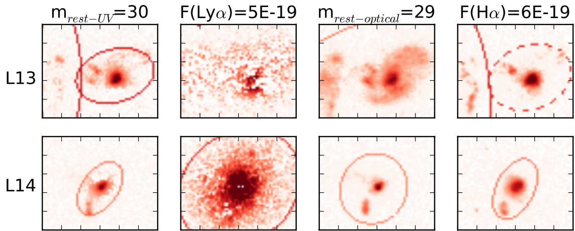
Fig. B.3. As Fig. B.1 for z2L13 and z2L14. For z2L13 SEx aperture in \text{Ly}\alpha happens to be outside the shown region. Also, two main sources connected by undetectable ( m_{\text{rest-UV}} > 30 and F(\text{H}\alpha) < 6\text{E-}19 \text{ erg s}^{-1} \text{ cm}^{-2} ) surface brightness structures are seen in UV continuum and \text{H}\alpha . By using the chosen detection parameters, SEx found two sources as separated. As in \text{Ly}\alpha and optical continuum the photometric measurements are done centring the aperture close to the right clump, we locate the aperture on that one for the photometry in UV and \text{H}\alpha as well.
