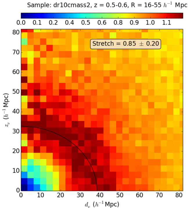
Figure 1. Example of a void stack in two dimensions and its stretch measurement. This stack includes voids from size 16 to 55 h^{-1} \text{ Mpc} . For clarity void galaxies are binned on to a uniform grid with cell size \sim 3 h^{-1} \text{ Mpc} , though the bins are not used in the stretch calculation. The black line shows an ellipse with the same stretch as the stacked void, and the caption shows the measured stretch and uncertainty. The uncertainty is the 1\sigma deviation taken from 1000 bootstrapped samples. The colour bar shows the density in each grid cell in units of the mean density of this sample.
