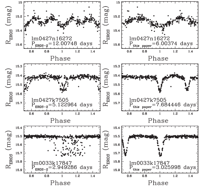
Figure 4. Light curves of EBs before (left panel) and after (right panel) correction of the period (see text for details).
