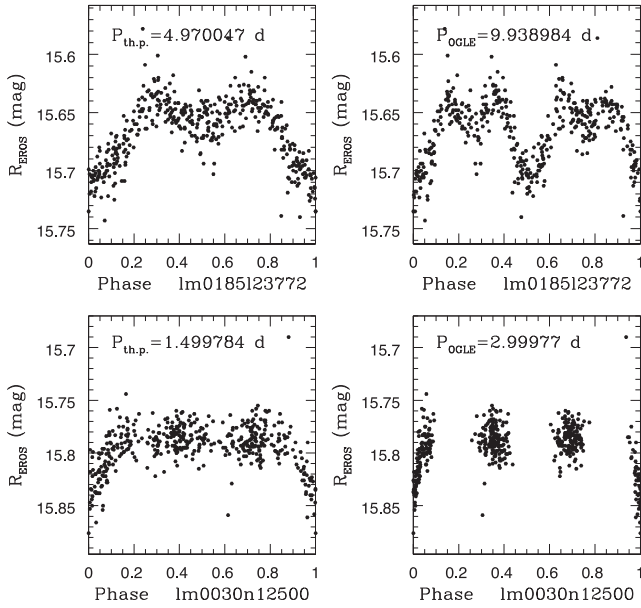
Figure 8. Light curves of Im0185123772 and Im0030n12500 with the periods used in this paper (left panel) and provided by the OGLE III catalogue (right panel).
