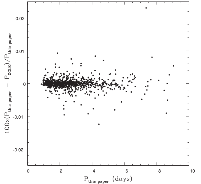
Figure 7. Comparison between periods adopted in this paper and those in the OGLE III and OGLE IV catalogues for the 1072 EBs in common. Two objects, namely Im0185123772 and Im0030n12500, were not included because their OGLE periods differ significantly from our values (see text and Fig. 8 for details).
