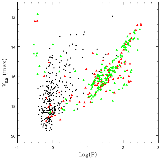
Figure 16. PL distribution at K_{s,0} maximum of the 563 contact binaries shown in Fig. 14. Black dots are objects with (V - I_0) < 0.3 mag, and red triangles are objects with (V - I_0) \geq 0.3 mag of which those with 13 or more epochs in the K_s band are marked in green.
