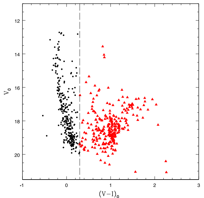
Figure 14. Colour-magnitude diagram of 563 contact binary stars which have V and I (OGLE III) and K_s (VMC) magnitudes. Black dots are objects with (V - I)_0 < 0.3 mag and red triangles are objects with (V - I)_0 \geq 0.3 mag. The dashed line corresponds to (V - I)_0 = 0.3 mag.
