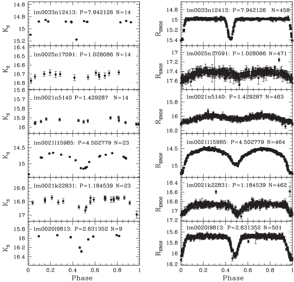
Figure 11. Light curves in the K_s (left panels) and R_{EROS} (right panels) passbands of example HEBs with a counterpart in the VMC catalogue. P – period (d), N – number of observations in the corresponding passband.
