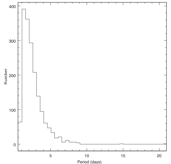
Figure 5. Period distribution of our sample of LMC EBs.
