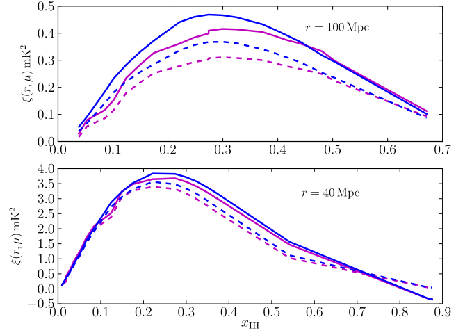
Figure 10. The two-point correlation function as a function of neutral fraction x_{\text{HI}} for a given correlation length r for the numerical simulation. Solid and dashed lines correspond to calculations with and without the redshift space distortion effect, respectively. The magenta and blue lines show results for \mu_r = 1 and \mu_r = 0 , respectively. Here, we have used the method described in Section 6 to perform the two-point correlation analysis on effectively 504 LC volumes thus suppressing the sample variance seen in Fig. 9.
