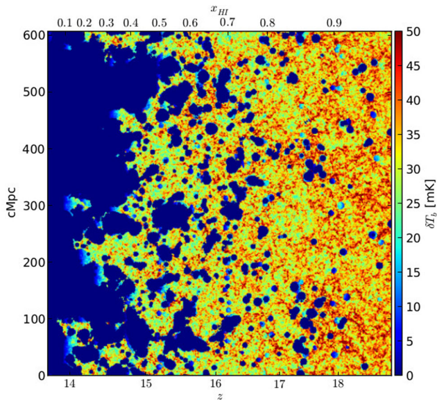
Figure 2. A slice through the 21-cm brightness temperature LC volume from the seminumerical simulation.
