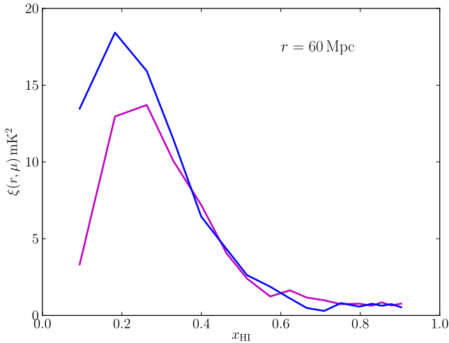
Figure 11. The two-point correlation function as a function of neutral fraction x_{\text{HI}} for the seminumerical simulation without the redshift space distortion effect. The magenta and blue lines show results for \mu_r = 1 and \mu_r = 0 , respectively.
