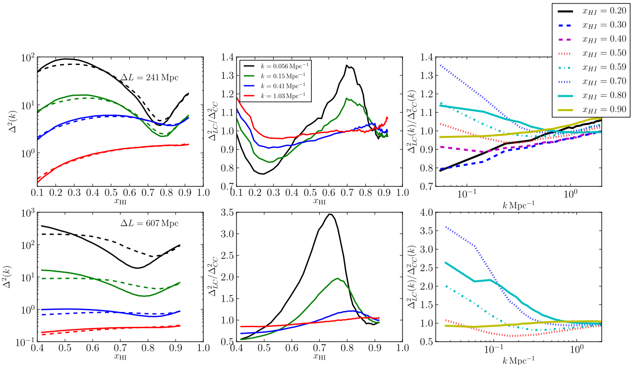
Figure 5. Same as Fig. 3, but we include redshift space distortions while estimating power spectra with and without the LC effect.
