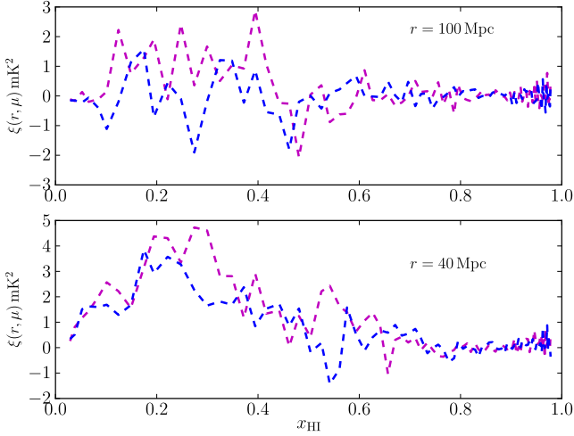
Figure 9. The two-point correlation function as a function of neutral fraction x_{\text{HI}} for a given correlation length r for the numerical simulation. We use the LC volume for this calculation. The magenta and blue lines show results for \mu_r = 1 and \mu_r = 0 , respectively. For \mu_r = 1 , we correlate points taken from two different slices along the line of sight which are, respectively, r and r/2 distance apart from each other and from the centre corresponding to neutral fraction x_{\text{HI}} . For \mu_r = 0 , we correlate points taken from the 2D slice corresponding to neutral fraction x_{\text{HI}} .
