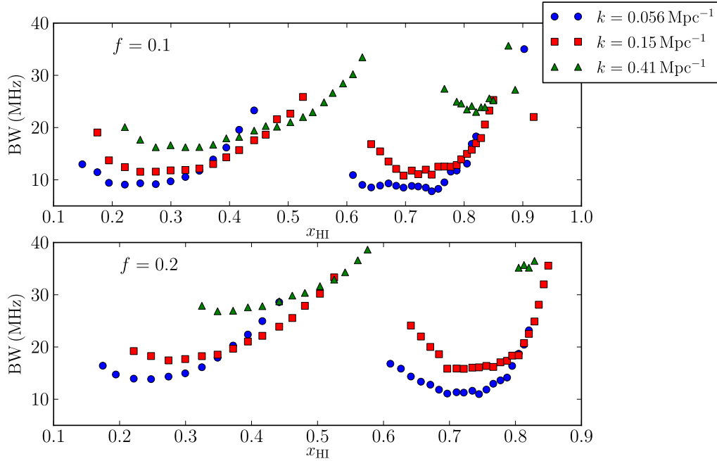
Figure 13. The optimum bandwidth for analysing observed EoR H I 21-cm data as a function of the neutral fraction x_{\text{HI}} for different k -modes. The gap in each line around x_{\text{HI}} \sim 0.5 to 0.7 indicates that the optimum bandwidth for those neutral fractions are much higher than full box size.
