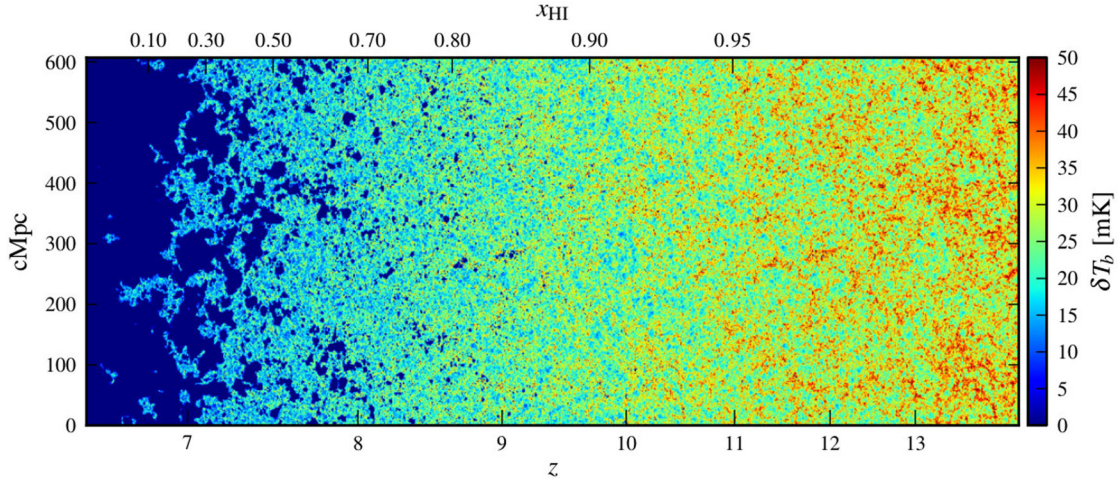
Figure 1. A slice through the 21-cm brightness temperature LC volume from the numerical simulation.
