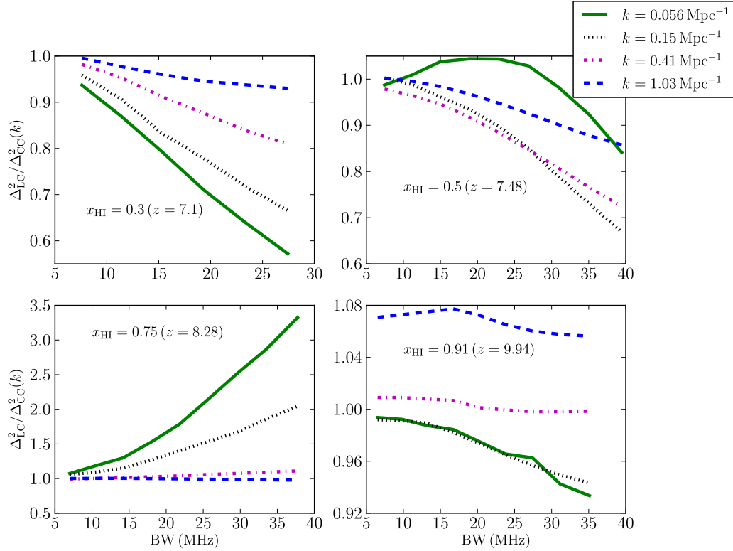
Figure 12. The ratio between power spectra with and without the LC effect as a function frequency bandwidth over which the power spectra have been evaluated. Note that the scale on the y-axis is different for the different panels.
