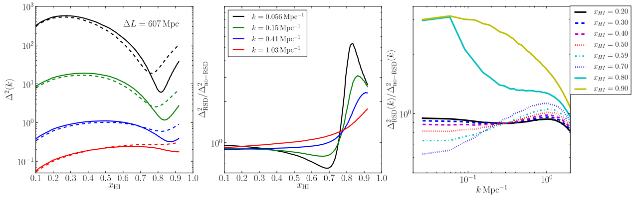
Figure 4. Same as the lower panel of the Fig. 3, except here we include the redshift space distortion effect but not the LC effect. The solid and dashed lines in the left-hand panel correspond to the spherically averaged power spectrum without and with the redshift distortion effect, respectively.
