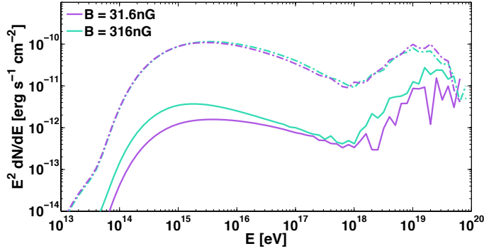
Fig. 2. Solid lines: the energy flux of secondary leptons produced by \pi\gamma interactions in a 3 Mpc magnetised region around a source at redshift z = 0.14 that emits UHECRs with L_{\text{cr,iso}} = 10^{47} \text{ erg s}^{-1} . The volume-averaged magnetic field strength in the magnetised region is \bar{B} = 31.6 \text{ nG} (purple), 316 \text{ nG} (green). The noise in the pion bump is due to the finite number of particles injected in our simulations. Dot-dashed lines: the energy flux of secondary leptons produced by \pi\gamma interactions beyond the first 3 Mpc of propagation.
