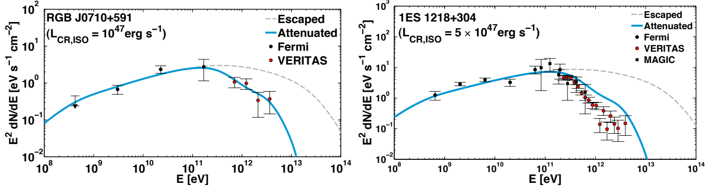
Fig. 6. The expected photon energy flux, resulting from the UHECR secondary electron synchrotron model a magnetised region with average magnetic field strength \bar{B} = 100 nG for RGB J0710+591 ( left ) and 1ES 1218+304 ( right ). Long-dashed lines show the spectrum that escapes from the magnetised region. Blue solid lines show the spectra with account of the attenuation by the EBL, for which the model of Kneiske & Dole (2008) has been considered.
