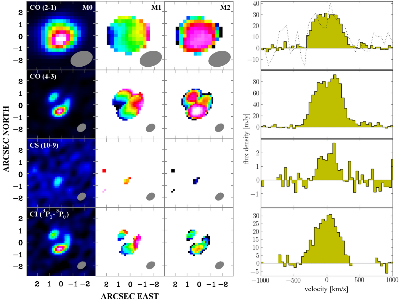
Fig. 4. Moment maps and line profiles of the emission lines detected in H1429–0028 as observed by ALMA: CO(2 → 1) on the first (upper) row ; CO(4 → 3) on the second row ; CS(10 → 9) on the third row ; [CI ^3P_1 \rightarrow ^3P_0 ] on the fourth row . The columns show different image moments: moment 0 (M0, velocity-integrated flux, left ), 1 (M1, velocity map, middle ), and 2 (M2, dispersion map, right ). Natural weighting was adopted to produce the moments. The beam is shown at the lower right in each panel as a shaded ellipse. Axes units are arcseconds. Colour scales of M0 are from -0.3 to 8 ( first row ), 18 ( second ), 2 ( third ), 5 \text{ Jy km s}^{-1} ( fourth ). Colour scales in M1 and M2 are, respectively, -200 to 200 \text{ km s}^{-1} and 0 to 170 \text{ km s}^{-1} . The right-most column shows the line-profiles at a spectral resolution of 40 \text{ km s}^{-1} . The first row also shows the CARMA spectrum as a dotted line.
