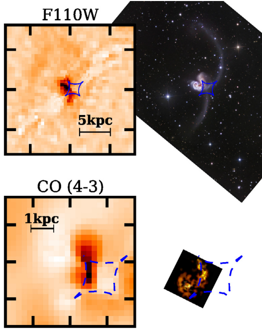
Fig. 9. Using the Antennae galaxy merger as a toy model to help visualise the background galaxy of H1429-0028. The two upper images show the F110W source-plane reconstruction from Fig. 8 (left hand-side) and the Antennae galaxies as seen in the optical (right hand-side). The two bottom images show the CO ( J:4 \rightarrow 3 ) velocity-integrated flux source-plane reconstruction from Fig. 8 (left hand-side) and the CO ( J:J^{\text{up}} = 1, 2, 3 ) map in the Antennae galaxies as observed by ALMA. Image credits: NASA, ESA and Ivo Saviane (upper-right picture), ALMA (ESO, NRAO, NIAO; bottom-right picture).
