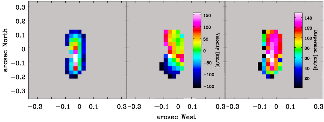
Fig. 10. Source-plane dynamical properties of H1429-0028. The left hand-side panel shows the velocity-integrated intensity map. The middle panel shows the velocity field, while the right hand-side panel shows the velocity dispersion map. Colour scales for the middle and right panels are given by the inset bar.
