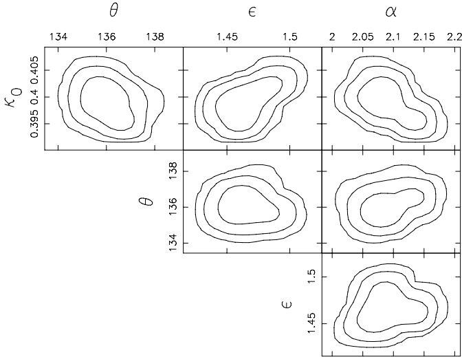
Fig. 7. Parameter confidence space. Parameters shown are the normalisation surface mass density ( \kappa_0 in units of 10^{10} M_\odot \text{ kpc}^{-2} ), the lens elongation ( \epsilon ), the mass profile power-law index ( \alpha ), and the orientation of the lens semi-major axis ( \theta in degrees measured counter-clockwise from north).
