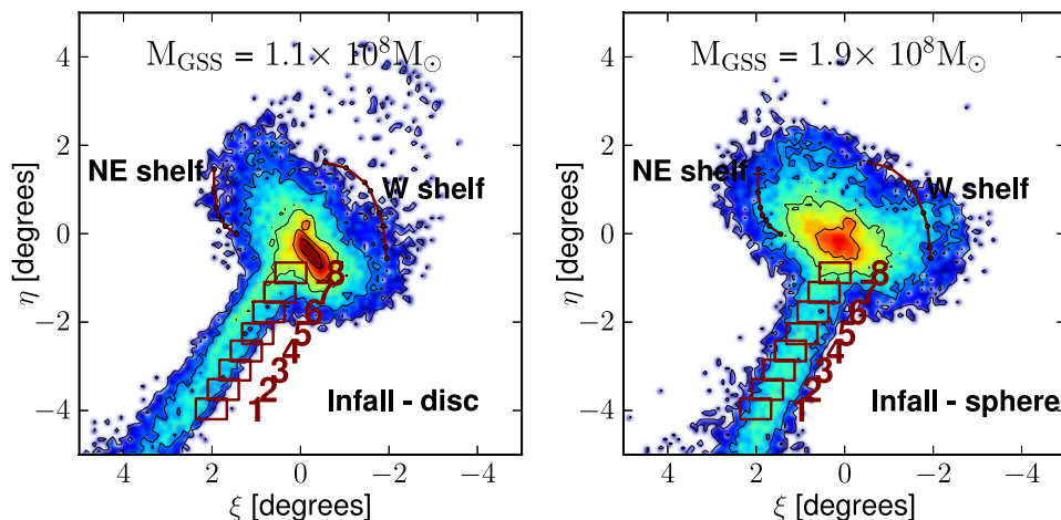
Figure 12. Stellar density maps in standard sky coordinates similar to Fig. 2 but for our cosmologically motivated ‘first-infall’ model plotted for a cold discy progenitor (left-hand panel) and a hot spheroidal dwarf progenitor (right-hand panel). Our simulations favour a dynamically hot spheroidal dwarf over a cold discy progenitor.
