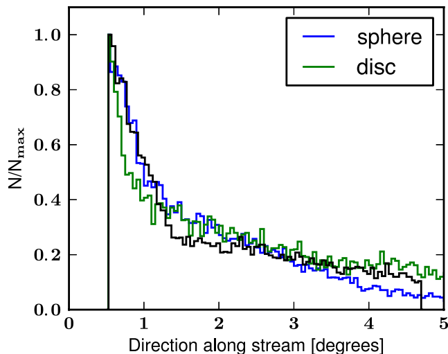
Figure 6. Stellar number density profile in the direction parallel to the stream. The black line shows the data from McConnachie et al. (2003). The blue line is the result from the spherical Plummer model while the green line corresponds to model Disc6. Since the number of stellar particles in the stream in our simulations is vastly superior to the number of observed stars, we normalize each profile by their respective maxima in order to be able to compare them directly to the observed profile. Furthermore, we exclude particles that are outside the region corresponding to the observed fields when calculating the profiles from our simulations.
