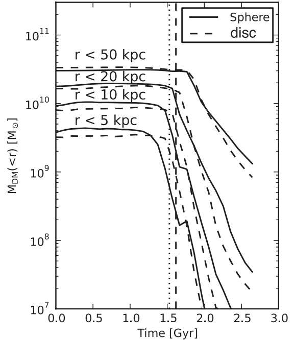
Figure 18. Evolution of the enclosed dark matter mass M_{\text{DM}(<r)} of the satellite as a function of time for different radii r in our first-infall N -body models. The solid and dashed line correspond to a spherical or a disc progenitor, respectively. The vertical dotted line indicates the time when the satellite is at r \sim 40 kpc, which is the starting point for various empirical models, discussed in Section 3. The vertical dashed line corresponds to the pericentric passage. Due to the highly eccentric orbit required to reproduce the GSS, in both models the satellite is able to retain a significant fraction of its dark matter halo as it falls towards M31 from 200 to 40 kpc.
