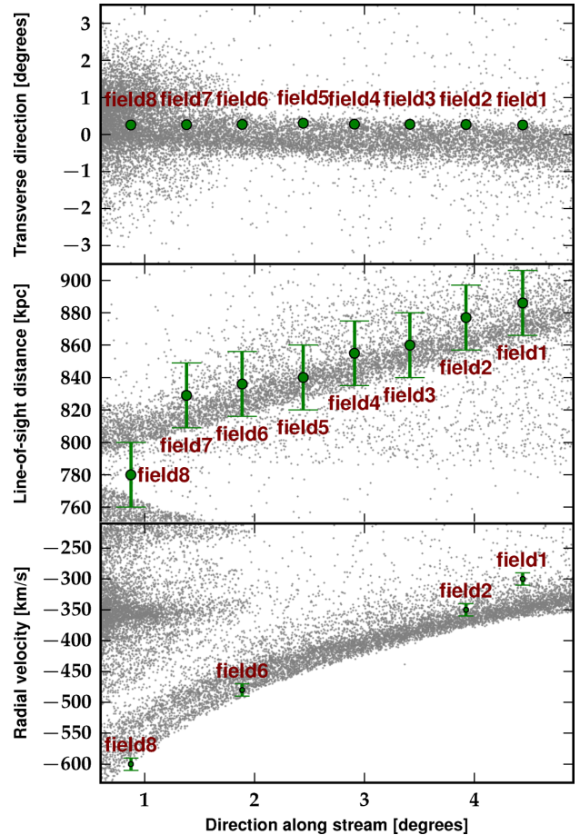
Figure 14. Comparison of results from our N -body simulation of the first-infall model using a discy satellite (grey dots) to the observational data (green points with error bars). The figure is similar to Fig. 4. The agreement with the data is poorer than that of our model with a spherical progenitor (see Fig. 13).
