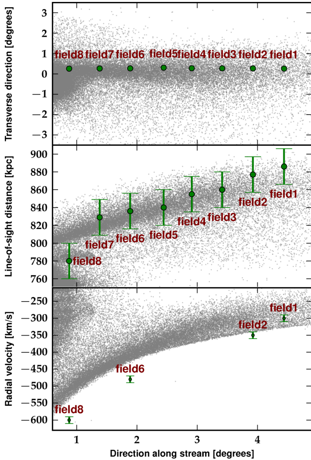
Figure 4. Comparison of N -body results from the Plummer model with positional and kinematical data of the GSS: position in stream-aligned coordinates (top panel), heliocentric distance (middle panel) and radial velocity (bottom panel) as a function of distance along the stream. Green filled circles show the data points corresponding to the fields 1–8 of McConnachie et al. (2003). Radial velocity measurements are taken from Ibata et al. (2004) and are only available in four of these fields. The particles of the progenitor in our simulation are represented as grey dots. The model is able to fit reasonably well the observations and can reproduce the distance–position correlation quite well. However, the phase plot (bottom panel) shows clearly that the velocity along the stream is mostly underestimated.
