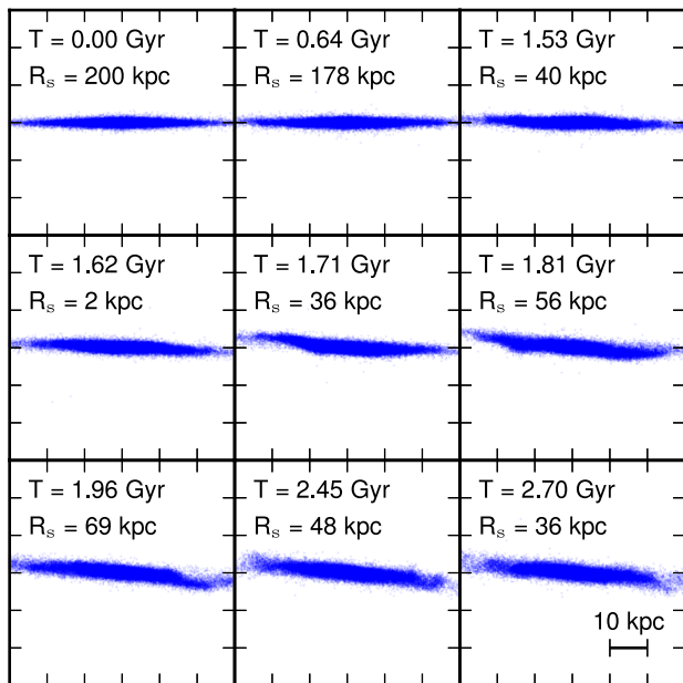
Figure 19. Edge-on view of the M31 disc at different times in our first-infall model with a spherical infalling satellite. The disc is visibly perturbed by the passage of the satellite and exhibits a warp-like structure at later times. The time after the start of the simulation and the orbital radius R_s , which is the distance of the centre of mass of the satellite to M31, is indicated in each frame.
