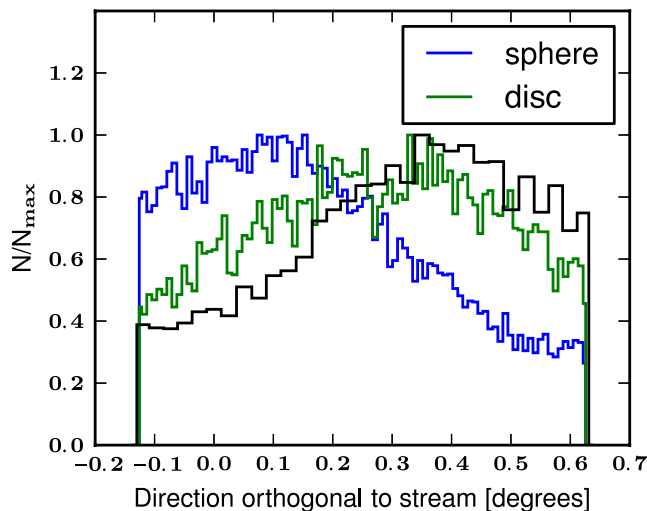
Figure 7. Stellar number density profile of satellite stars in the direction orthogonal to the stream. The lines have the same meaning as in Fig. 6. The GSS shows an asymmetry in the stellar distribution in the transverse direction which is better reproduced by a cold disc satellite than a dynamically hot progenitor.
