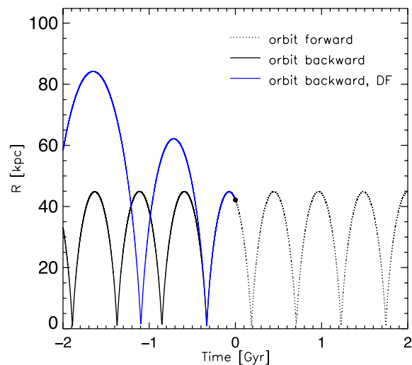
Figure 8. Tracing the progenitor orbit back in time: (x, y) projection (top) and orbital radius evolution (bottom) for the numerically integrated orbits for initial conditions given by equation (5) for the empirical models. The dotted line represents the forward integration from the initial point (denoted with a filled circle) while the solid lines correspond to the past of the progenitor with (blue line) and without (black line) DF.
