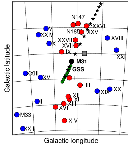
Figure 9. The sky map of the satellites of M31 is shown (see Conn et al. 2013; Ibata et al. 2013 for full details). We have shown the positions of the giant stream (GSS) by the filled green circles. The grey box shows the initial position for the GSS progenitor in the previous empirical models (see equation 5 in Section 3). The orbit of the progenitor satellite given by the N -body simulation of our first-infall model (see Section 5) is shown by stars, which lies almost on the same thin plane as most of the satellites of M31. In our model, the progenitor satellite is accreted from a large first turnaround distance of about 200 kpc.
