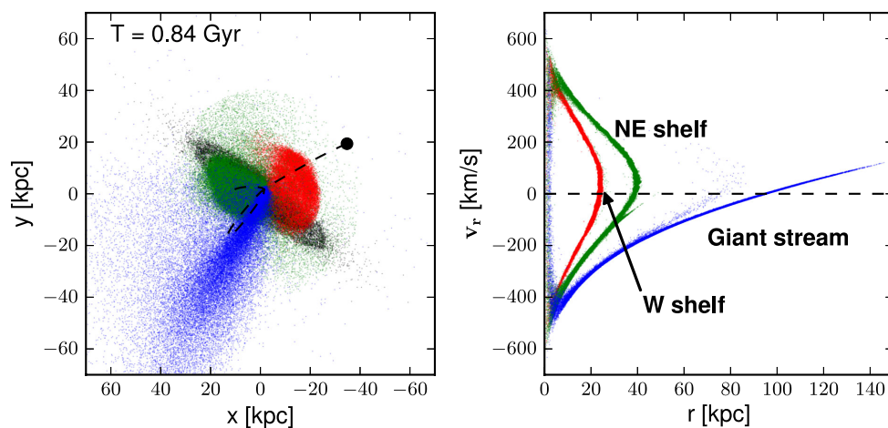
Figure 1. Real space x-y (left-hand panel) and phase-space r-v_r (right-hand panel) projection of stellar particles in the progenitor satellite with a Plummer profile at the final time, t = 0.84 Gyr. On the x-y projection, we also show the particles that compose the disc of M31 (black dots) and the orbit of the progenitor (dashed line) as traced by the initially-most-tightly-bound particles. In both panels, the particles of the progenitor are colour-coded by the number of their pericentric passages: 1 (blue), 2 (green) or 3 (red).
