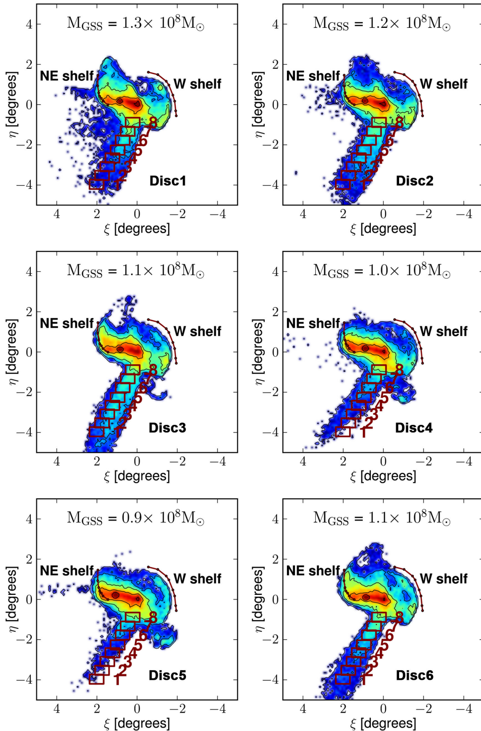
Figure 3. Disc progenitors: stellar density maps in standard sky coordinates at t = 0.84 Gyr for the six disc models of the satellite studied here. The six models differ only in the initial orientation of the disc of the infalling satellite w.r.t. M31. The plots have the same representation as the Fig. 2. We see that all models, initialized with a disc progenitor, tend to underestimate the stream mass which has an observed value of M_{\text{GSS}} \sim 2.4 \times 10^8 M_{\odot} . The best overall agreement with the GSS data (see also Fig. 5) is obtained for model Disc6 corresponding to a satellite whose major axis is perpendicular to that of M31.
