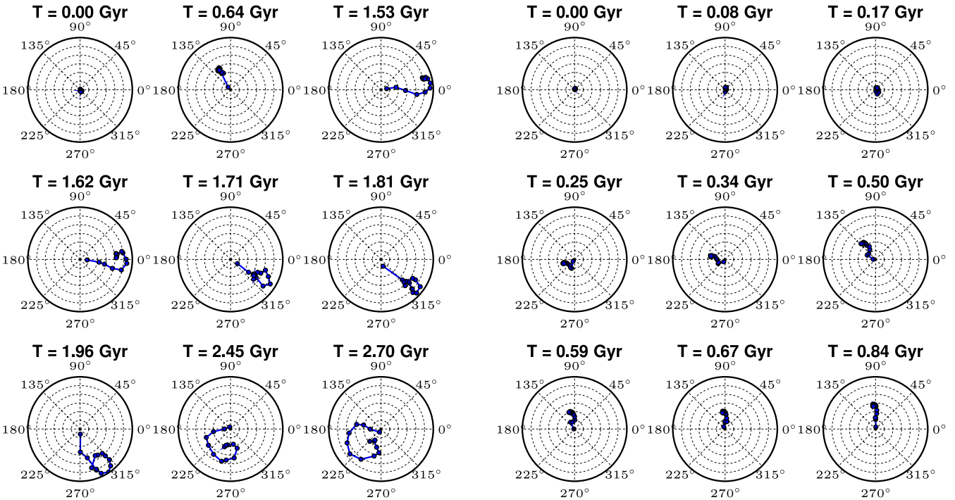
Figure 21. The diagram of the line of nodes showing the time evolution of the warp of M31 in our first-infall model, discussed in Section 5. The snapshots are shown from the start of the simulation ( T = 0 Gyr) to the last time step ( T = 2.7 Gyr) which corresponds to the present time. To make this diagram, the disc of M31 is divided into concentric annuli of width of about 1 kpc starting at 3 kpc from the centre of M31 disc. The radial coordinate is the warp or inclination angle that an annulus of the disc makes with the inner disc plane, shown at 1^\circ intervals. The azimuthal coordinate gives the azimuth of the line of nodes. The solid points are plotted for the radially ordered annuli at 1 kpc intervals, apart from the first central point which is averaged over 3 kpc annulus. At the start of our simulation, there is no warp, and all points crowd at the centre of the diagram. After the passage of the satellite through M31, the line of nodes first form a straight line and then form a spiral when the differential rotation sets in (Briggs 1990). The warp rotates clockwise and has a winding period of about 3 Gyr.
