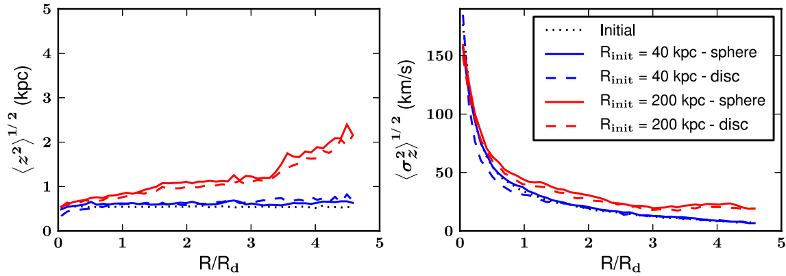
Figure 20. Heating of the disc of M31 due to the perturbations from the satellite in the N -body models that we studied in this work. The results are shown for both discy and spherical progenitors and also for empirical models with a dark-matter-poor satellite ( R_{\text{init}} = 40 kpc), studied in Section 3, and our first-infall models with a dark-matter-rich satellite ( R_{\text{init}} = 200 kpc), studied in Section 5. Mean vertical height \langle z^2 \rangle^{1/2} and the vertical velocity dispersion \langle \sigma_z^2 \rangle^{1/2} as functions of cylindrical radius in units of the scale radius R_d = 5.4 kpc (see Table 1) of the disc are plotted. In both of our first-infall models, the passage of the satellite significantly disturbs the disc because the progenitor retains a large fraction of its dark matter mass. The panels show that the outer regions of the disc ( R > 2R_d ) are heated and become thicker with respect to the inner parts, in our cosmologically motivated first-infall model.
