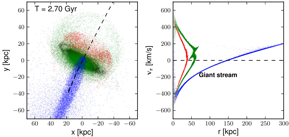
Figure 11. Distribution of stellar particles in the satellite in the x – y plane (left-hand panel) and the phase plot in the r – v_r plane (right-hand panel) at t = 2.7 Gyr for our first-infall N -body model using a spherical progenitor. The plots represent the same quantities as in Fig. 1 but are now made for our first-infall model. Although difficult to identify in real space, the presence of two tidal caustics corresponding to a second and a third orbital wrap are clearly seen in the phase space (right-hand panel). The NE shelf shown in green and the W shelf shown in red, near the zero velocity surfaces, correspond to stars on their second and third pericentre passages, respectively. The position of the remnant of the satellite, which lies in the region of the NE shelf, is clearly seen in this plot which is in agreement with results from a recent statistical approach (Fardal et al. 2013).
