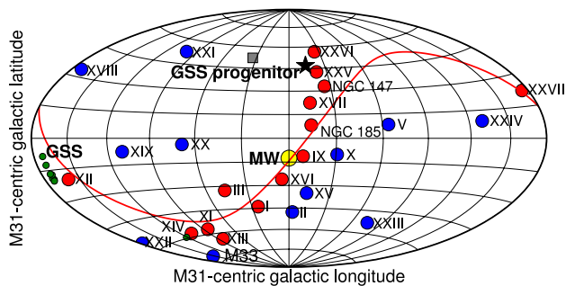
Figure 10. This map is similar to Fig. 9 but all positions are now viewed from Andromeda. We show the initial position of the satellite in our first-infall model (see equation 6 in Section 5) by star. The thin plane containing many of the M31 satellites is also drawn (see Conn et al. 2013; Ibata et al. 2013 for full details). The position of the giant stream (GSS) is also shown on this map by green filled circles.
