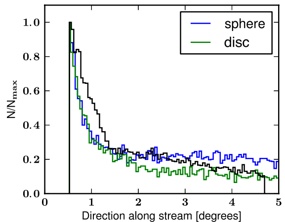
Figure 15. Density profile of satellite stars calculated in the direction parallel to the stream (same as done for Fig. 6) for our first-infall models. The black line shows the data from McConnachie et al. (2003). The blue line is the result from the spherical Plummer model while the green line corresponds to a discy satellite. We find minor deviations from the observed profile (black line) with a steeper shape at small distances and a shallower behaviour at large radii for both a spherical (blue line) or disc (green line) satellite. The length of the stream is broadly consistent with its observed value.
