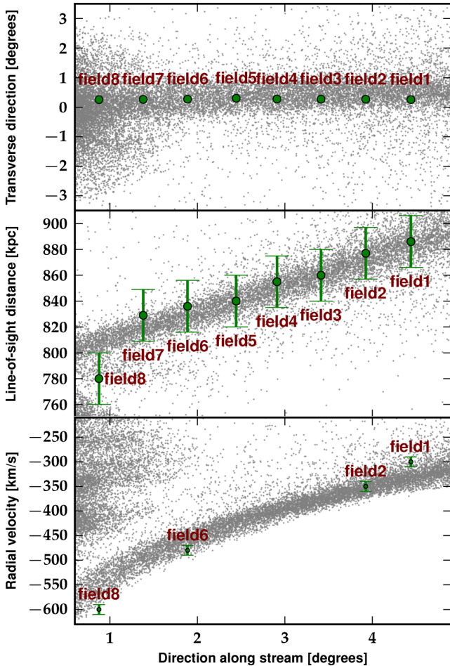
Figure 13. Comparison of results from our N -body simulation of the first-infall model using a spherical Plummer satellite with observational data for the GSS. The figure is similar to Fig. 4. Our cosmologically motivated first-infall scenario for the formation of the giant stream successfully reproduces the stream’s three-dimensional position and kinematics.
