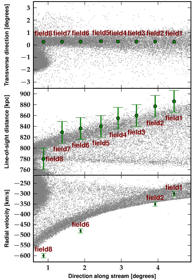
Figure 5. The figure compares the results from our N -body simulation for model Disc6 with the observational data. This figure is similar to Fig. 4 but is now made for a discy satellite. Compared to the spherical Plummer satellite (Fig. 4), the disc model shows a larger spread in the distance–position correlation (middle panel). A disc satellite also fails to properly model the radial velocity data which, apart from the farthest data point, are systematically underestimated (bottom panel).
