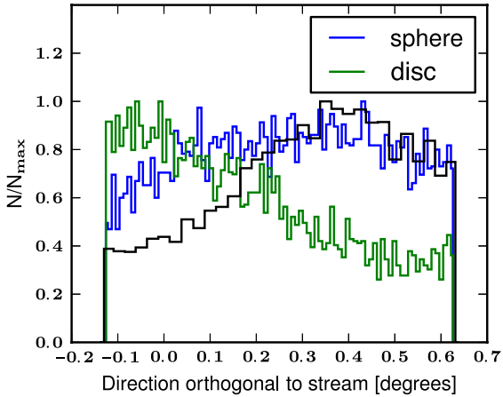
Figure 16. Density profile of satellite stars calculated in the direction transverse to the stream as presented previously in Fig. 7 but now for our first-infall models. The black line shows the data from McConnachie et al. (2003). The blue line is the result from the spherical Plummer model while the green line corresponds to a discy satellite. The spherical progenitor clearly reproduces better the asymmetric shape of the profile than the discy satellite.
