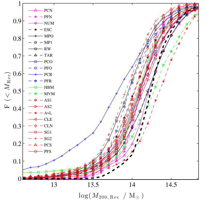
Figure 5. The CDF of recovered halo mass delivered by the 23 methods when the group/cluster membership is not known. The true M_{200} CDF is shown via the thick black dashed line. It is clear that all methods are recovering lower halo masses than that of the ‘true’ mass. A two-sample Kolmogorov–Smirnov (KS) test also demonstrates that the recovered mass distributions are not statistically similar to the true mass distribution (delivering p -values for all methods p \leq 0.01 ).
