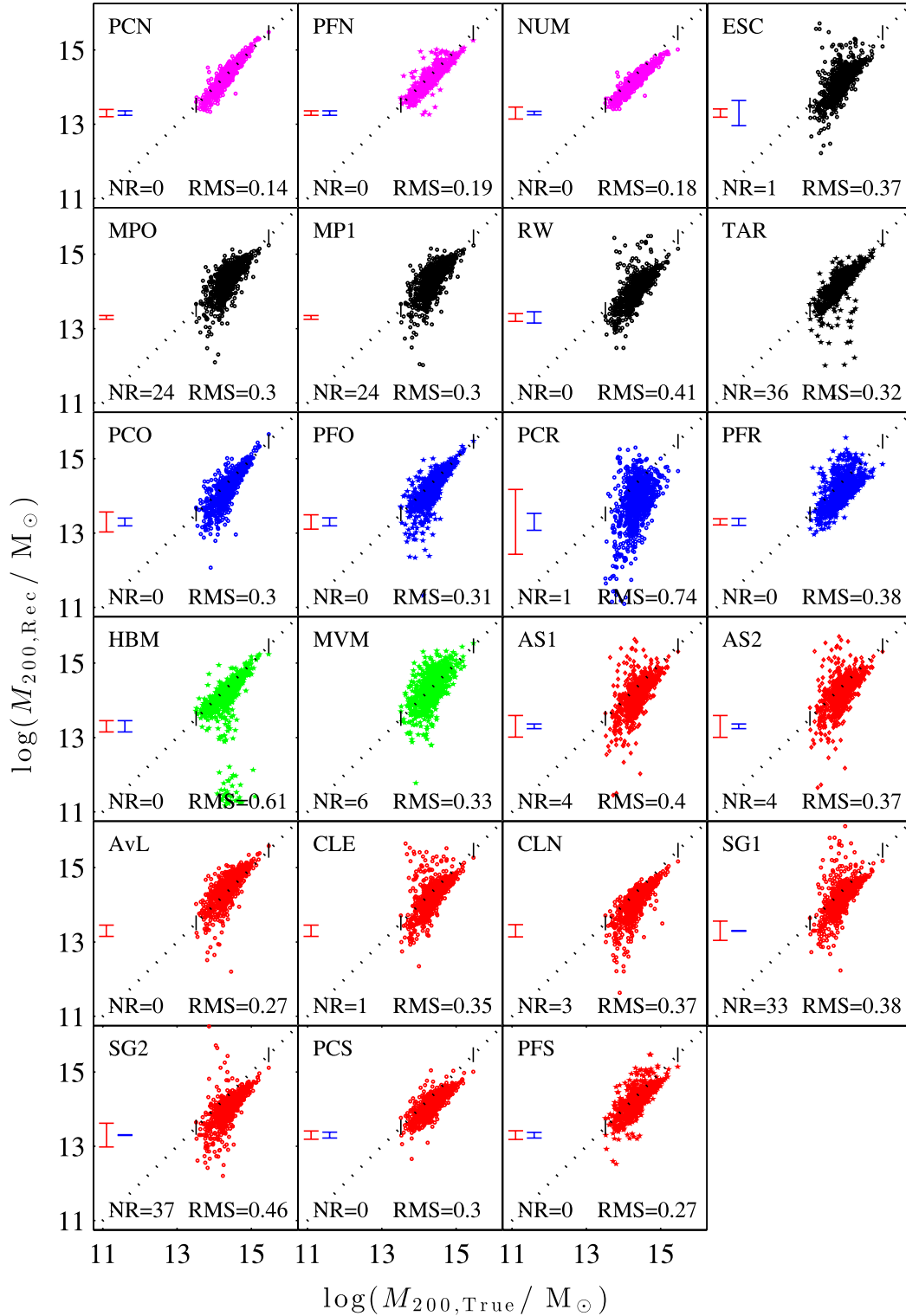
Figure 3. Recovered versus true mass when the group/cluster membership is not known. The black dotted line represents the 1:1 relation. ‘NR’ in the legend represents groups/clusters that are not recovered because they are found to have very low ( <10^{10} M_{\odot} ) or zero mass. The black ticks that lie across the 1:1 relation represent the minimum and maximum ‘true’ halo M_{200} . The vertical red bar represents the mean statistical error delivered by methods and the vertical blue bar represents the mean systematic error delivered by methods.
