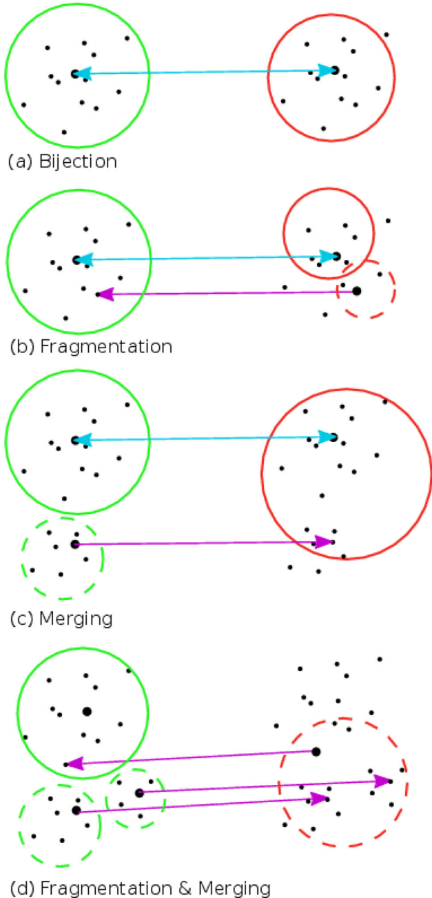
Figure 3. Schematic links between true groups (green circles) and FoF-extracted groups (red circles), each with their respective MMG (black dots). The solid circles represent primary true and FoF groups, while the dashed circles respectively correspond to secondary true groups and FoF fragments. The cyan double arrows each indicate the one-to-one correspondence between the MMG in the true and extracted groups. The purple rightwards-pointing arrows correspond to the MMG of a true group ending up as a galaxy that is not the most massive of its extracted group. The purple leftwards-pointing arrows represent the cases where the MMG of an extracted group is not the most massive of its parent true group.
