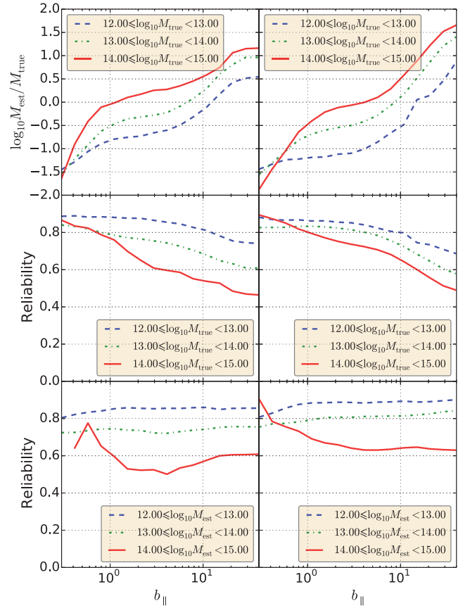
Figure 11. Variation of the mass bias and reliability as a function of b_{\parallel} for b_{\perp} = 0.1 , for subsamples 2 (left) and 6 (right).
