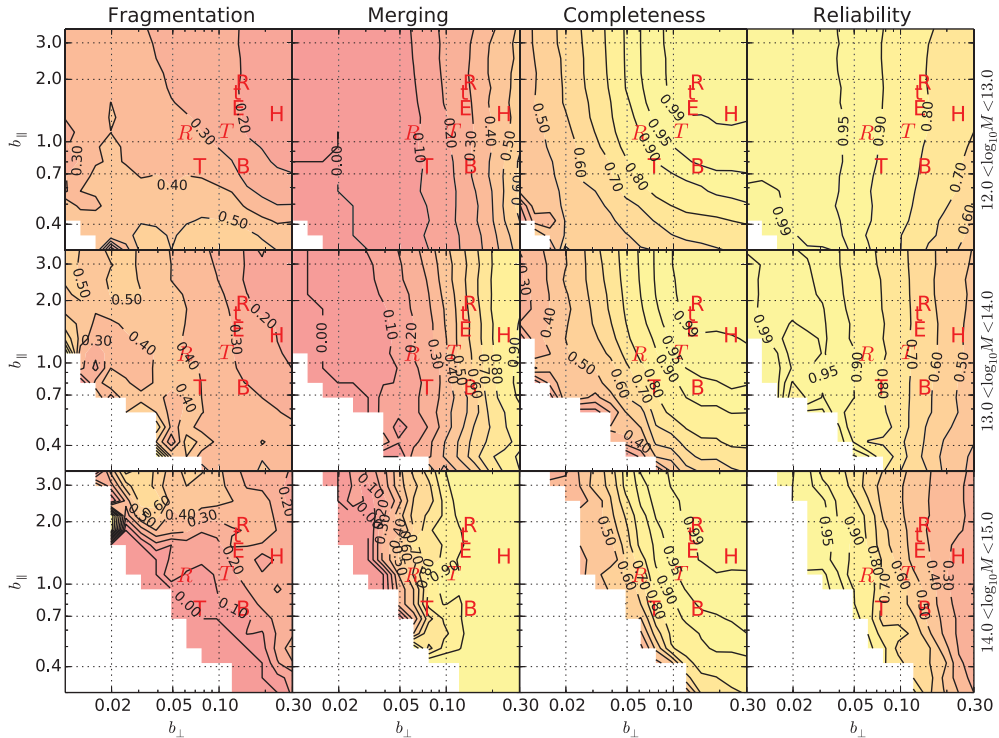
Figure 5. Same as Fig. 4, but where the different rows correspond to different bins of extracted group masses estimated from the virial theorem. The white zones show cases where the LLs led to no unflagged groups extracted.
