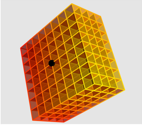
Figure 1. A representation of the full mock galaxy catalogue. Each small box is a 137 Mpc long cube. The observer is at the large black point in the middle of one of the square sides of the superbox.
