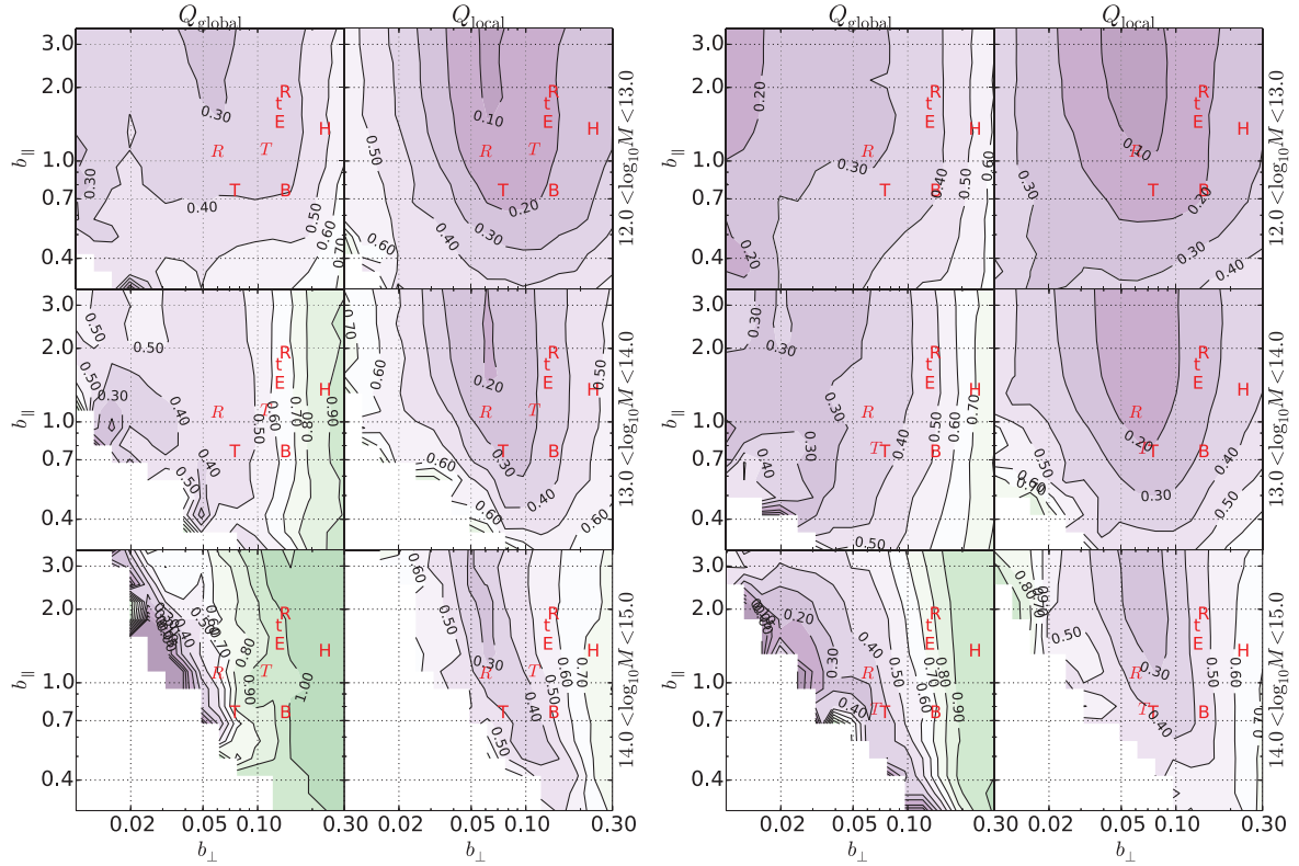
Figure 9. Same as Fig. 8 but in bins of estimated masses. The white zones show cases where the LLs led to no unflagged groups extracted.
