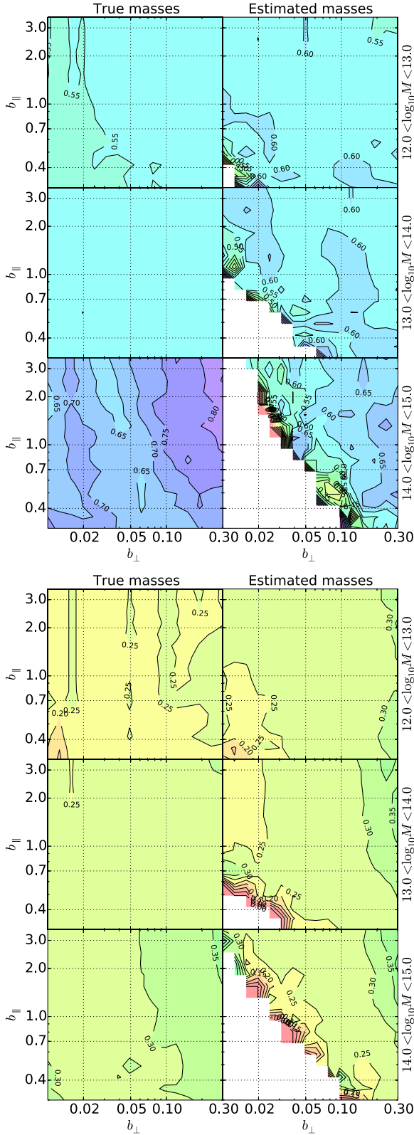
Figure B1. Fraction of selected groups flagged as either split by the transformations of the simulation box or lying close to the edges of the mock galaxy survey for catalogues 2 (top) and 6 (bottom), in bins of true and estimated masses.
