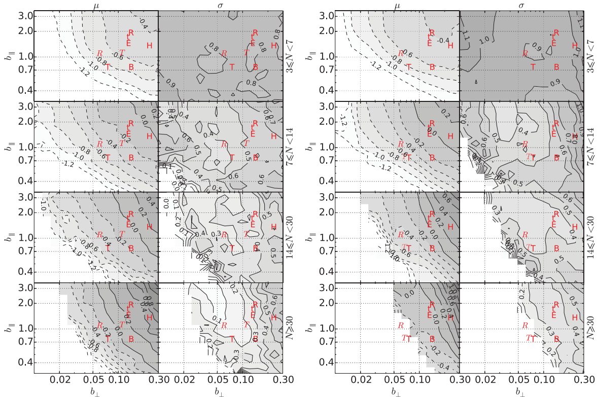
Figure 10. Bias ( \mu ) and inefficiency ( \sigma ) of the group masses estimated by the virial theorem (equation 17) on our 16 \times 16 grid of LLs, in four bins of extracted group richness (we do not consider extracted groups for which the parent true group has \leq 3 members). The bias and inefficiency are respectively computed as the median and half 16–84 interpercentile of \log_{10}(M_{\text{EG}}/M_{\text{TG}}) . Results are shown for primary, unflagged groups. The left and right panels are, respectively, for galaxy subsamples 2 and 6. The symbols are as in Fig. 4. The white zones indicate LLs with no unflagged groups extracted.
