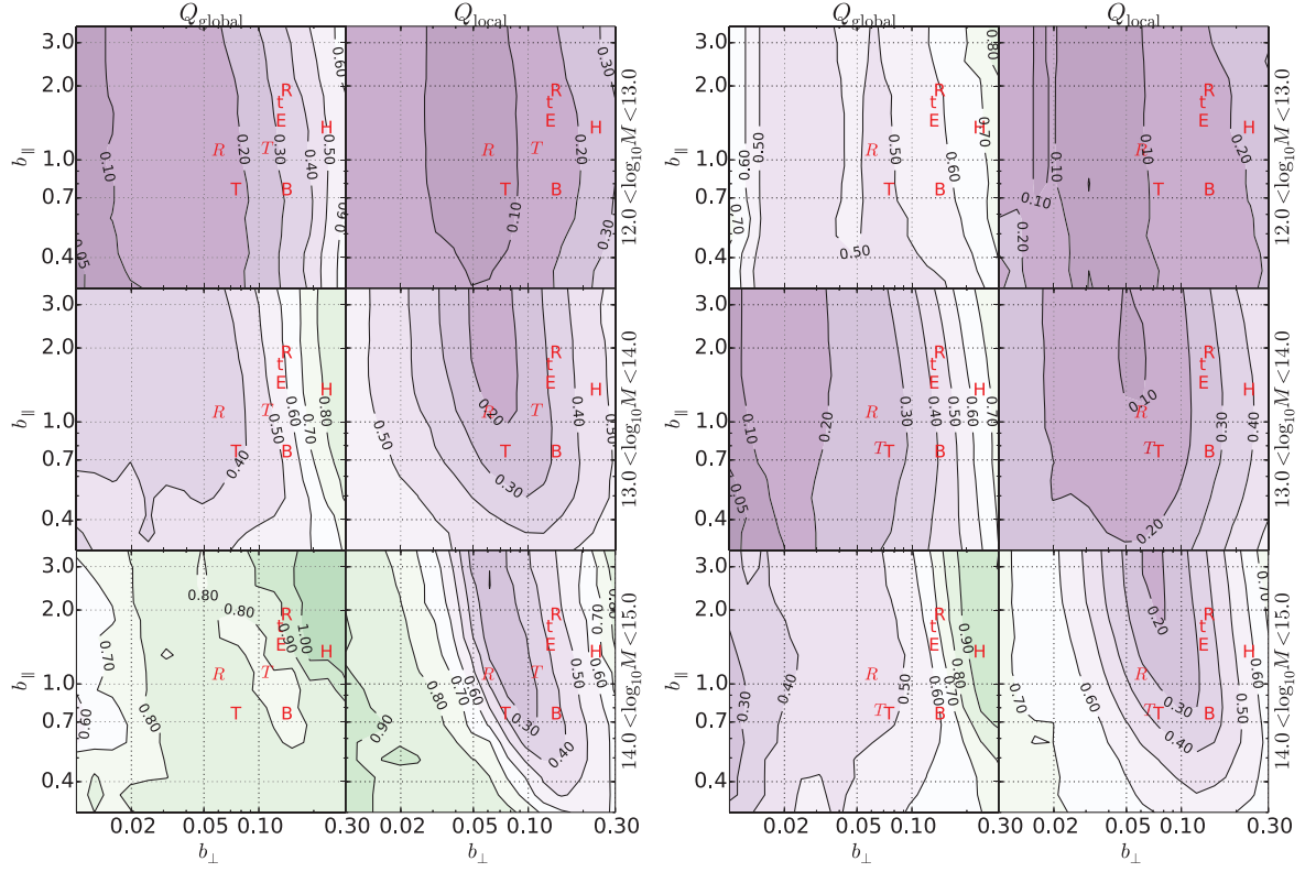
Figure 8. Global and local quality factors in a 16 \times 16 grid of LLs for subsamples 2 (left) and 6 (right), in three bins of true masses. Results are shown for unflagged groups (restricted to primary groups for Q_{\text{local}} ) of at least three members (in both the true and extracted group). The symbols are as in Fig. 4.
