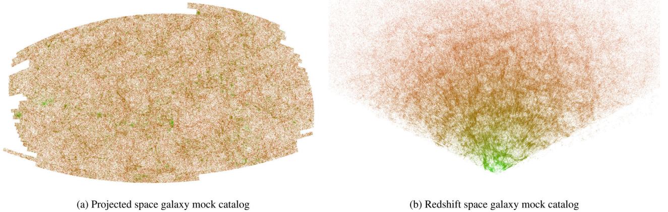
Figure 2. Views of our initial, flux-limited, 2.2 sr SDSS mock galaxy catalogue, projection on the celestial sphere (left) and 3D cone (right, not sliced). The colours provide the absolute r -band magnitude (green for low luminosity). (a) Projected space galaxy mock catalogue. (b) Redshift-space galaxy mock catalogue.
