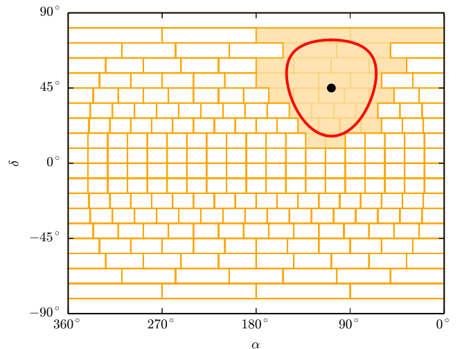
Figure A1. An illustration of the grid on the celestial sphere for a fast search of neighbours. Selected boxes to search are highlighted, for the given angular distance from the central point (red line). Note that both the search angle and the cell size are greatly exaggerated for illustrative purposes.
