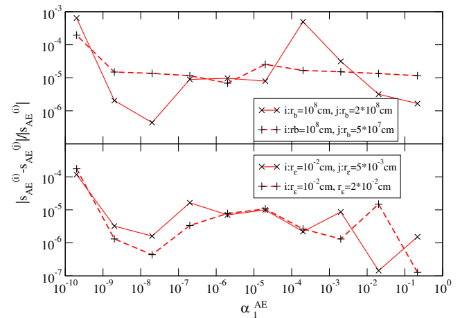
FIG. 5 (color online). The fractional difference in sensitivity against the PPN parameter \alpha_1^x in Einstein-æther theory for different boundary radius r_b (top) and core radius r_c (bottom) with the APR EoS. We set the coupling constants to c_1 = 2c_2 = 2c_3 = -2c_4 , with M_{\text{obs}} = 1.4M_\odot .
