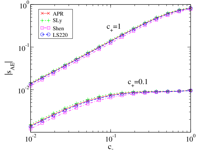
FIG. 4 (color online). The absolute magnitude of the sensitivity in Einstein-æther theory against c_- for c_+ = 1 and c_+ = 0.1 . We saturate the PPN parameters \alpha_1^x and \alpha_2^x and set the NS mass to M_{\text{obs}} = 1.4M_\odot .
