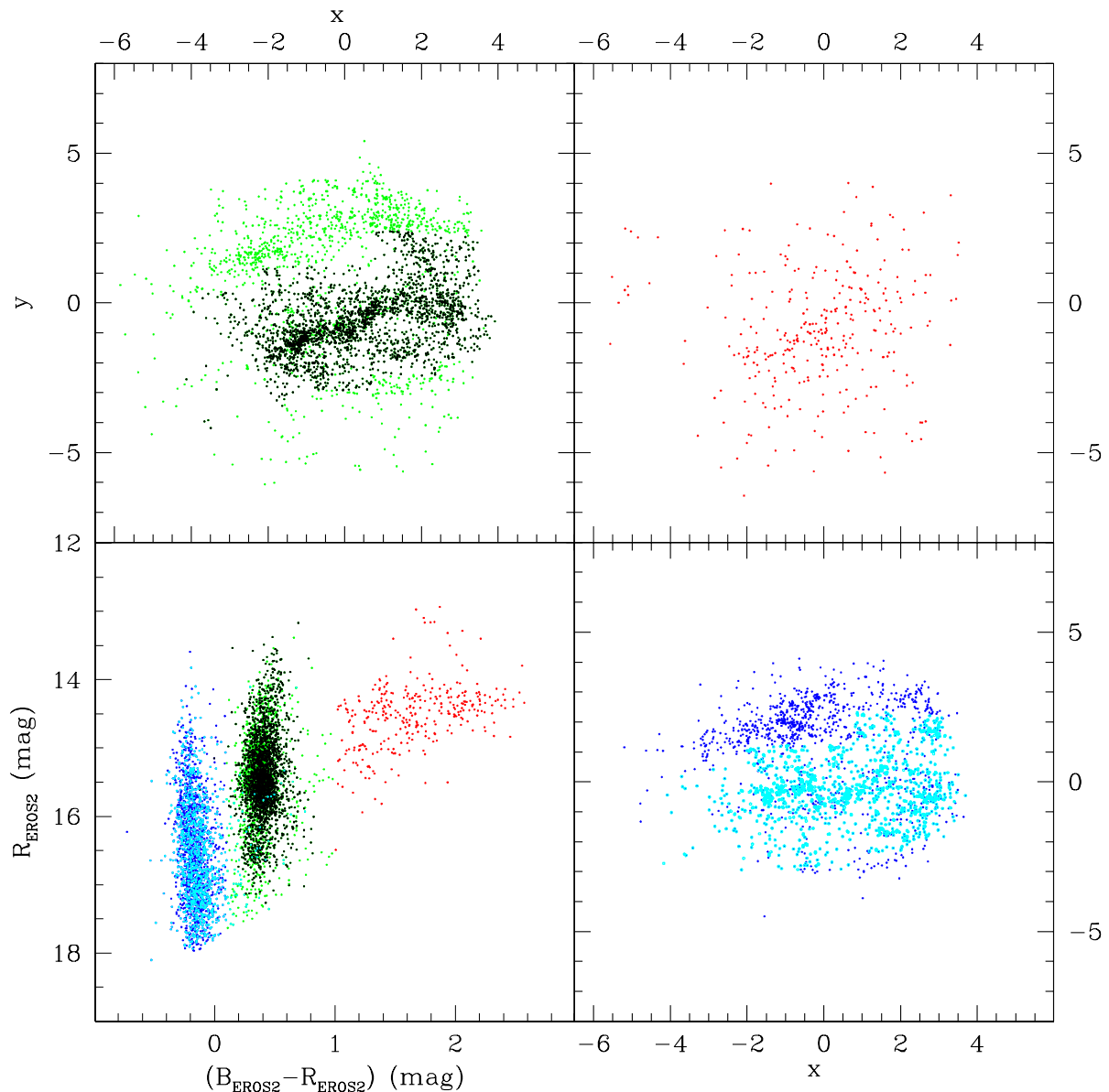
Figure 16. Lower-left panel: (R_{\text{EROS2}}, B_{\text{EROS2}} - R_{\text{EROS2}}) CMD of the EROS-2 CC candidates in the LMC. Blue, green and red circles indicate respectively hot ECLs, CCs and LPVs, according to our colour selection criteria (see the text for details). Upper-left panel: spatial distribution of the CCs; upper-right panel: distribution of the LPVs and binary systems (lower-right panel) that contaminate the list of EROS-2 CC candidates in the LMC. x and y are related to \alpha and \delta according to equations described in the Appendix.
