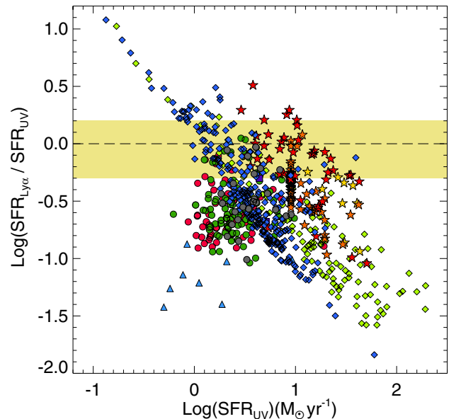
Fig. 12. SFR(Ly \alpha ) to SFR(UV) ratio as a function of SFR(UV). The color code for the local sample is the same as in previous figures. Several high- z samples are also included: green and blue diamonds (Gronwall et al. 2007; Guaita et al. 2010); yellow, orange, and red stars (Curtis-Lake et al. 2012; Taniguchi et al. 2005; Jiang et al. 2013). The SFRs are observed values not corrected for dust extinction. The dashed line corresponds to the SFR ratio of unity. The yellow region denotes the SFR ratio values that would be derived for different star formation histories (see text for details).
