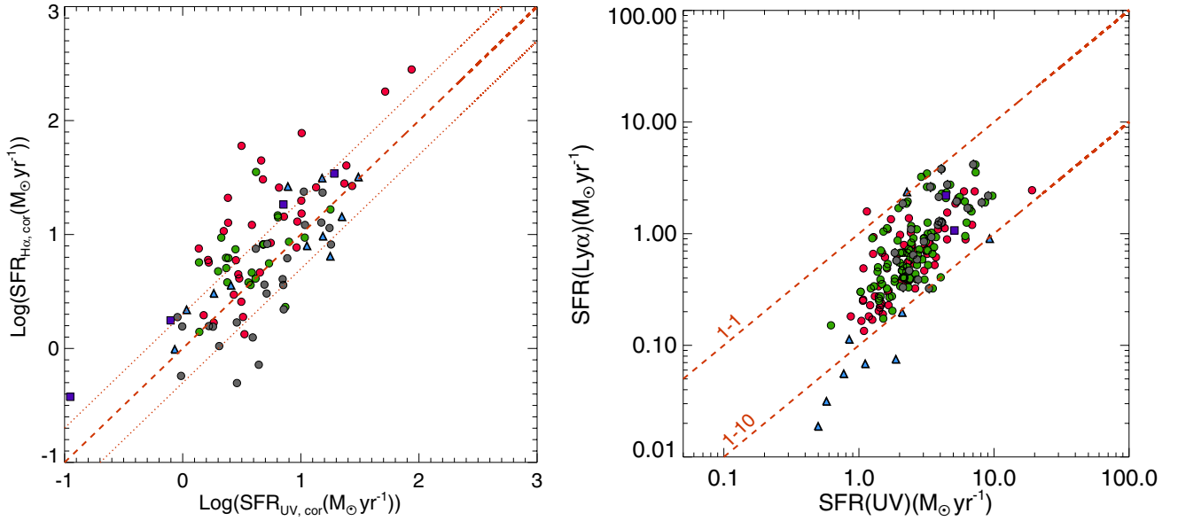
Fig. 11. Comparison between SFR indicators. The SFR values are calculated using Kennicutt (1998) calibration. The left panel shows SFR(H \alpha ) versus SFR(UV) both corrected for dust extinction derived from the Balmer decrement. The dashed line denotes the line of equality, while the dotted lines have a factor-of-2 deviation. The right panel presents the observed SFR(Ly \alpha ) as a function of SFR(UV), with no correction for dust extinction. The two dashed lines mark the 1:1 and 1:10 ratios for SFR Ly \alpha :SFR UV . The symbols are the same as in Fig. 10.
