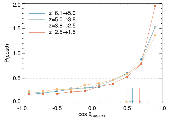
Figure 6. PDF of the cosine of relative angle between the spin of the advected gas, \langle \lambda \rangle_{v_r} , for different pairs of redshifts as labelled. The mean of this PDF is also represented as a vertical arrow for the various pairs of redshifts considered. The orientation of the spin of filaments is temporally coherent.
