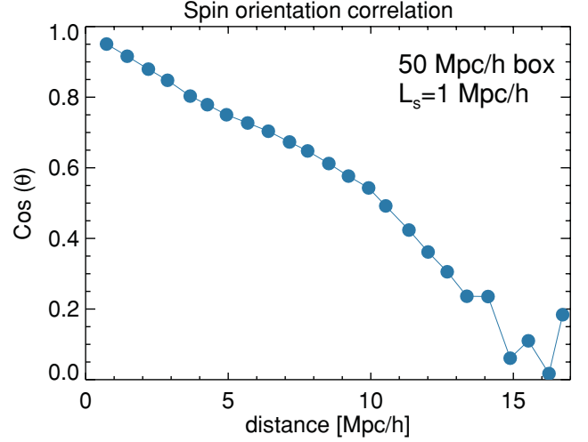
Figure B1. Expectation of the relative orientation of the angular momentum of the filamentary flow as a function of the separation along the filament; this quantity is found to be quite stable with regard to redshift.
