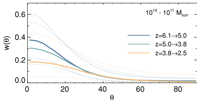
Figure 3. The covariances (thick line) between different redshifts (as labelled) of the thresholded density maps on the virial sphere, R_{\text{vir}} , together with the corresponding dispersion (interquartile, dotted lines). The lower bound of the thresholded density is chosen such that filamentary structures stand out, while the upper bound is adopted to minimize the signal from the satellites (see the text, Section 2). The orientation of filaments is temporally coherent, as is qualitatively illustrated in Fig. 2.
