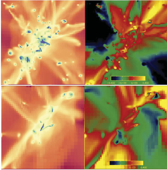
Figure 7. The distribution of the z component (i.e. along the spin axis of their dark matter halo) of the spin parameter ( \lambda_z , right-hand panels) at z = 3.8 in the HORIZON-MareNostrum simulation for two different mass haloes: 5 \times 10^{12} (top panels) and 3 \times 10^{12} M_\odot (bottom panels). Projections of the hydrogen density are shown in the left-hand panels. The field of view is 4 virial radii on a side. It is apparent that some filaments display large values of \lambda_z (colour coded in yellow).
