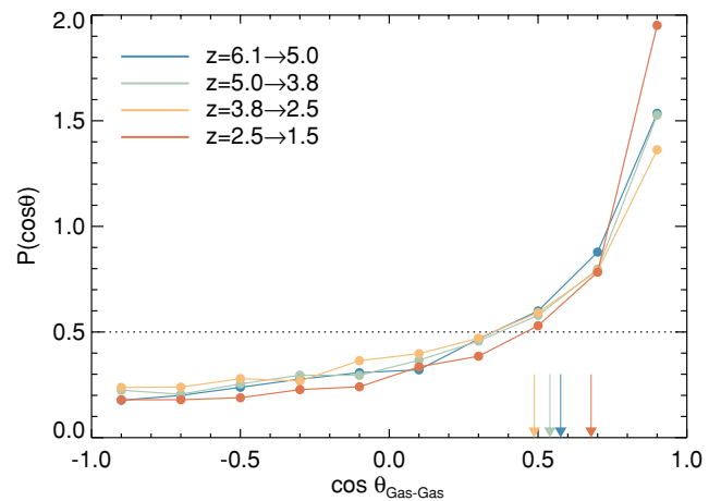
Figure 6. PDF of the cosine of relative angle between the spin of the advected gas, \langle j \rangle_{\text{vir}} , for different pairs of redshifts as labelled. The mean of this PDF is also represented as a vertical arrow for the various pairs of redshifts considered. The orientation of the spin of filaments is temporally coherent.
