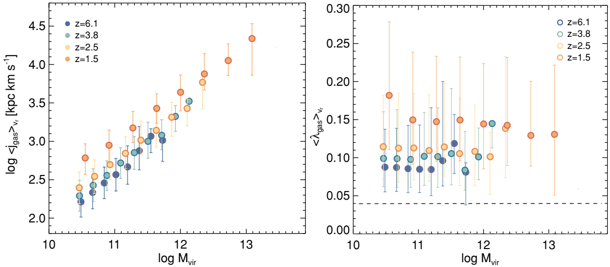
Figure 4. Left: advected specific momentum of gas as a function of cosmic time and mass in the HORIZON-MareNostrum simulation. Note that more and more gas angular momentum is being advected as a function of time and mass. Right: advected spin parameter of gas as a function of cosmic time and mass; a redshift trend persists, while the amplitude of the advected spin parameter is larger than the averaged value of 0.04 (indicated by the horizontal dashed line) measured for dark matter haloes independently of time and mass (Barnes & Efstathiou 1987; Kimm et al. 2011).
