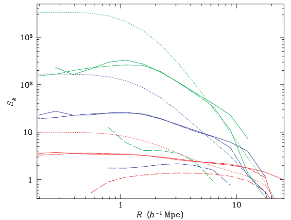
Figure 6. Hierarchical amplitudes S_k(R) for galaxy number count measured in from numerical simulations for k = 3, 4 and 5 (bottom to top). Solid lines show galaxy (substructure) S_k , and long-dashed lines show halo S_{k,h} . Dotted lines show the point cluster model expressions in equations (30)–(32).
