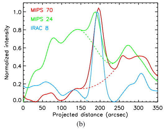
Fig. 3. a) Three color image as in Fig. 1 with the region along which the profiles are measured for the main “pillar of creation”. b) Normalized infrared emission profiles (MIPS70 in red, MIPS24 in green, and IRAC8 in blue, solid lines) and interpolations performed to measure the fluxes of the structure (dashed lines).
