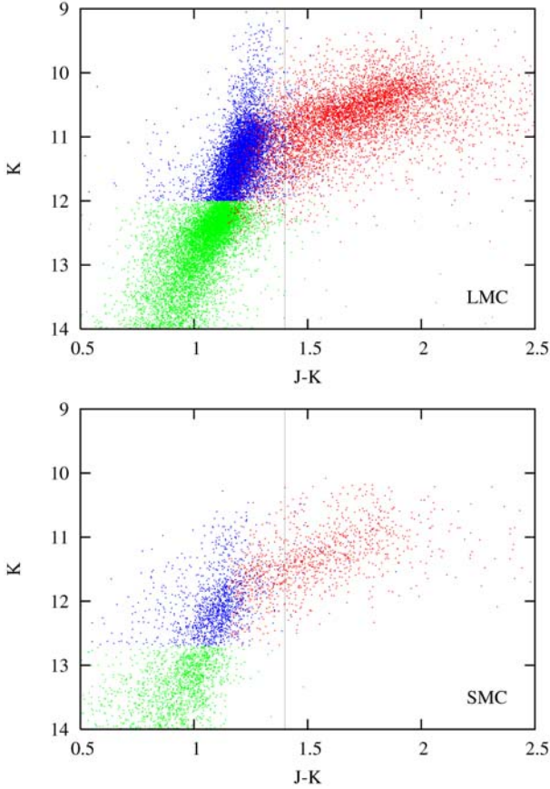
Fig. 8. K - J - K diagram for LMC and SMC red variables.
