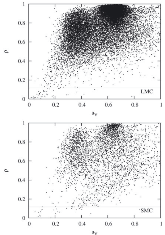
Fig. 3. Plot of the colour-magnitude correlation coefficient against the slope of magnitude-colour relation, for EROS LMC and SMC data. The correlation coefficient serves as a measure of quality of the slope a_V . The horizontal lines correspond to probability 0.995 of the null hypothesis H_0 , i.e. points lying above correspond to statistically significant correlation.
