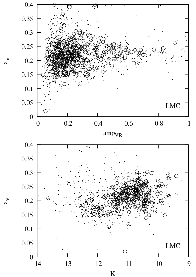
Fig. 11. Slope a_V against V - R amplitude amp_{VR} ( top ) and against 2MASS K magnitude, for MACHO LPV V and R photometry of the LMC. The C-rich stars are marked with circles.
