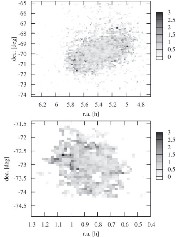
Fig. 12. Maps of the C/O ratio in the LMC (upper panel) and in the SMC (lower panel) obtained from EROS data using the a_V(J - K) method described in Sect. 4.4.
