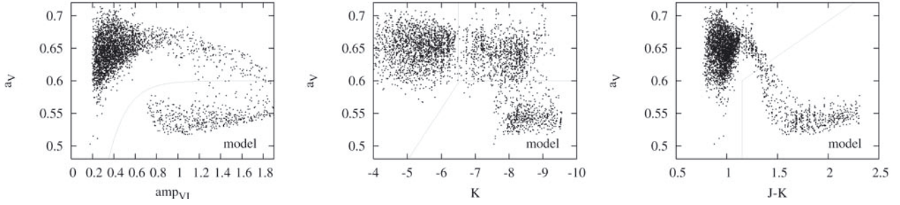
Fig. 13. Same as in Fig. 4 for the model slope parameter a_V calculated for real LMC stars using Marigo et al. (2003) model sequences (see text for details). Our crude model yields a clear separation of O-rich RGB, O-rich AGB, and C-rich AGB stars.
