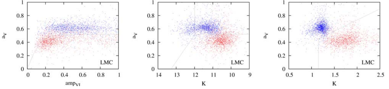
Fig. 10. Separation of C-rich, O-rich AGB, and red variables below the TRGB for LMC from OGLE LPV I and V photometry (Soszynski et al. 2005). The colour slope parameter a_V vs. the amplitude of colour change ( left panel ). The colour slope parameter a_V vs. K 2MASS magnitude ( middle panel ). Colour slope parameter vs. J - K colour ( right panel ).
