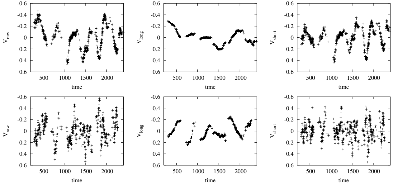
Fig. 1. Sample EROS light curves for two stars with spectral types assigned by Cioni et al. (2001): DCMC J052618.12-694100.0 of type C (top row) and DCMC J052446.91-694949.9 of type M (bottom row). The left, middle, and right panels present the raw, low-pass, and high-pass light curves, respectively. For details of filtering see Sect. 3.2
