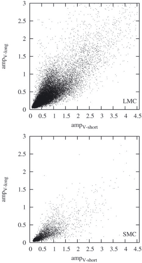
Fig. 15. Correlation between amplitudes of LSP and of shorter period variation for EROS LMC and SMC data. Crosses mark large-amplitude variables.
