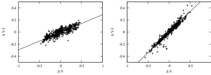
Fig. 2. Sample plot of raw colour and magnitude variations for the same 2 stars as in Fig. 1. We also plot the regression lines. Their inclination parameter is a_V , discussed in the text.
