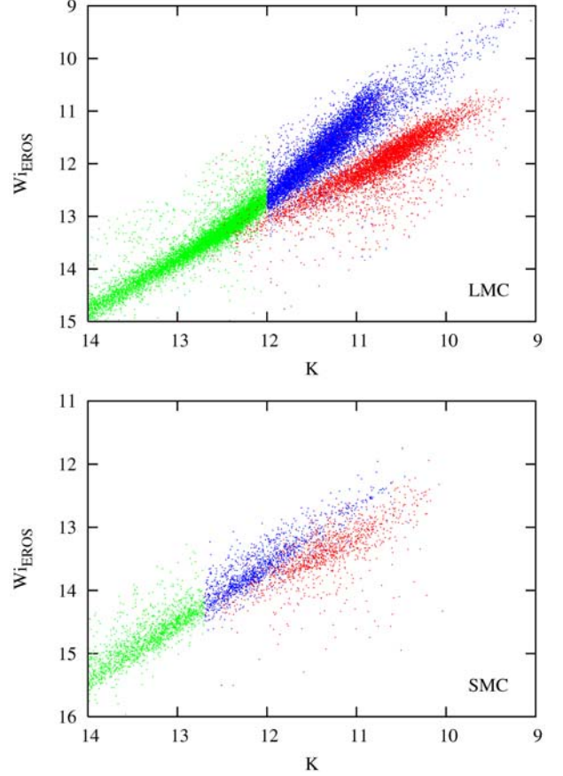
Fig. 9. EROS Wesenheit index vs. K magnitude, for LMC and SMC red variables. Wesenheit index is derived from EROS R and B magnitudes.
