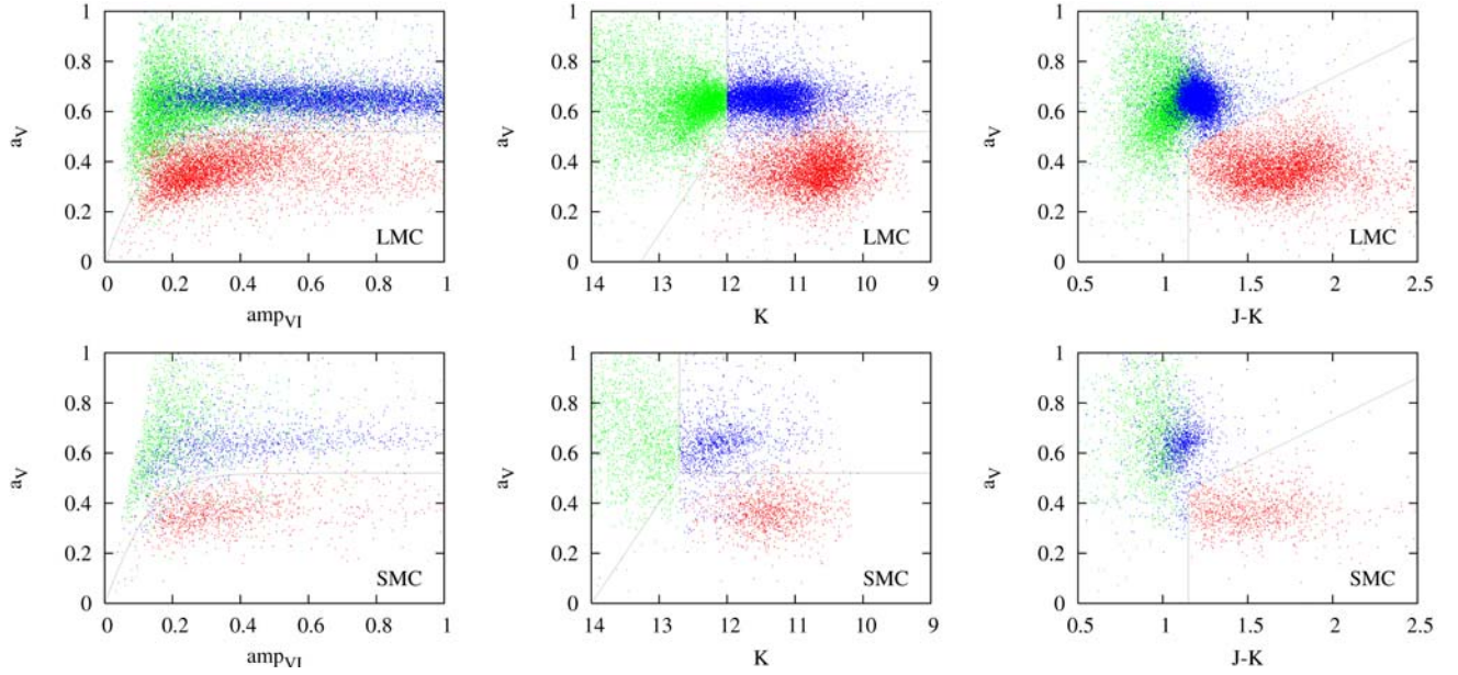
Fig. 4. Plots depicting three methods of distinguishing O- and C-rich variable stars ( from left to right ): slope-colour amplitude a_V(amp_{VI}) , slope- K magnitude a_V(K) and slope- J - K colour a_V(J - K) , for EROS LMC ( top ) and SMC ( bottom ) data. Vertical lines indicate adopted TRGB dividing RGB and AGB stars. See text for a detailed description of the methods and parameters of the boundaries. Black, dark grey, and light grey dots (blue, red, and green in electronic edition) respectively mark O- and C-rich AGB stars and O-rich RGB ones, classified using K magnitudes for AGB/RGB and leftmost panels for O/C content.
