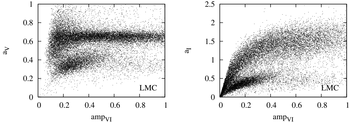
Fig. 5. Comparison of a_V plot in Fig. 4 with that for a_I .
