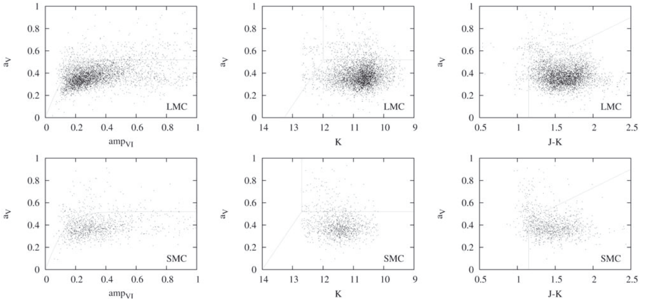
Fig. 7. C-rich stars in LMC (upper panels) from Kontizas et al. (2001) and Groenewegen (2004) and in SMC (lower panels) from Rebeiro et al. (1993) and Morgan & Hatzidimitriou (1995). Colour-slope parameter a_V in function of: amplitude of colour change amp_{VI} (left panels); K 2MASS magnitude (middle panels); J - K colour (right panels).
