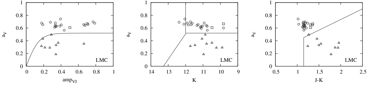
Fig. 6. Similar plots as in Fig. 4 for C-rich, O-rich, and intermediate stars of Cioni et al. (2001), of respective spectral types C (triangles), M (circles), and S (squares).
