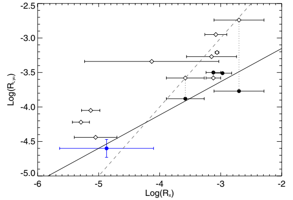
Fig. 8. Normalized Ly \alpha flux R_{\text{Ly}\alpha} = f_{\text{Ly}\alpha}/f_{\text{bol}} as a function of normalized X-ray flux R_X = f_X/f_{\text{bol}} for all the IUE ( \diamond ) and HST ( \bullet ) Ly \alpha flux measurements of M dwarfs in the literature. Our measurement for GJ 436 data is shown in blue. The dotted lines link HST and IUE measurements for objects that have been measured with both instruments. The plain line shows the best-fit linear regression to HST measurements, \log(R_{\text{Ly}\alpha}) \approx 0.5 \log(R_X) - 2.2 . The grey dashed line indicates the \log R_{\text{Ly}\alpha} = \log R_X relation. The horizontal error bars in the X-ray flux are the dispersions reported in Table 2.
