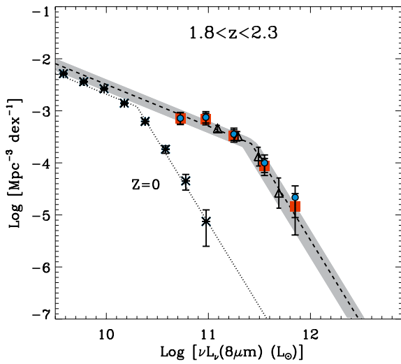
Fig. 2. Rest-frame 8 \mu\text{m} LF estimated at z \sim 2 using the 1/V_{\text{max}} method. Light blue circles and red squares represent the rest-frame 8 \mu\text{m} LF derived from our 24 \mu\text{m} sample with and without X-ray AGNs respectively. Empty triangles represent the rest-frame 8 \mu\text{m} LF derived by Caputi et al. (2007) at z \sim 2 . Asterisks show the local reference taken from Huang et al. (2007) and the dotted line represents the best-fit to these data points with a double power law function with fixed slopes (i.e., \phi \propto L^{-0.8} for L < L_{\text{knee}} and \phi \propto L^{-3.2} for L > L_{\text{knee}} ). The dashed line represents the best fit of the rest-frame 8 \mu\text{m} LF at z \sim 2 assuming that the shape of the rest-frame 8 \mu\text{m} LF remains the same since z \sim 0 . The dark shaded area span all the solutions obtained with the \chi^2 minimization method and compatible, within 1\sigma , with our data points.
