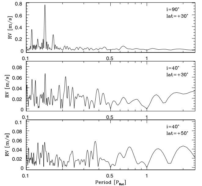
Fig. 10. Lomb-Scargle periodogram of the residuals of the 3 RV variations showed in Fig. 1 after the five-sinusoid fit with fixed periods at the rotational period of the star and its harmonics.
