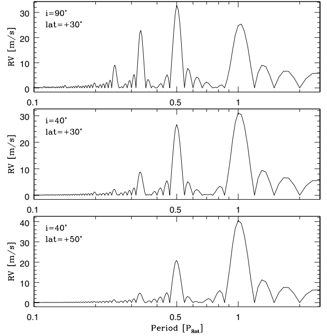
Fig. 2. Lomb-Scargle periodograms of the three RV modulations showed in Fig. 1. The fundamental frequency, P_{\text{rot}} , and its first harmonics are detected.
