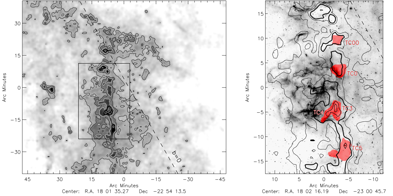
Fig. 6. Left: large scale extinction map of the Trifid region. Right: GLIMPSE 8\ \mu\text{m} image of the Trifid nebula with iso-extinction contours. In both figures contours correspond to A_V = [10, 15, 20, 40, 60] mag, the dashed line follows the Galactic plane. The red shaded regions delineate the S_{1.25} > 10 mJy/11'' beam Trifid Condensations (TC, Cernicharo et al. 1998 ) studied in Sect. 4.3 at 1 arcmin resolution.
