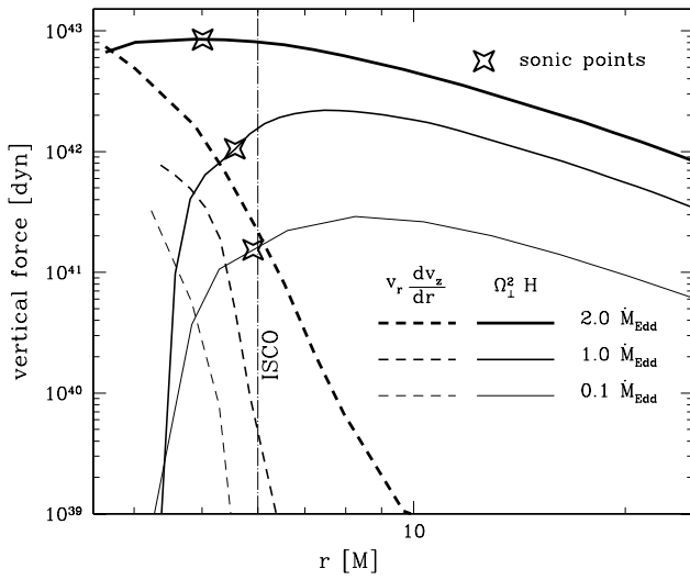
Fig. 12. Comparison of the dynamical ( v_r dv_z/dr \approx Vd(VdH/dr)/dr ) and gravitational ( \Omega_1^2 H ) components of the vertical equilibrium equation at the photosphere. The stars denote locations of the sonic radii.
