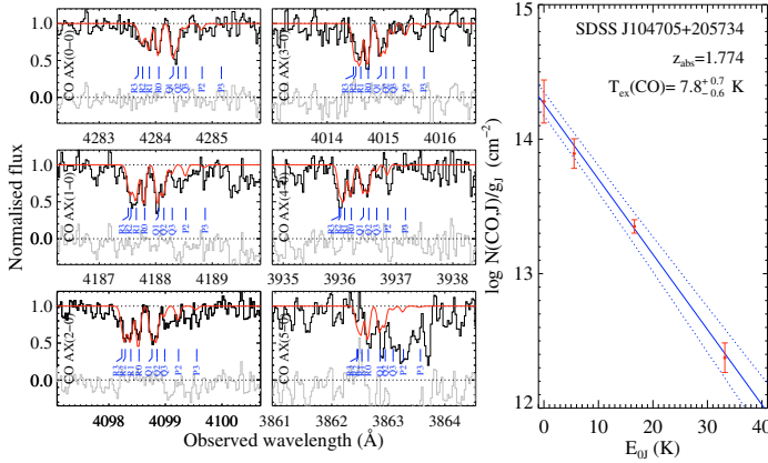
Fig. 1. Left: A^1\Pi(v') \leftarrow X^1\Sigma^+(v = 0) electronic bands of CO detected at z_{\text{abs}} = 1.774 towards the quasar SDSS J104705+205734. The modelled profile is over-plotted in red with the fitting residuals shown in grey. Short vertical lines indicate the branch ("R", "P" or "Q") and the rotational level of the transition ( J = 0-3 ). Right: the corresponding excitation diagram of CO gives the column density of the rotational levels J weighted by their quantum degeneracy ( g_J ) versus the energy of these levels relative to the ground state. The excitation temperature is directly given by -1/(a \ln 10) where a is the slope of the linear fit (solid blue line, with 1\sigma errors represented by the dotted curves).
