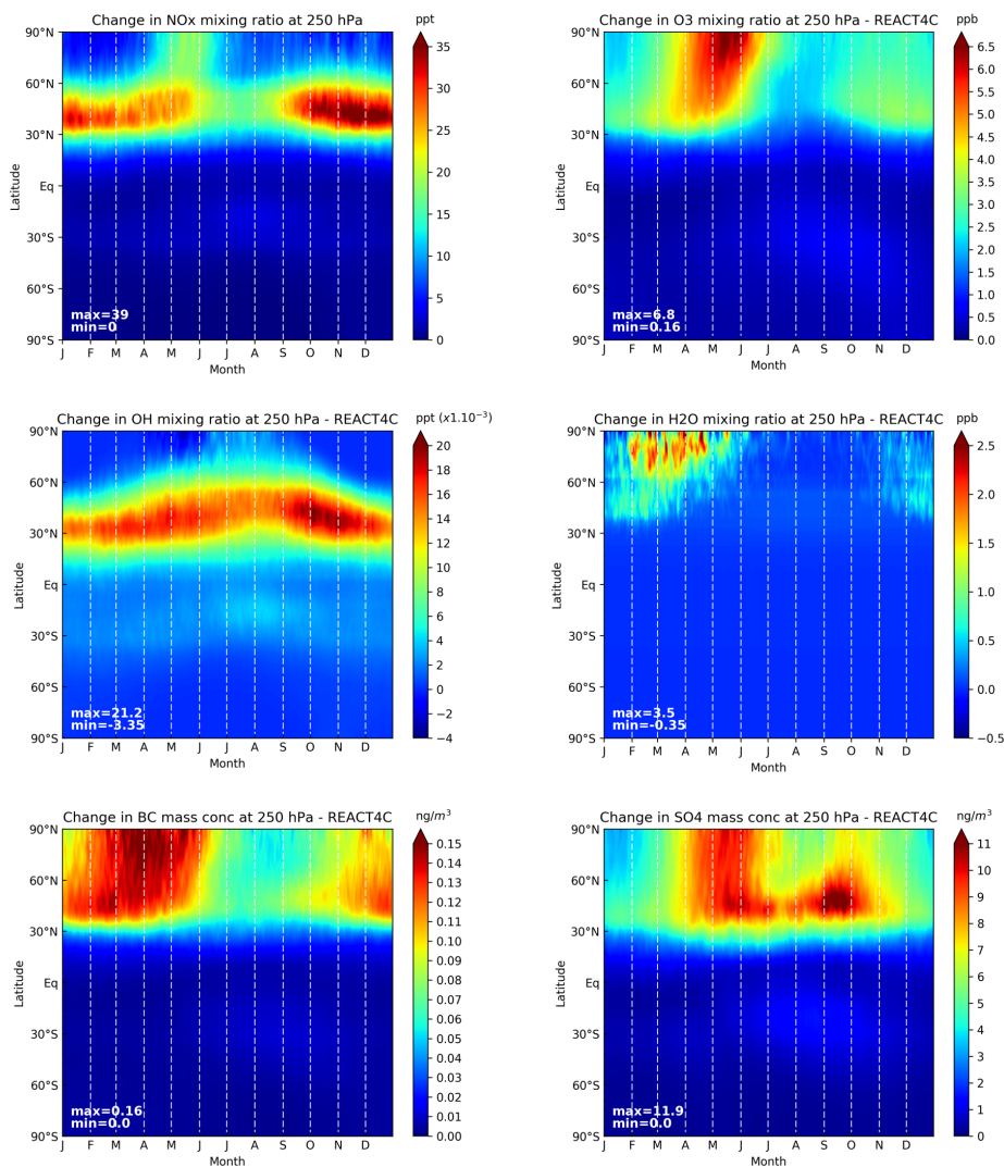
Figure 3. Daily and zonally averaged perturbation due to aircraft emissions at 250 hPa of NO x (pptv), O 3 (ppbv), OH ( 10^{-3} pptv), H 2 O (ppbv), BC (ng/m 3 ) and SO 4 (ng/m 3 ) for the REACT4C_2006 inventory.
