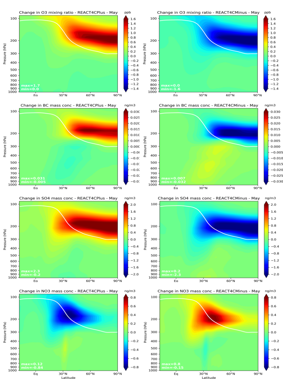
Figure 8. Zonal mean difference for the months of May for O_3 (ppbv), BC ( ng/m^3 ), SO_4 ( ng/m^3 ) and NO_3 ( ng/m^3 ) between the REACT4C_PLUS (left) and REACT4C_MINUS (right) simulations and REACT4C_2004 as the reference. The solid line represents the tropopause pressure.
