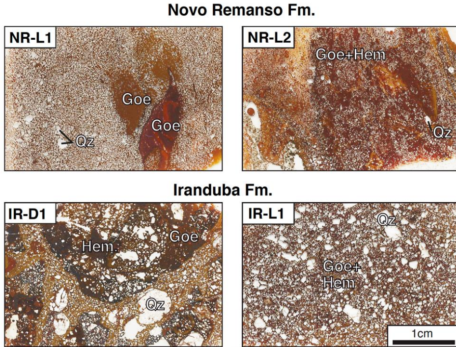
Fig. 4. Optical micro-photographs of thin sections of the NR-L1, NR-L2, IR-D1 and IR-L1 samples. Goethite (Goe), hematite (Hem), and quartz (Qz) occur in all samples but with different proportions. Goethite and hematite are differentiated by colors. Deep red is characteristic of hematite, orange of goethite, and yellow/orange of Al-goethite.
