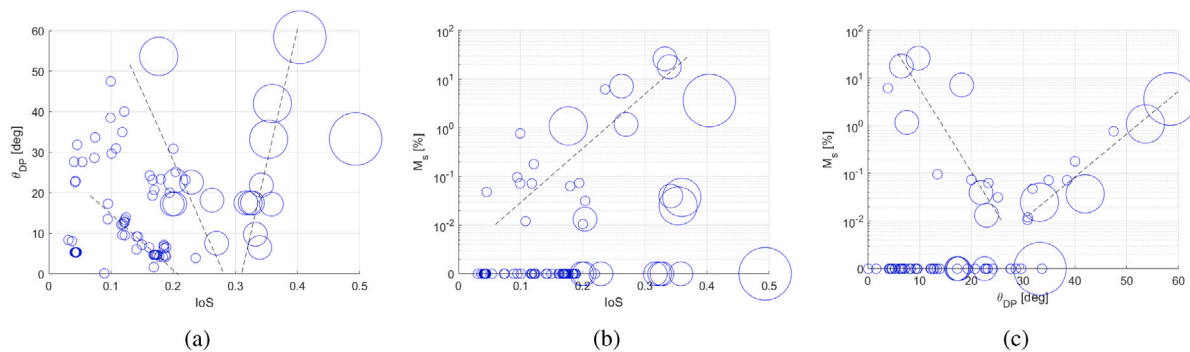
Fig. 4. Aggregated simulation data as function of the Index of Smoothness (IoS), minimum theoretical angle of friction according to the Drucker–Prager criterion ( \theta_{DP} ), percentage of mass shed (if any, M_s ), and percentage of inner rigid volume (size of marker, with smaller circles representing fully fragmented aggregates). Data and major trends are shown for all simulations in the (a) \text{IoS}-\theta_{DP} , (b) \text{IoS}-M_s and (c) \theta_{DP}-M_s planes. Logarithmic y-axes in (b) and (c) are adjusted to show cases without any mass shedding (with M_s = 0 ).
