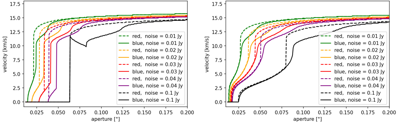
Fig. D.1. Change in the ^{12}\text{CO } v=0 \text{ } J=2-1 velocity measure as a function of the aperture size. The velocity measures are extracted for a range of aperture sizes and noise levels following the same procedure as outlined in Step 2 in Sect. 5.2. The left panel is constructed for a velocity profile with \beta=1 and the right panel for \beta=5 . Velocity measures extracted from the red (blue) wing are indicated with ‘red’ (‘blue’) in the legend in the panels.
