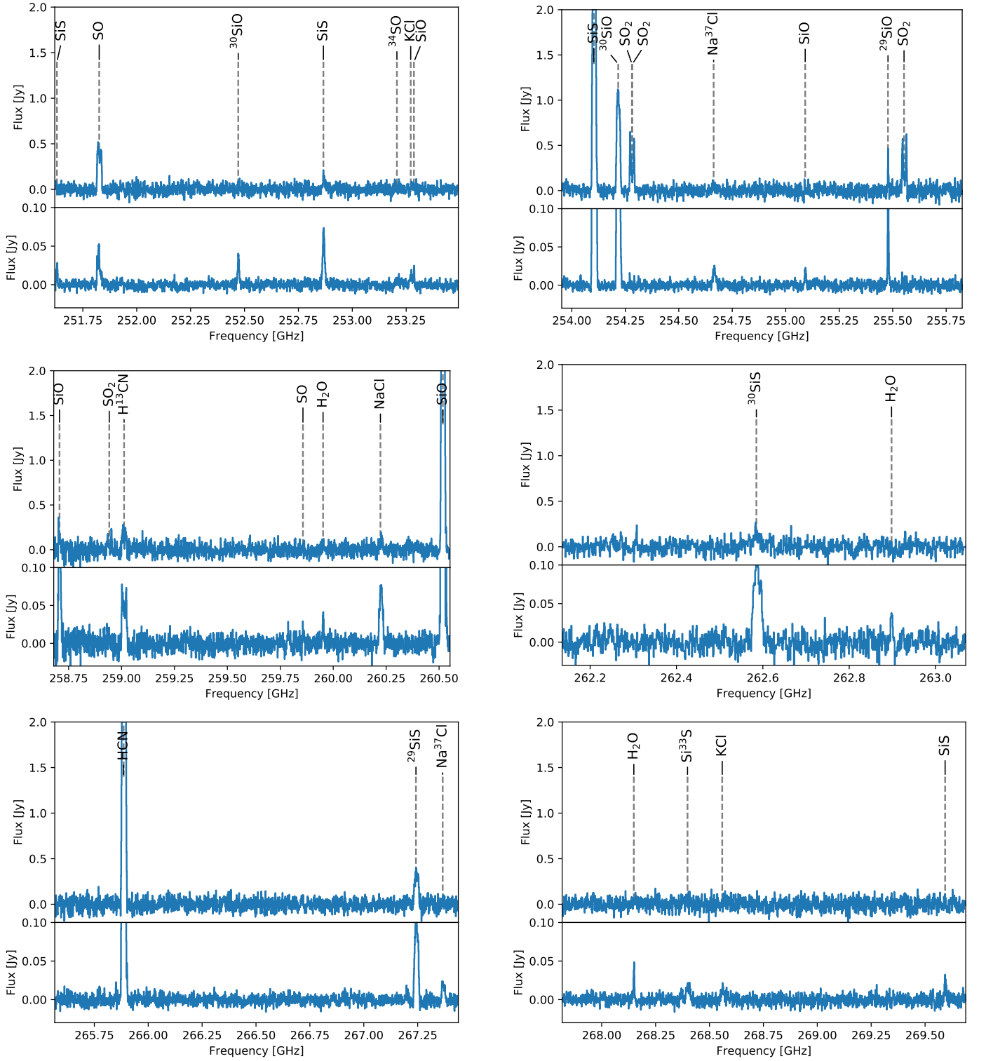
Fig. B.3. ALMA spectra of IRC -10529. Caption; see Fig. 7. Data are displayed for cubes 10 to 15.
