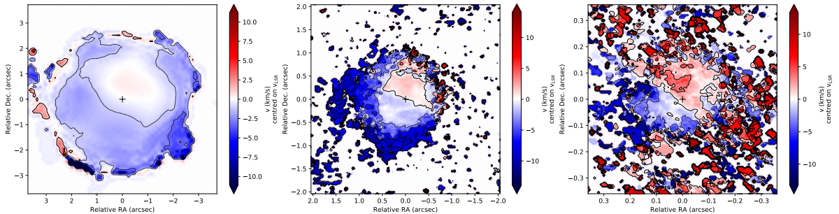
Fig. 6. SiO moment1-maps of IRC -10529. Low ( left panel ), medium ( middle panel ), and high ( right panel ) spatial resolution moment1-map of SiO v = 0 J = 5 - 4 . The black cross indicates the position of the AGB star. The distinct spatial difference between red and blue-shifted velocity components indicates signs of rotation or bipolarity in the inner \sim 0''.5 region of IRC -10529.
