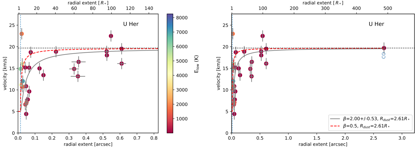
Fig. C.7. Wind kinematics for U Her. See Fig. 11 caption.
