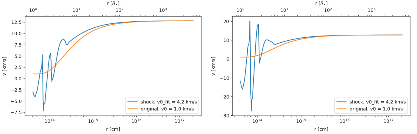
Fig. D.3. Wind velocity profile mimicking pulsation-induced shocks just above the stellar atmosphere. The orange curve shows a beta velocity wind profile for \beta = 5 and v_0 = 1 \text{ km s}^{-1} . The blue curve in the left panel is constructed by: (i) using the shock velocity modelled by Bladh et al. (2019) , see their Fig. 1) up to \sim 10 R_\star followed by; (ii) a beta velocity profile that is fitted through the velocity points beyond \sim 8 R_\star , with \beta = 5 and the fit parameter v_0 which produces a smooth transition from the pulsation-dominated region towards the freely expanding wind region. In the right panel , the blue curve is constructed in a similar way as in the left panel, but this time the shock velocities modelled by Bladh et al. (2019) are multiplied by a factor of 3.
