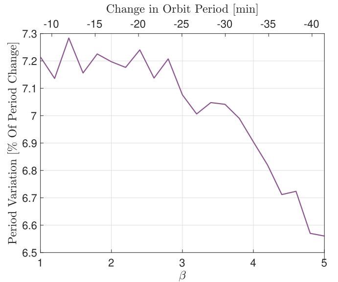
Figure 7. Variation in orbit period as a percent of the change in orbit period for varying values of \beta . The curve is also plotted against the actual change in orbit period.
