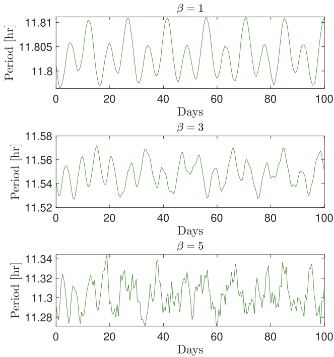
Figure 16. Time history of the orbit period for \beta = 1, 3 , and 5 from the full 3D GUBAS simulations. At \beta = 5 the two-mode structure breaks down and the orbit period variations become irregular. This corresponds to out-of-plane rotation in the barrel instability.
