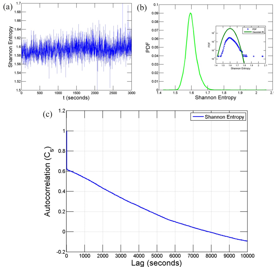
Figure 5. The first 3000 samples of the time series of Shannon entropy in (a), PDF of Shannon entropy along with a Gaussian fit in semi-log plot (inset) in (b) and the autocorrelation of Shannon entropy in (c).
