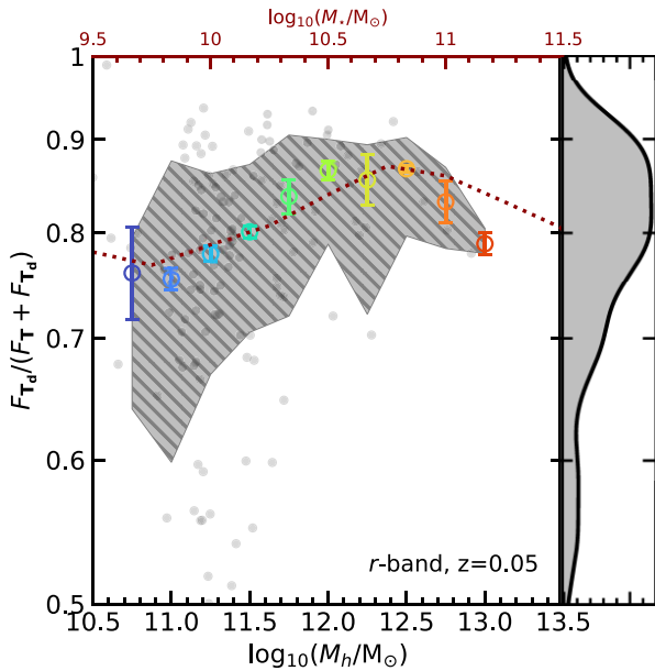
Figure 9. Scatter plot showing the fraction of tidal flux that is found in dense ( \rho_* > 500 M_\odot \text{kpc}^{-3} ) tidal features ( F_{\text{Tidal}}/(F_{\text{Tidal}} + F_{\text{T}}) ) versus the total flux in all tidal features) as a function of halo mass. Coloured error bars show the median value in overlapping mass bins with its 1\sigma uncertainty determined from 100 000 bootstraps. The dotted red line indicates the same median trend with stellar mass (errors are similar). The hatched and shaded grey region indicates the 1\sigma scatter in the grey points. The histogram on the y-axis shows the distribution of the dense f_{\text{tidal}} marginalized over mass. The fraction of flux in dense tidal features appears to increase by a small amount with halo mass (with large scatter), but there is some indication that it begins to fall again around L^* .
