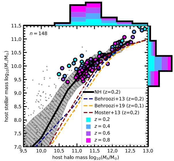
Figure 1. Scatter plot and stacked histograms showing the distribution of host galaxy halo masses and stellar masses selected at z = 0.2 along with their progenitors at z = 0.4, 0.6 , and 0.8 . There are a total of 148 objects (37 unique objects at four different snapshots). Objects in our sample are indicated by coloured points while all other objects are indicated by smaller grey points. The thick black line and shaded region indicate the median halo mass–stellar mass relation and its 1\sigma scatter. Also indicated by coloured dashed lines show relations from the literature (Behroozi et al. 2013, 2019; Moster et al. 2013).
