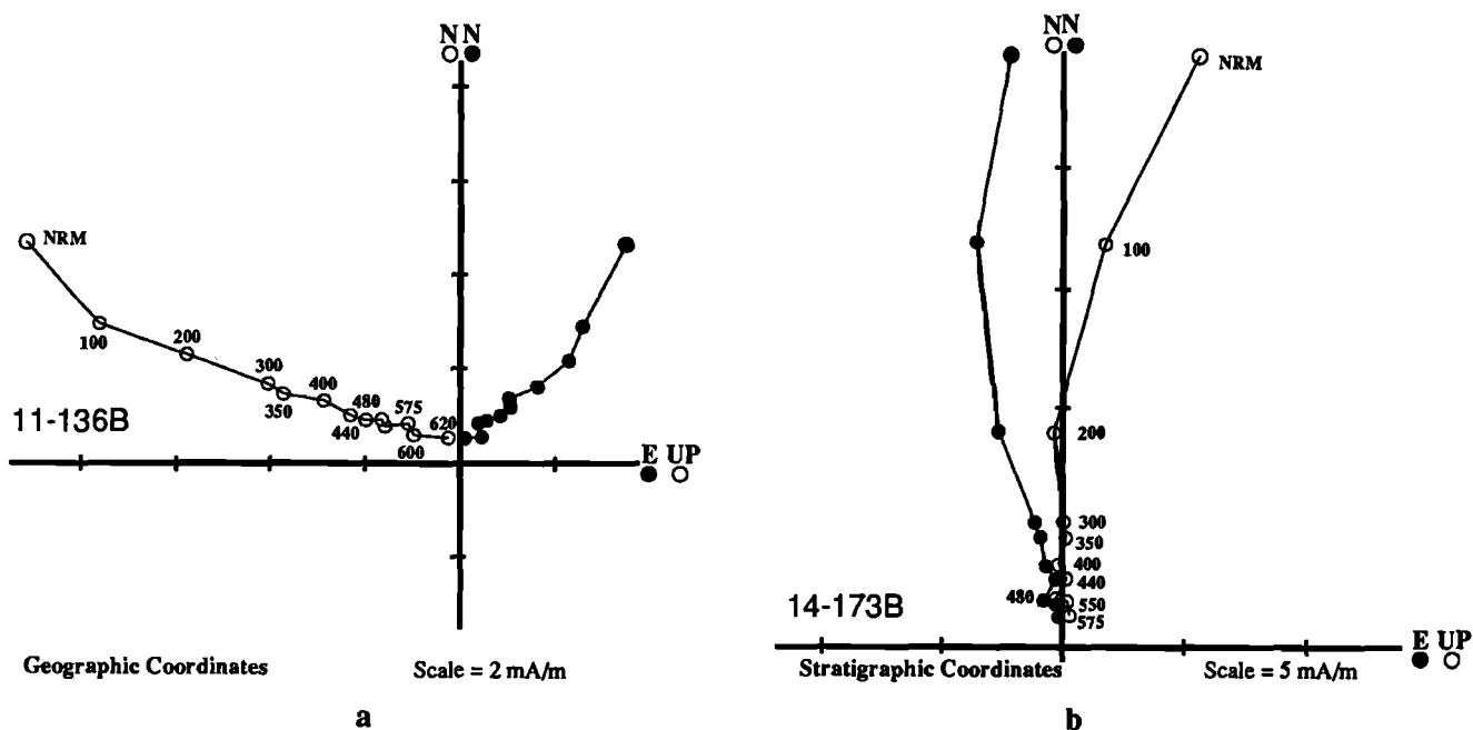
Fig. 5. Orthogonal vector projection of representative thermal demagnetizations from middle Jurassic ( J_{2t} ) samples demonstrating (1) different unblocking temperatures for different sites; (2) steeper directions than present Earth field (PEF) in (a) geographic coordinates and (b) horizontal directions in stratigraphic coordinates. Solid symbols are in horizontal plane, and open symbols in NS vertical plane. Numbers adjacent to data points indicate temperatures (degrees Celsius).
