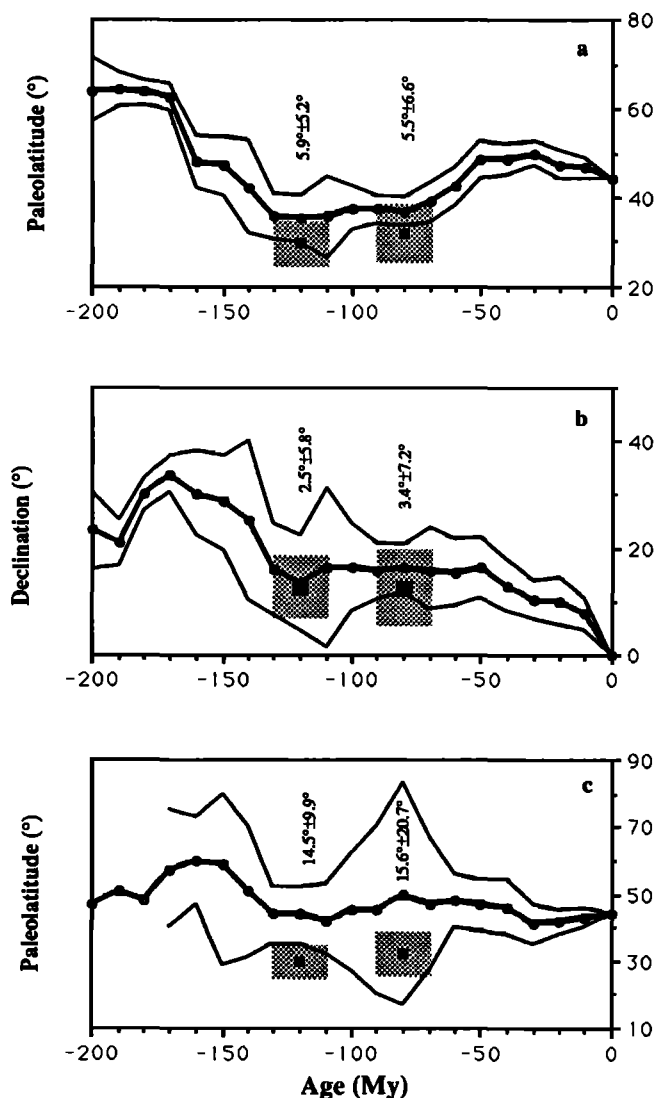
Fig. 14. (a,b) Predicted paleolatitude and paleodeclination of sampling area calculated from Eurasian APWP of Besse and Courtillot [1991]. (c) Predicted paleolatitude from Irving and Irving [1982] APWP. Squares are results from this study for Ju-KI and Ku-II intervals including error bars on ages and mean directions (stippled areas). Differences between results from this study and reference curves are given.
