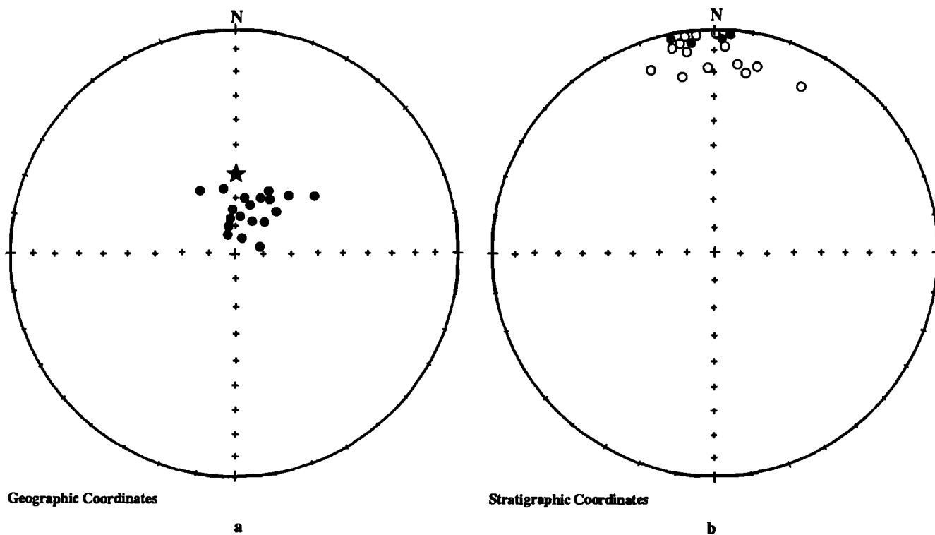
Fig. 6. Equal-area projection of high temperature component (HTC) directions of all middle Jurassic ( J_{2t} ) specimens (a) before and (b) after bedding correction. Note that most directions are steeper than present Earth field (PEF, shown by a star) in geographic coordinates and very shallow in stratigraphic coordinates. Closed (open) symbols are for directions in lower (upper) hemisphere.
