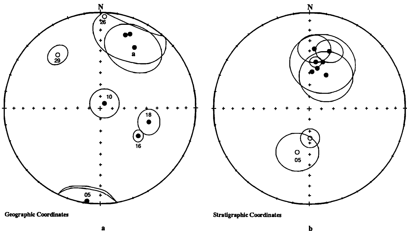
Fig. 12. Equal-area projection of HTC site mean directions from upper Cretaceous-lower Tertiary ( K_{2d} - E_{1-2z} ) sites, (a) before and (b) after bedding correction, with circles of 95% confidence demonstrating positive fold test. Symbols and conventions as in Figure 6.
