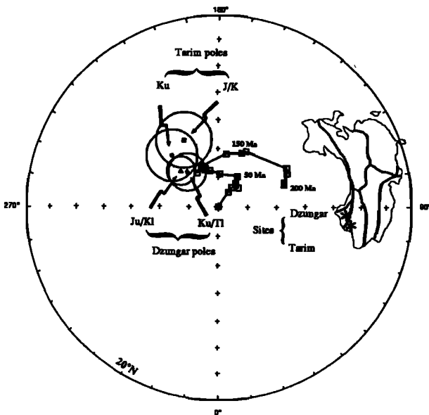
Fig. 13. Apparent polar wander path of Eurasia after Besse and Courtillot [1991], marked with open squares connected by a line (time interval between successive poles is 10 Ma). Other poles are solid square = J/K from Tarim [Li et al., 1988a], solid circle = Ku from Tarim [Li et al., 1988a], triangle = Ju/KI from Dzungar Basin (this study), diamond = Ku/II from Dzungar Basin (this study) and asterisks = Dzungar and Tarim Basin sampling areas.
