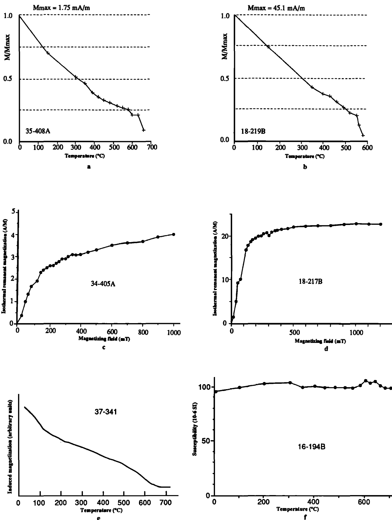
Fig. 10. Results of magnetic study for upper Cretaceous-lower Tertiary ( K_{2d} - E_{1-2z} ) samples. Normalized demagnetization intensity curves presenting clear unblocking temperatures at about (a) 650° and (b) 550°C ; IRM acquisition curves for two types of samples, with (c) high coercivity minerals (goethite and hematite) and (d) a low coercivity mineral (magnetite); (e) thermomagnetic curve in air, demonstrating the existence of goethite (about 100°C), hematite (about 650°C) and a fraction of magnetite (580°C), the applied magnetic field is about 0.6T; (f) susceptibility curve showing stable susceptibility during thermal demagnetization.
