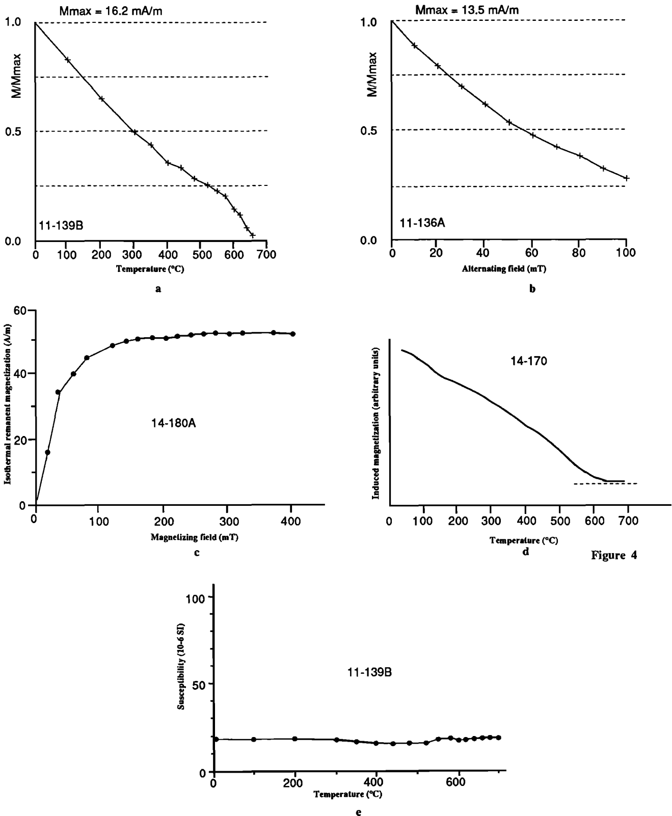
Fig. 4. Results of magnetic study for middle Jurassic ( J_{2t} ) samples. (a, b) Normalized NRM intensity curves showing an unblocking temperature of about 650 ^{\circ}C during thermal demagnetization in Figure 4a, and a rather high coercivity during demagnetization in Figure 4b. M_{max} is the maximum magnetization measured during demagnetization. (c) Acquisition of IRM indicating predominant magnetite for site 14. (d) Thermomagnetic curve in air showing a decrease of magnetic intensity at about 580 ^{\circ}C , also indicative of magnetite for the same site. The applied magnetic field is about 0.5 T. (e) Susceptibility curve demonstrating absence of magnetic mineral change during thermal demagnetization.
