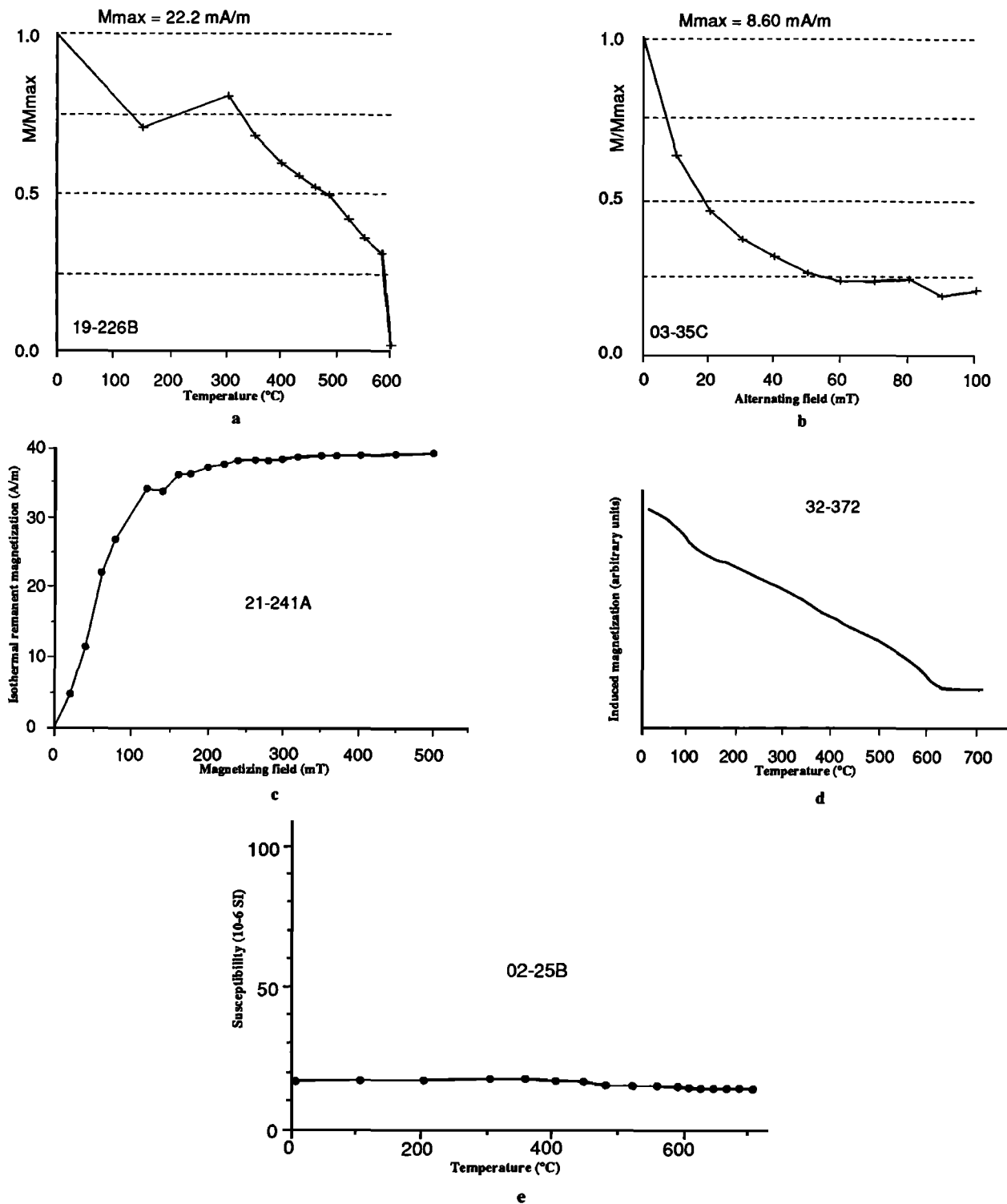
Fig. 7. Results of magnetic study for upper Jurassic-lower Cretaceous ( J_{3q} - K_{1t} ) samples. (a, b) Normalized demagnetization intensity curves (as in figures 4a and 4b, but with unblocking temperature at about 580°C and lower coercivity); (c) Acquisition of IRM showing that prominent magnetic carrier is magnetite. (d) Thermomagnetic curve in air. Note that Curie points of goethite and magnetite are rather clearly discerned at about 100° and 580°C, together with some hematite with Curie point above 600°C. The applied magnetic field is about 0.6T. (e) Susceptibility curve for a representative specimen showing the lack of magnetic mineral change during thermal demagnetization.
