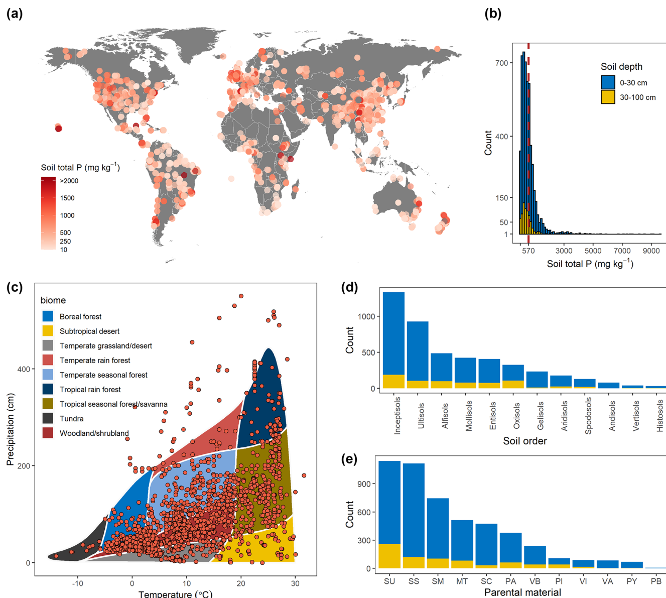
Figure 1. The distribution of our site-level training data. The database contains 5275 observations ( a , b ) covering all major terrestrial biomes ( c ), 12 soil orders ( d ), and 12 parent materials ( e ). The dashed red line in panel ( b ) indicates the arithmetic mean of the soil total P concentration ( 570 \text{ mg kg}^{-1} ). The abbreviations in panel ( e ) represent the following: SU, unconsolidated sediments; SS, siliciclastic sedimentary; SM, mixed sedimentary; MT, metamorphics; SC, carbonate sedimentary; PA, acid plutonic; VB, basic volcanic; PI, intermediate plutonic; VI, intermediate volcanic; VA, acid volcanic; PY, pyroclastics; PB, basic plutonic.
