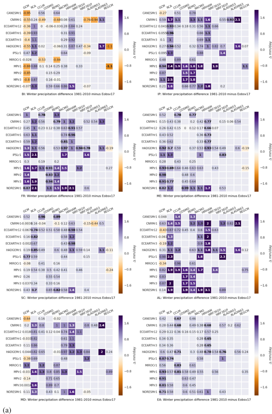
Figure 5a. Same as Figure 2 for precipitation biases as compared to E-OBS. (a) DJF and (b) JJA.
