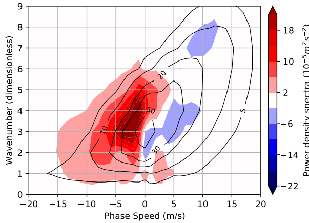
FIG. 4. Latitudinal average (35°–65°N) of the Hayashi spectra of meridional wind at 500 hPa in the model. Contours indicate the ctrl run (contours between 5 and 100 × 10 −5 m 2 s −2 ). Colors indicate the difference between the AA and ctrl runs.
