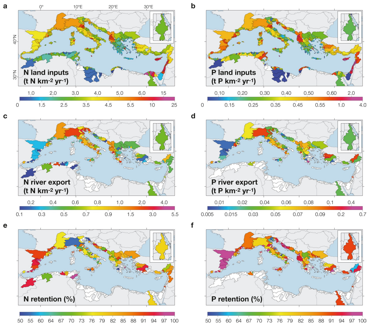
Figure 2. N and P budgets for the 2000–2009 period. (a and b) Nitrogen and phosphorus land inputs per basin (land inputs = fertilizers + manure + \text{N}_2 -fixation + atmospheric deposition + sewage – crop uptake), (c and d) riverine export to coastal seas, and (e and f) the corresponding retention on land (land inputs – river export). Data are spatialized per square km so that basins can be directly compared.
