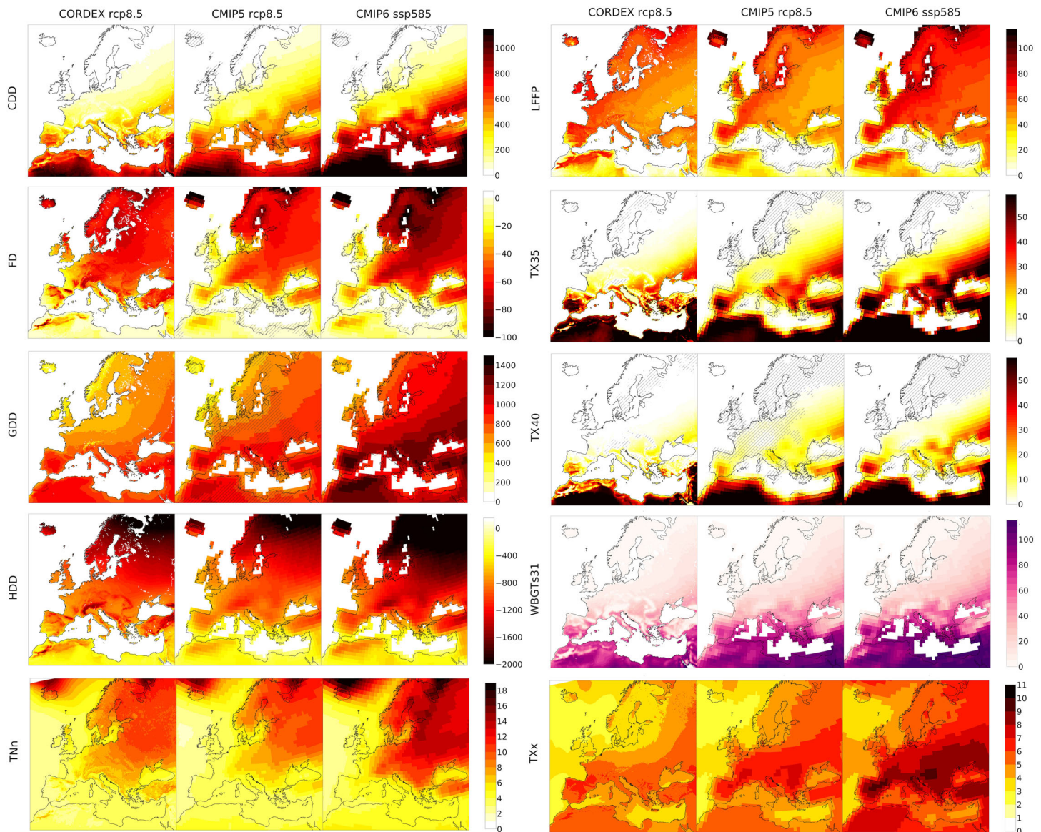
Figure 6. Changes of the following indices: Cooling degree days >22^{\circ}\text{C} change (CDD, units: degree days derived over the whole year), frost days (FD, units: number of days per year), growing degree days >5^{\circ}\text{C} (GDD, units: degree days), heating degree days (HDD, units: degree days), length of frost-free period change (LFFP, units: days), number of days per year with maximum temperature over 35^{\circ}\text{C} and 40^{\circ}\text{C} (TX30 and TX40, units: days per year), and number of yearly events with wet bulb globe temperature greater than 31^{\circ}\text{C} (WBGTS31, units: number of events per year). Results are shown for EUROuro-CORDEX (55 simulations), CMIP5 (12 simulations), and CMIP6 (12 simulations) for 2071–2100 (Far future) relative to 1981–2010. Dashed lines cover areas where changes are not significant at the 95% confidence level (Student's t test).
