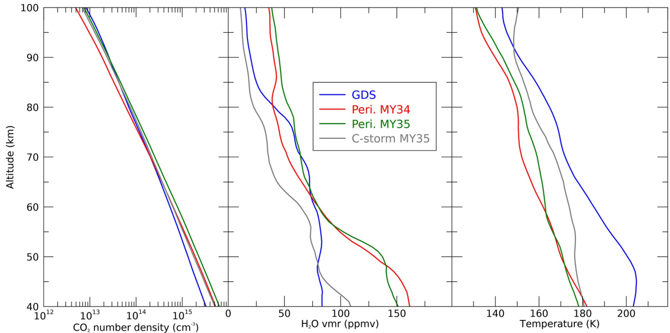
Figure 2. CO 2 number density, H 2 O relative abundance and temperature derived from Atmospheric Chemistry Suite (ACS) data by Belyaev et al. (2021) for the four cases investigated in this study: MY34 global dust storm (GDS) and Perihelion, MY35 Perihelion and C-storm.
