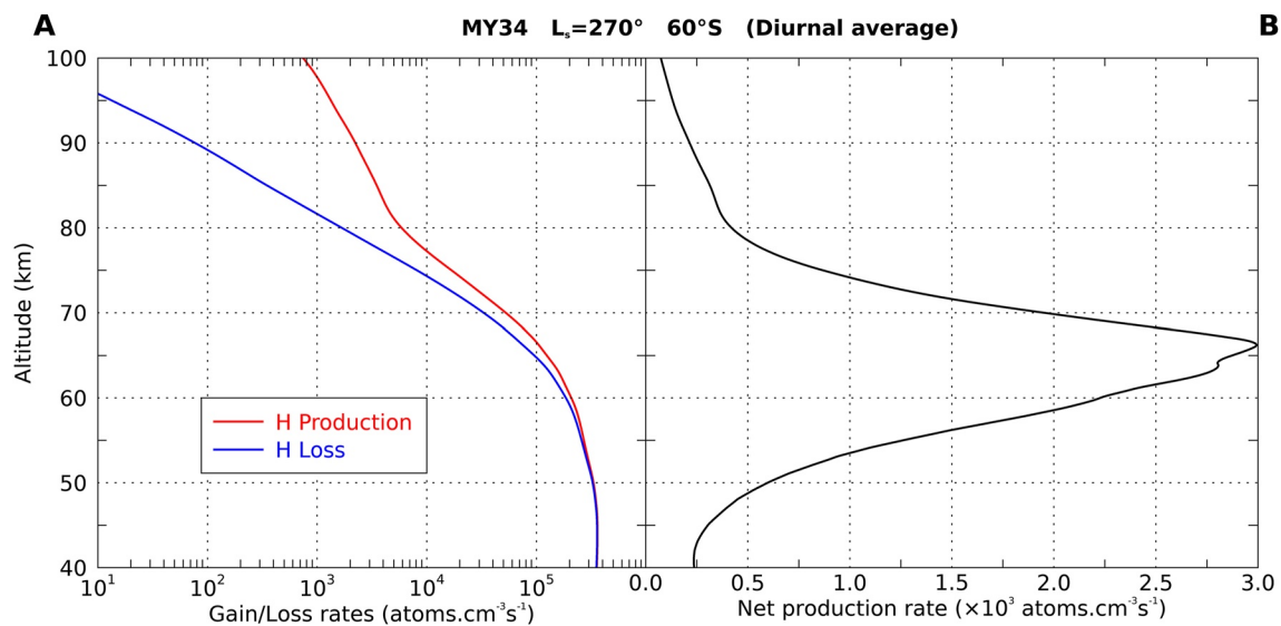
Figure 3. (a) H production and loss rates as predicted by a photochemical model for the MY34 Perihelion case, using pressure, temperature, and water vapor profiles obtained by Atmospheric Chemistry Suite MIR channel. H production is only due to water vapor photolysis. H loss relies on reactions with O 3 , HO 2 , and O 2 . (b) H net budget calculated by subtracting loss from production rates.
