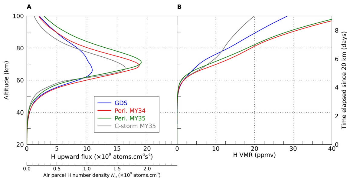
Figure 8. A synthesis of the four configurations explored with the air parcel model: global dust storm, MY34 and MY35 Perihelion, MY35 C-storm. (a) H upward flux and concentration in the parcel during its rise from 20 to 100 km. Panel (b) same as panel (a) except N_H is converted into H volume mixing ratio (parts-per-million in volume).
