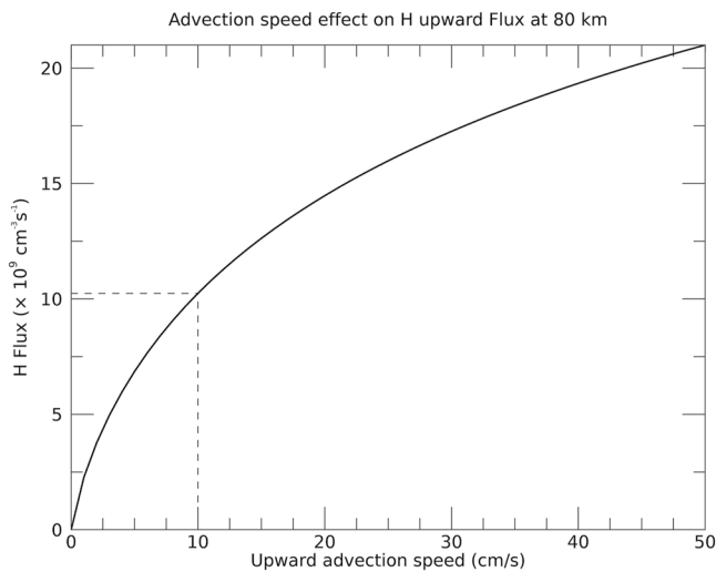
Figure 7. Sensitivity of the simulated H flux at 80 km to upward velocity in the case of the MY34 Perihelion simulation. Our baseline has a velocity of 10 cm/s, yet even a twofold increase or decrease in velocity only impacts H flux by ~40%.
