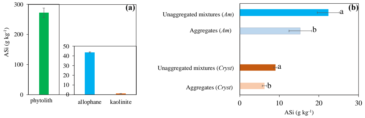
Figure 3. Estimated contents of amorphous Si (ASi), as quantified following DeMaster (1981) from \text{Na}_2\text{CO}_3 extractable Si ( \text{Na}_2\text{CO}_3\text{-Si} ) data (Fig. S2 and S3), in phytolith, allophane, kaolinite, mixtures and aggregates of the amorphous ( Am ) and crystalline ( Cryst ) models.
