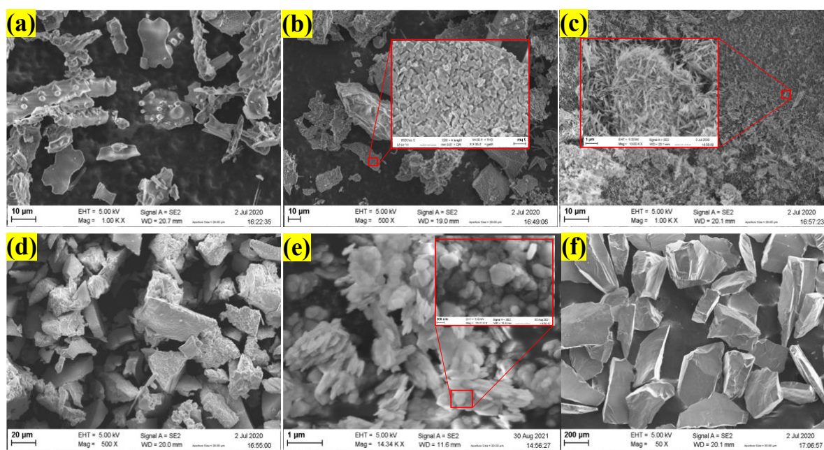
Figure S1. Scanning electron microscope (SEM) images of: (a) rice phytolith, (b) allophane, (c) goethite, (d) ferrihydrite, (e) kaolinite, and (f) quartz.
