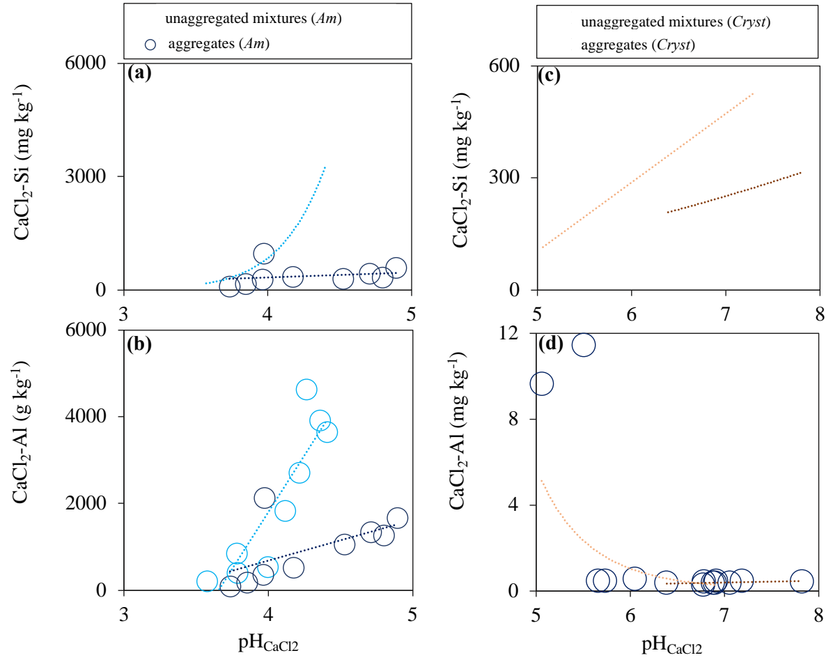
Figure 6. Concentrations of Si and Al in the \text{CaCl}_2 extracts ( \text{CaCl}_2\text{-Si} and \text{CaCl}_2\text{-Al} ) as plotted against pH of respective \text{CaCl}_2 extracts ( \text{pH}_{\text{CaCl}_2} ) in (a-b) the unaggregated mixtures and aggregates of the amorphous ( Am ) model, (c-d) the unaggregated mixtures and aggregates of the crystalline ( Cryst ) model.
