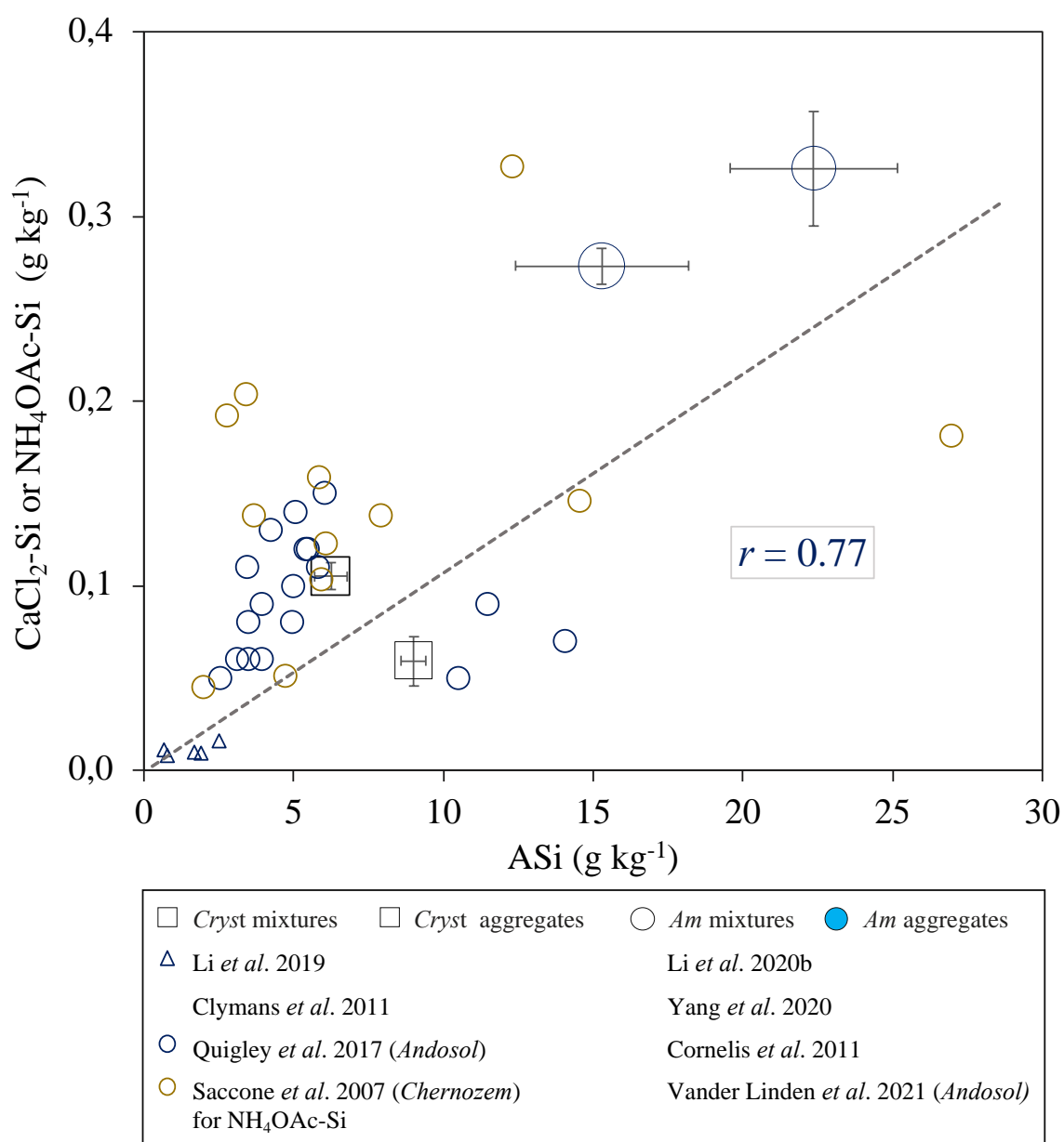
Figure 9. Plot of bioavailable Si content, as assessed by \text{CaCl}_2 0.01 M or \text{NH}_4\text{OAc} 0.5 M, against amorphous Si content (ASi), as assessed by \text{Na}_2\text{CO}_3 (DeMaster, 1981), in soil samples from different soil–plant systems, and in the Am and Cryst mixtures and aggregates of this study. Note: \text{NH}_4\text{OAc-Si} only concerns the Chernozem samples (Saccone et al. , 2007).
