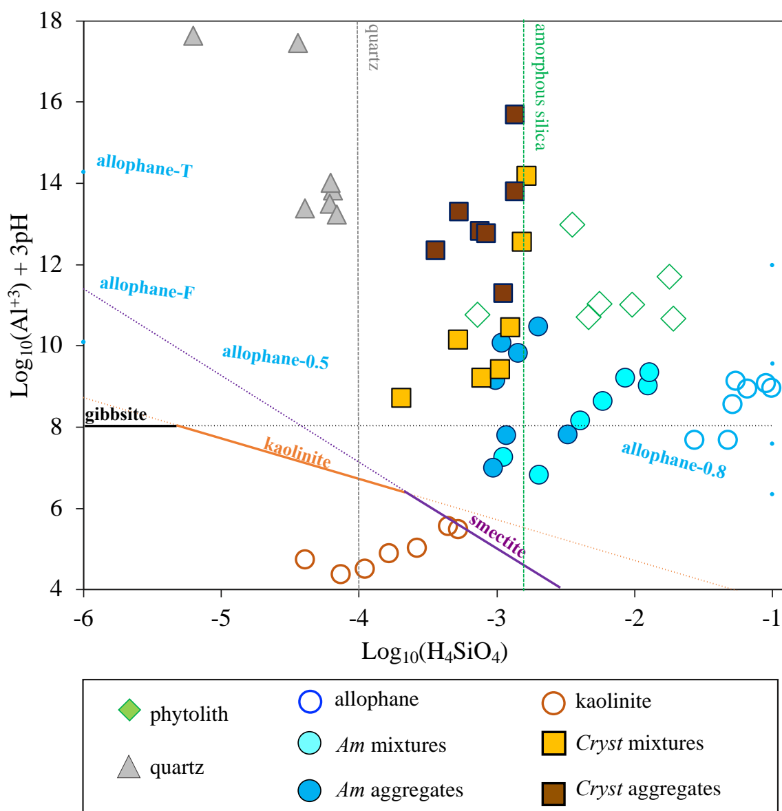
Figure 8. Plot of the logarithmic values of experimental \text{Al}^{3+} , \text{H}^+ and \text{H}_4\text{SiO}_4 concentrations (mol \text{l}^{-1} ) in \text{CaCl}_2 extracts at each kinetic step (this study) in the stability diagram for reference allophane, gibbsite, kaolinite and smectite in the \text{Al}_2\text{O}_3 – \text{SiO}_2 – \text{H}_2\text{O} system. Allophane-T refers to theoretical composition calculated with amorphous silica and amorphous alumina as end-members, and might be regarded as a freshly precipitated amorphous aluminosilicate phase (Dobrzyński, 2006). Allophane-F refers to field data from Pačes (1978). Allophane-0.5 and allophane-0.8 refer to data on synthetic allophanes with Si/Al ratio of 0.5 and 0.8, respectively (Su and Harsh, 1998). Gibbsite, kaolinite and smectite solubility lines refer to Lindsay (1979).
