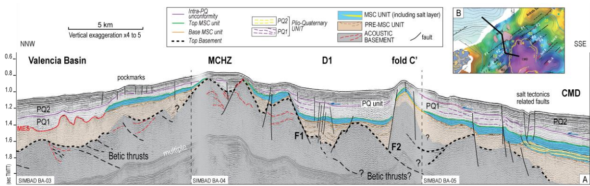
Figure 7. A: Seismic profile across the Mallorca Channel, illustrating the MCHZ (Mallorca Channel Horst Zone) adjoining the MCDZ (Mallorca Channel D epression Zone, here D1 depocenter/mini-basin). Faults clearly offset the MSC unit (in blue) and thicken the PQ unit. Betic orogenic thrusts are observed towards the Valencia Basin and normal faults like F1 could scale at depth into the thrusts, as observed on deep penetration seismic lines. B: Base Pliocene souths map (see Figure 10) showing the location of the seismic profile shown in A.
